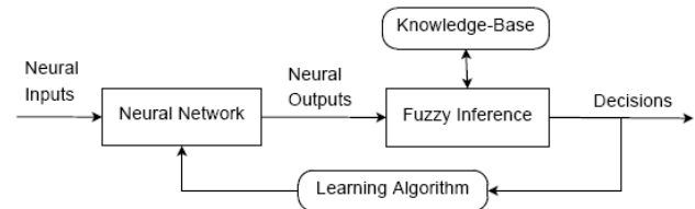
Figure 3. Neuro-fuzzy system [50].
