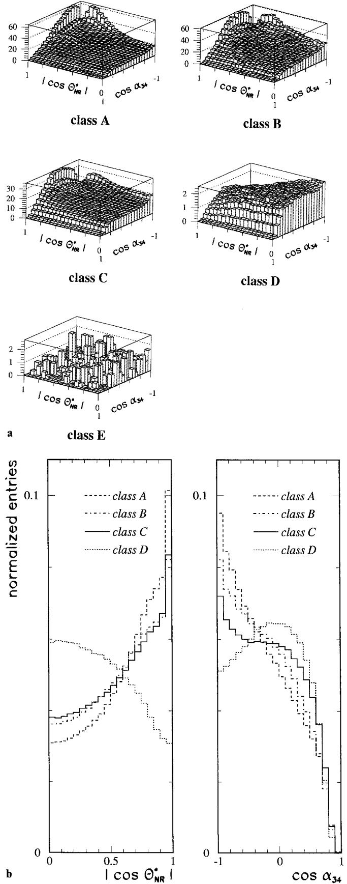
Fig. 6a, b. Distributions of the 4-jet events after cuts from the classes A , B , C , D , E (deduced from large statistics of generated events for QCD and Abelian model). a two-dimensional; b projections on |\cos \theta_{NR}^*| and \cos \alpha_{34} (without class E )
