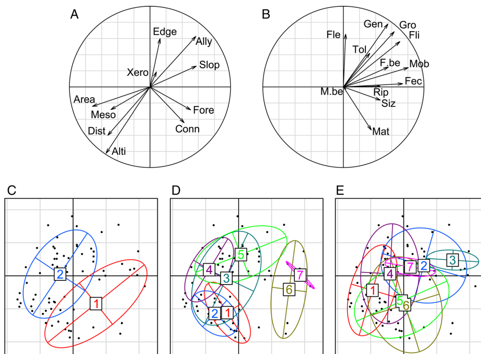
FIG. 3. Results of the RLQ approach. In all panels, axis 1 is horizontal and axis 2 is vertical. Axis 1 expressed 53% of the covariance between the environmental variables and species traits. Axis 2 expressed 30% of this covariance. Panel (A) displays a correlation circle where each arrow gives the Pearson correlations between an environmental variable and the two axes of the RLQ. Environmental variables included abiotic factors (Alti, averaged altitude; Area, log-transformed area; Conn, connectivity; Dist, distance to roads; Edge, edge length; Slop, slope, i.e., difference in altitude) and flora indicators (Ally, Alyssa-Sedion albi habitat; Fore, forest habitats; Meso, Mesobrometum; and Xero, Xerobrometum) see Materials and methods for details. Panel (B) displays a correlation circle where each arrow gives the Pearson (Spearman) correlations between a quantitative (ordinal) trait and the two axes of the RLQ. Panels (C–E) display nominal traits. The attributes of the nominal traits are positioned at the center of the species points that possess them, and an ellipse indicates the dispersion of species points around the center. Scales in all panels are given by a grid with cell side equal to 0.2 in panels (A and B) and to 1.0 in panels (C–E). Codes for all traits as in Fig. 2.
