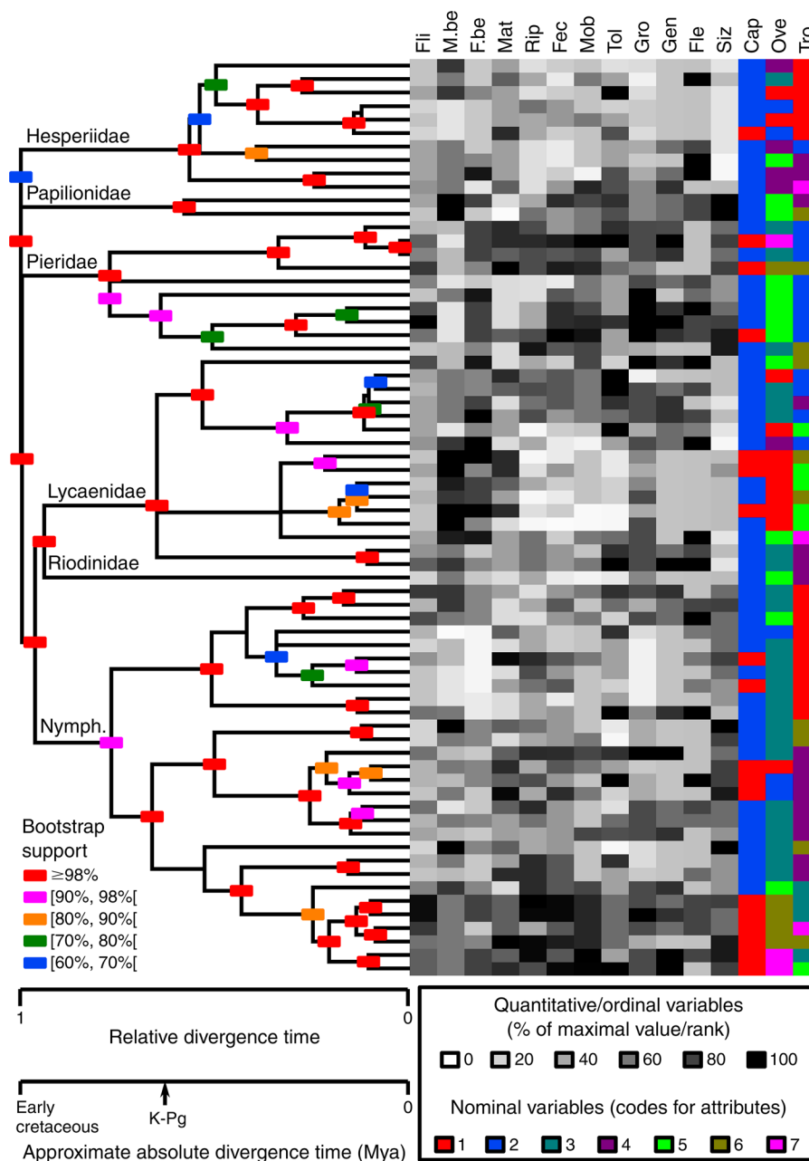
FIG. 2. Molecular phylogenetic tree of the 68-species RAxML maximum likelihood analyses (Stamatakis 2006) and life history traits. Branch lengths on the phylogenetic tree are expressed as relative divergence time as estimated by PATHd8 algorithm (Britton et al. 2007). An indication of the time periods under which speciation events occurred is given at the bottom of the tree (where Cretaceous-Palaeogene is shown as K-Pg, and Mya stands for million years ago; Heikkilä et al. 2012, Wahlberg et al. 2013). Support values were derived from 1000 bootstrap replicates. The divergences of the families are indicated (Nymph. represents Nymphalidae). The life history traits are given in front of the phylogeny with color scales. Quantitative and ordinal traits were divided by their maximum value and rank, respectively, to obtain variables bounded by 0 and 1. Trait codes (top of Fig.) are: Fli, adult flight period; M.be, male behavior; F.be, female oviposition behavior; Mat, female maturation; Rip, ripe egg load; Fec, potential fecundity; Mob, mobility; Tol, tolerance; Gro, larval growth rate; Gen, generation number; Fle, developmental flexibility; Siz, adult size; Cap, capital breeder; Ove, overwintering stage; and Tro, tropic group (larvae) (Appendix C). Codes for the attributes of the nominal variables for the capital breeder are: 1, no egg at the beginning of the female adult stage; and 2, eggs at the beginning of the female adult stage. Codes for the overwintering stage are: 1, eggs; 2, small larvae; 3, mean larvae; 4, large larvae; 5, pupae; 6, adults; 7, in warm countries. Codes for the trophic group are: 1, monocot (Cyperaceae, Poaceae); 2, Brassicaceae, Fabaceae, Tropeolaceae; 3, Urticaceae, Cannabinaceae; 4, other flowering plants; 5, combination of herbs; 6, trees; 7, combination of herbs and trees (see Appendix B for the names of the species in the same order as in the phylogenetic tree and trait table, and see Appendix C for details on traits). Square brackets around the bootstrap support values designate intervals; i.e., they include the lesser value and go up, but do not include, the higher value.
