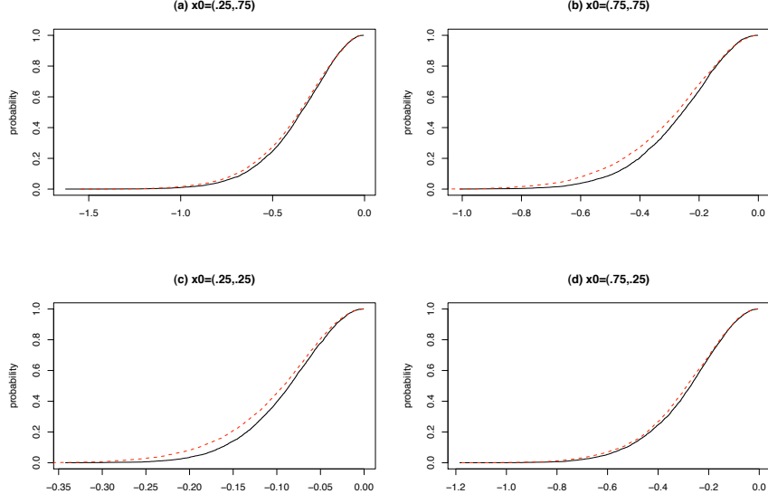
Figure 2: Solid curves are the empirical distribution functions of Z_n(0) and the dotted curves are those of n^{2/(p+1)} \{\hat{g}(\mathbf{x}_0) - g(\mathbf{x}_0)\} in the case where n = 100 and \lambda = 3 .
