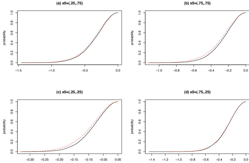
Figure 3: Solid curves are the empirical distribution functions of Z_n(0) and the dotted curves are those of n^{2/(p+1)} \{\hat{g}(\mathbf{x}_0) - g(\mathbf{x}_0)\} in the case where n = 400 and \lambda = 3 .
