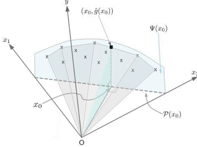
Figure 1: An illustration of \mathcal{P}(\mathbf{x}_0) , \mathbf{P}_i , \hat{\Psi} and \hat{g} in the case of p = 2 and q = 1 . The crosses are the points \mathbf{P}_i , and the gray surface is the roof of the conical-hull estimator \hat{\Psi} .
