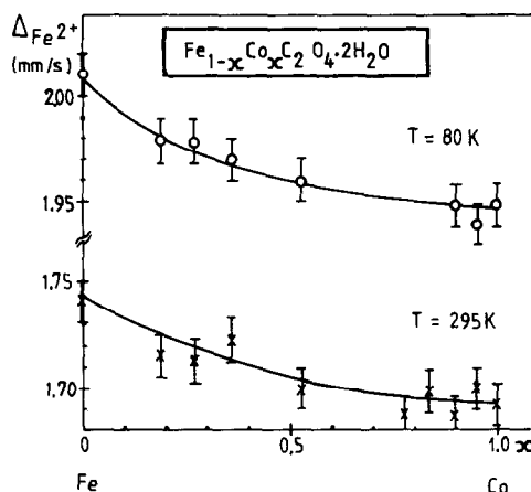
Fig. 4. 57 Fe 2+ quadrupole splittings in Fe 1-x Co x C 2 O 4 ·2H 2 O plotted against Co content in the mixed crystals.
