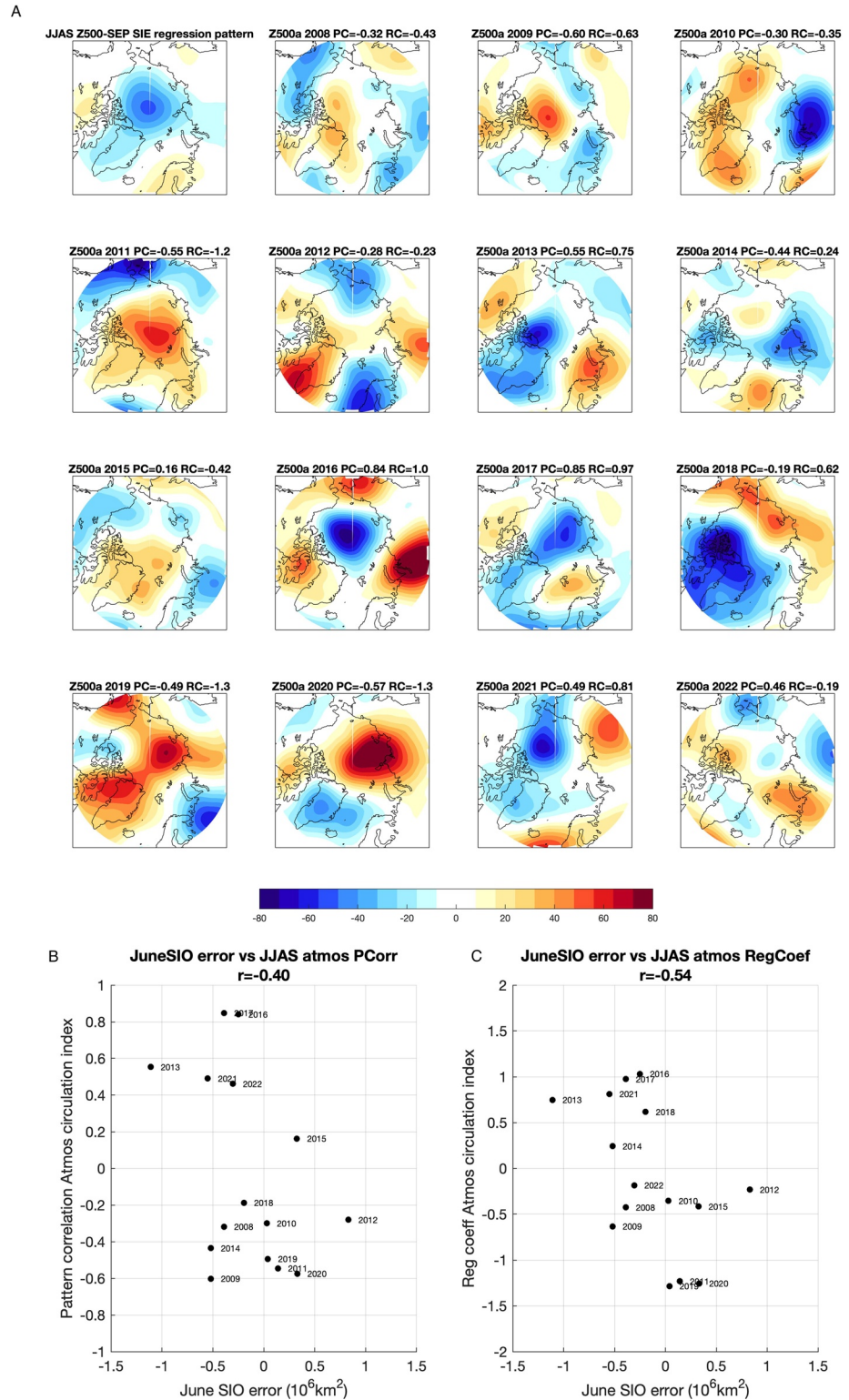
Figure 5. (a) The regression of June through September (JJAS) 500 hPa heights on September sea ice extent over 1979–2022 (in m per 10^6 \text{ km}^2 ), anomalous JJAS 500 hPa heights (in m) over 2008–2022, the titles show the pattern correlation (PC) and regression coefficient (RC) with the regression pattern in the top left panel. Only values north of 60^\circ\text{N} are shown. (b, c) Scatter plots of the June Sea Ice Outlook (SIO) median error ( x -axis) and the JJAS anomalous atmospheric circulation, characterized by pattern correlation (b) and regression coefficient (c).
