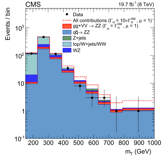
Fig. 4. Distribution of the transverse mass in the 2\ell 2\nu channel. Points represent the data, filled histograms the expected contributions from the backgrounds, and from the gluon fusion (gg) and vector boson fusion (VV) SM processes (including the Higgs-mediated contributions). The dashed line corresponds to the total expected yield for a Higgs boson width and a squared product of the couplings scaled by a factor 10 with respect to their SM values. The bin size varies from 80 to 210 GeV and the last bin includes all entries with transverse masses above 1 TeV.
