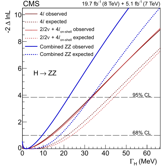
Fig. 5. Scan of the negative log-likelihood, -2\Delta\ln\mathcal{L} , as a function of \Gamma_H for the combined fit of the 4\ell and 2\ell 2\nu channels (blue thick lines), for the 4\ell channel alone in the off-shell and on-shell regions (dark red lines), and for the 2\ell 2\nu channel in the off-shell region and 4\ell channel in the on-shell region (light red lines). The solid lines represent the observed values, the dotted lines the expected values. (For interpretation of the references to color in this figure legend, the reader is referred to the web version of this article.)
