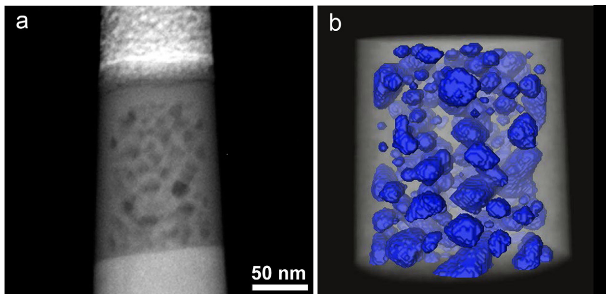
Figure 1. (a) 2D projection image of a needle-shaped pillar of a porous \text{La}_2\text{Zr}_2\text{O}_7 layer. (b) Visualization of the 3D SIRT reconstruction showing the pores in dark blue (after figures 1 and 2 of [7]).
