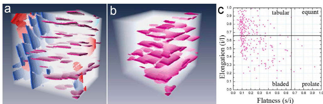
Figure 4. (a) 3D representation of a 5 \times 5 \times 5 \mu\text{m}^3 volume from a stress-free annealed single crystal, showing groups of single variant precipitates formed by autocatalytic nucleation and growth. (b) A single group selected for ease of visualization. (c) The Zingg and Tucker scheme revealing the shape distribution of the measured precipitates.
