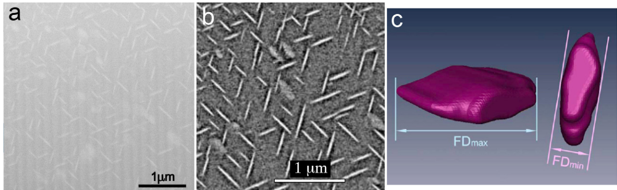
Figure 3. (a) Typical example of an SEM image of \text{Ni}_4\text{Ti}_3 precipitates showing only limited contrast before image treatment. (b) Better delineated precipitates after image processing. (c) Feret or clip diameter definition (min and max).
