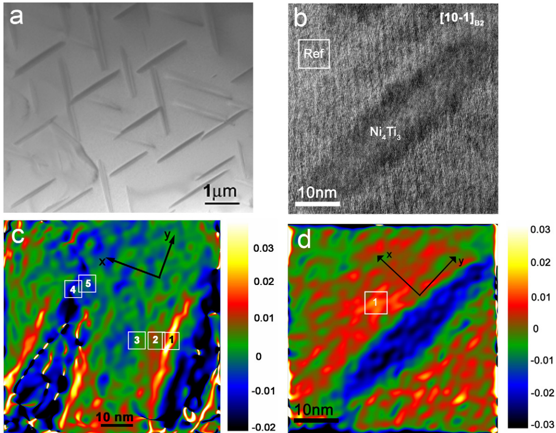
Figure 2. (a) Combination of four orientation variants of \text{Ni}_4\text{Ti}_3 precipitates in B2 austenite, (b) HRTEM [10-1]_{B2} image of a single precipitate (the square labeled as ‘Ref’ represents the undistorted austenite matrix), and (c) and (d) GPA maps showing the \varepsilon_{xx} matrix strain alongside precipitates observed in [1-1 1]_{B2} and [1 0 -1]_{B2} orientations, respectively ((d) shows the same precipitate as (b)).
