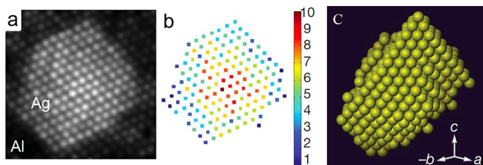
Figure 10. (a) HAADF-STEM image of an Ag particle in an Al matrix viewed along the [10\bar{1}] direction; (b) the estimated number of atoms for each column; and (c) [1\bar{1}0] 3D view of the reconstructed particle based on this and similar data from a \langle 100 \rangle direction.
