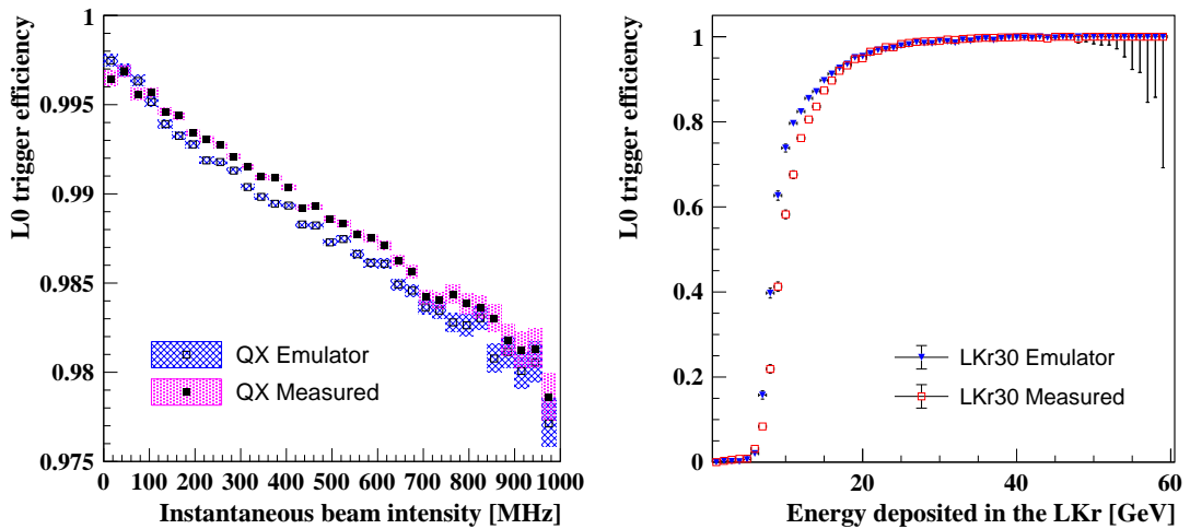
Figure 12: Efficiencies of the L0 trigger conditions QX (left) and LKr30 (right) measured using K^+ \rightarrow \pi^+\pi^+\pi^- events collected via the control trigger line, and simulated using the trigger emulator on the same data. The hatched areas indicate the statistical uncertainties of the measurements.
