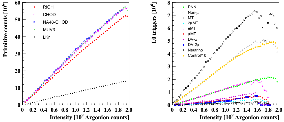
Figure 3: Number of primitives (left) and L0 triggers before downscaling (right) per spill as a function of the average beam intensity.
