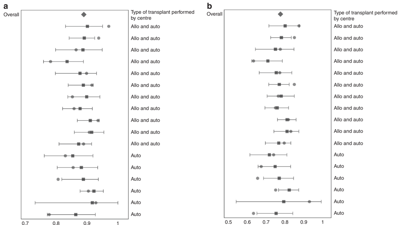
Fig. 1 Forest plot of the survival at 1 year ( a ) and 3 years ( b ) for autologous transplants in Belgium (2007-2013), as predicted by the multivariable model for all centres. Survival at 1 year was adjusted for transplant year, performance status, disease risk index and transplant number. Survival at 3 years was adjusted for transplant year, age, performance status, time between diagnosis and transplant, disease risk index and transplant number. Centres are represented by a blue square that indicates the 1-year (or 3-year) survival for that centre as predicted by the multivariable model (adjusted for case-mix). 95% confidence
