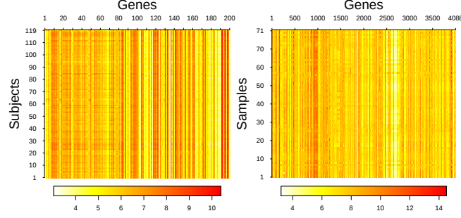
Figure 4: Heatmap of the predictor gene expression levels for the Scheetz et al. (2006) dataset (left panel) and for the Bühlmann et al. (2014) dataset (right panel).
