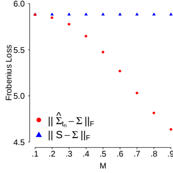
Figure 2: Simulation data. Frobenius loss (smaller is better) of the difference between \hat{\Sigma}_{t_n} and the true \Sigma and between S and \Sigma . Each symbol represents the empirical median of 300 repetitions from the same scenario where only the value M changes.
