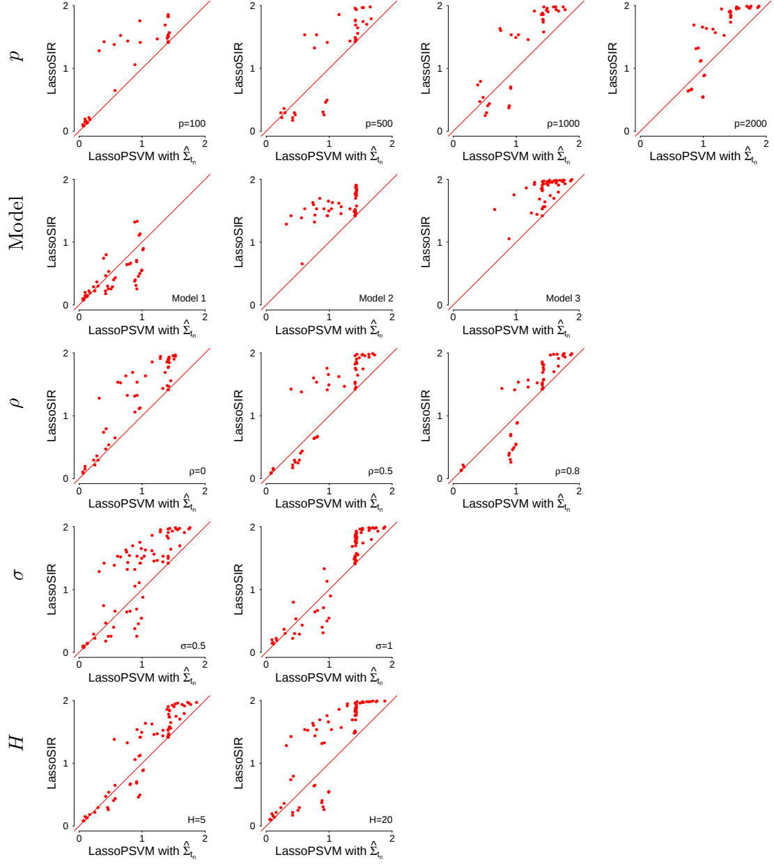
Figure 3: Simulation data. Results of the 144 scenarios split by values of p , model, values of \rho , \sigma and H .
