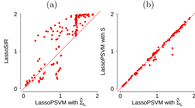
Figure 1: Simulation data. Frobenius loss (smaller is better) for LassoPSVM with \hat{\Sigma}_{t_n} (x-axis) and LassoSIR (y-axis) in panel (a) and LassoPSVM with \mathbf{S} (y-axis) in panel (b). Values above the main diagonal show a better performance of LassoPSVM with \hat{\Sigma}_{t_n} . Each symbol represents the empirical median of 300 repetitions from a scenario and the results of 144 different scenarios are plotted.
