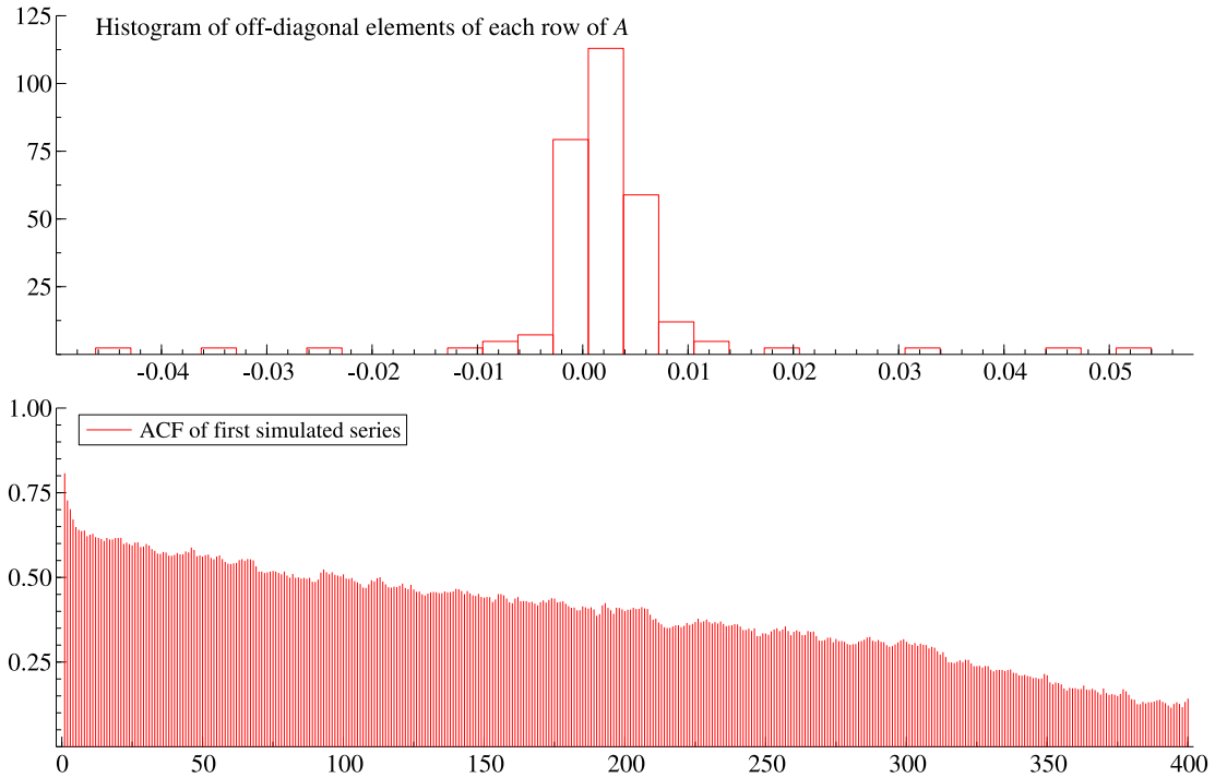
Fig. 1. Top: Histogram of the values of the 249 off-diagonal elements of each row of the matrix \mathbf{A}_n of the VAR(1) corresponding to DGP 2 . Bottom: Autocorrelogram of the first simulated series.
