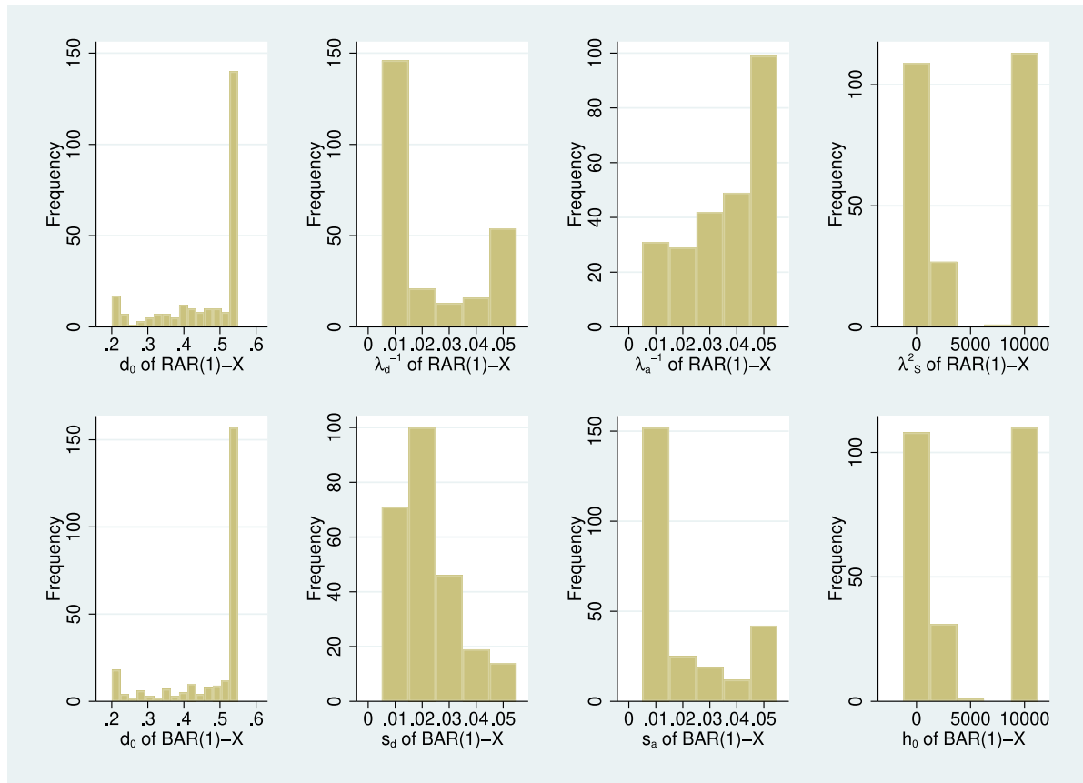
Fig. 5. Histogram of the four tuning parameters estimated by cross validation on the first sample of 1000 observations for the application.
