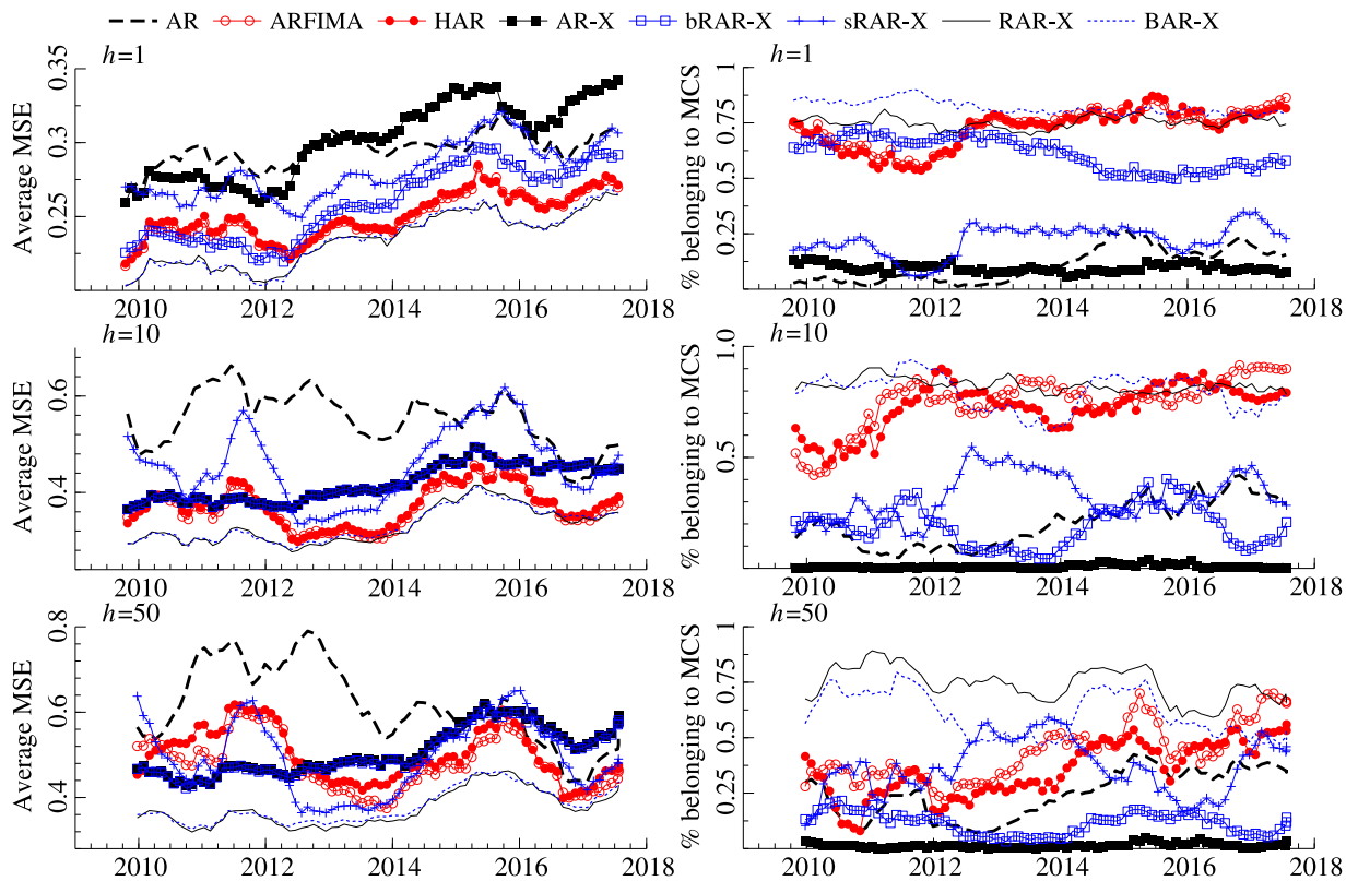
Fig. 3. Left panels: Average (over the 250 series) MSE loss computed on rolling windows of 250 forecasts. Right panels: Frequencies (over the 250 series) at which each model belongs to the MCS (at the 95% confidence level) for the MSE loss function and rolling windows of 250 forecasts. The top graph is for forecast horizon h = 1 , the middle one for h = 10 , and the bottom one for h = 50 .
