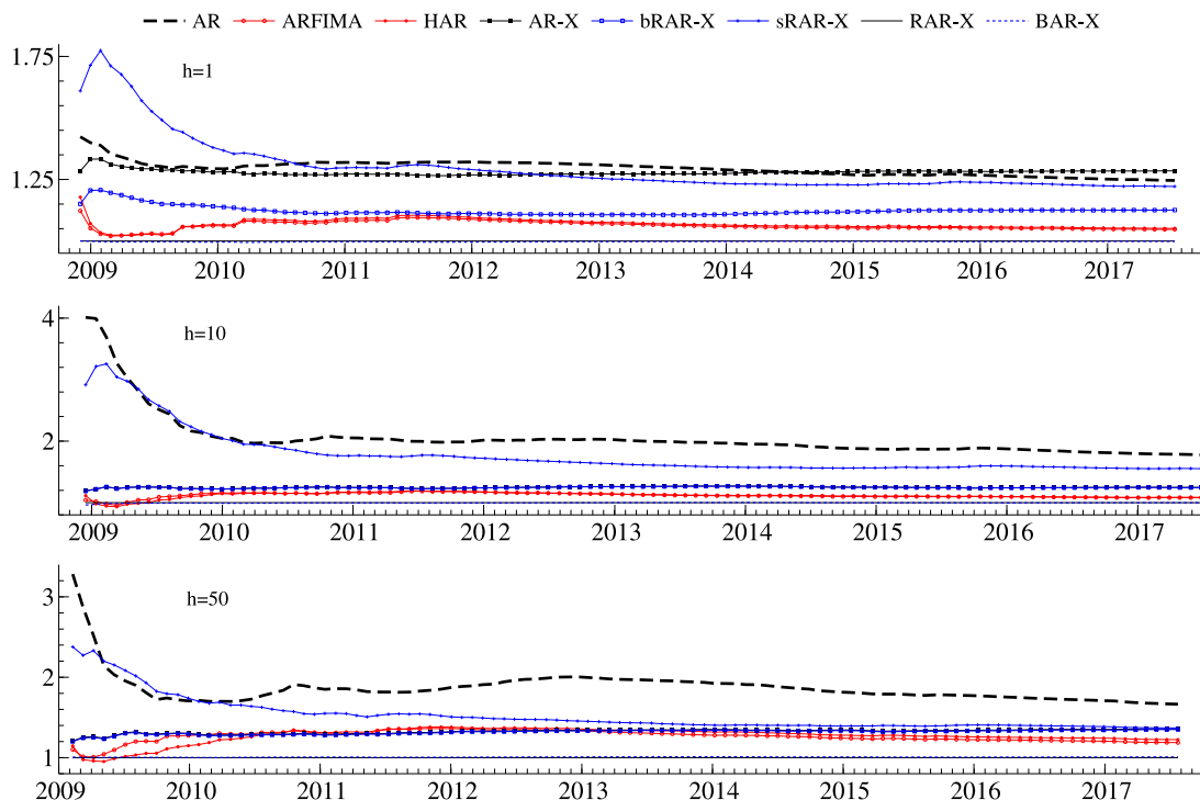
Fig. 2. Evolution of the ratio of the cumulative sum of squared forecast errors of each model with respect to the RAR-X model, over the sample period, for three forecast horizons ( h = 1, 10, 50 ). The models are the same as reported in Table 2.
