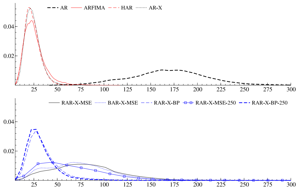
Fig. 4. Empirical distributions over 250 variables of BP(20) statistics computed for in-sample residuals. Each line corresponds to one of the models (estimated at horizon h = 1 ) presented in Table 4 (see the corresponding table note for definitions).
