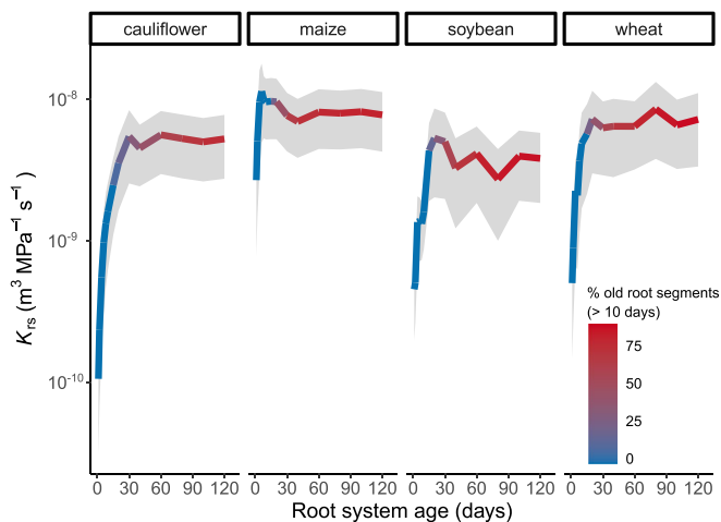
FIGURE 6 Modeled K_{rs} development with age in crop species. Colored lines and shaded areas represent K_{rs} (mean \pm standard error) of simulations using CPlantBox coupled with MARSHAL, for four different crops: cauliflower (forb), maize ( C_4 grass), soybean (legume) and wheat ( C_3 grass). The species were selected based on plant-functional diversity. The color scale indicates the proportion of old (>10 days) root segments in the total root system.
