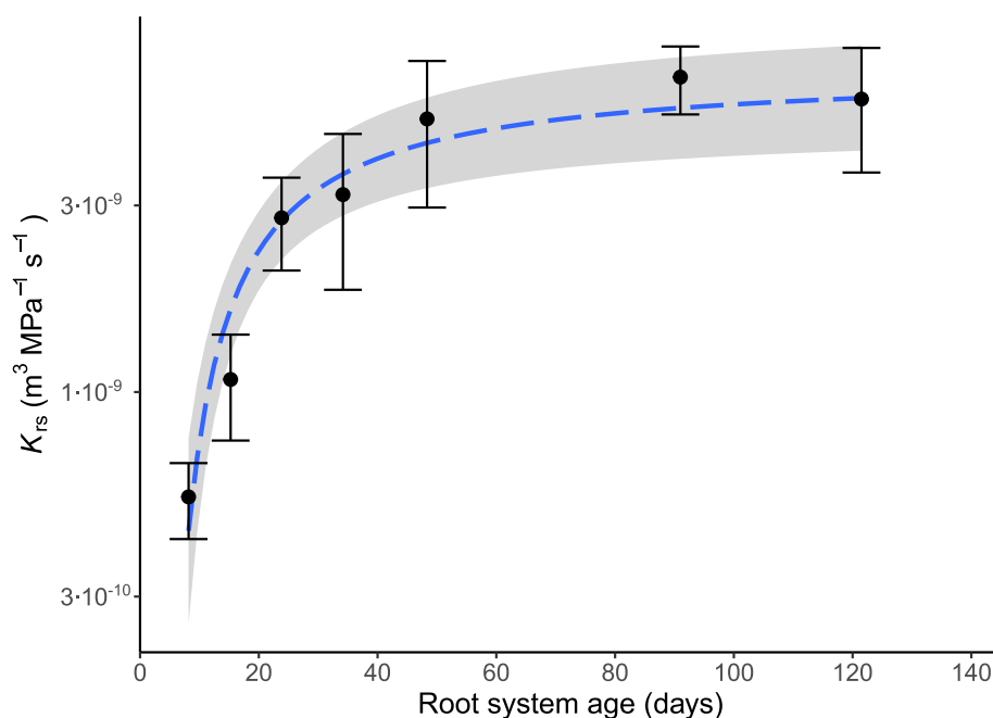
FIGURE 5 Relationship between root system age and K_{rs} in crop species. Data points and error bars represent K_{rs} (mean \pm standard error) of crop species (C 3 and C 4 grasses and dicot crops) grouped according to age (0–10, 10–20, 20–30, 30–40, 40–60, 60–100, >100 days). The dashed blue line and the shaded area represent a fitted exponential model ( \pm standard error).
