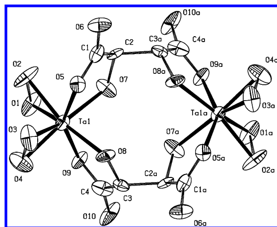
Figure 5. ORTEP plot of the molecular anion of 2b , [\text{Ta}_2(\text{O}_2)_4(\text{tart})_2]^{6-} (50% probability).
