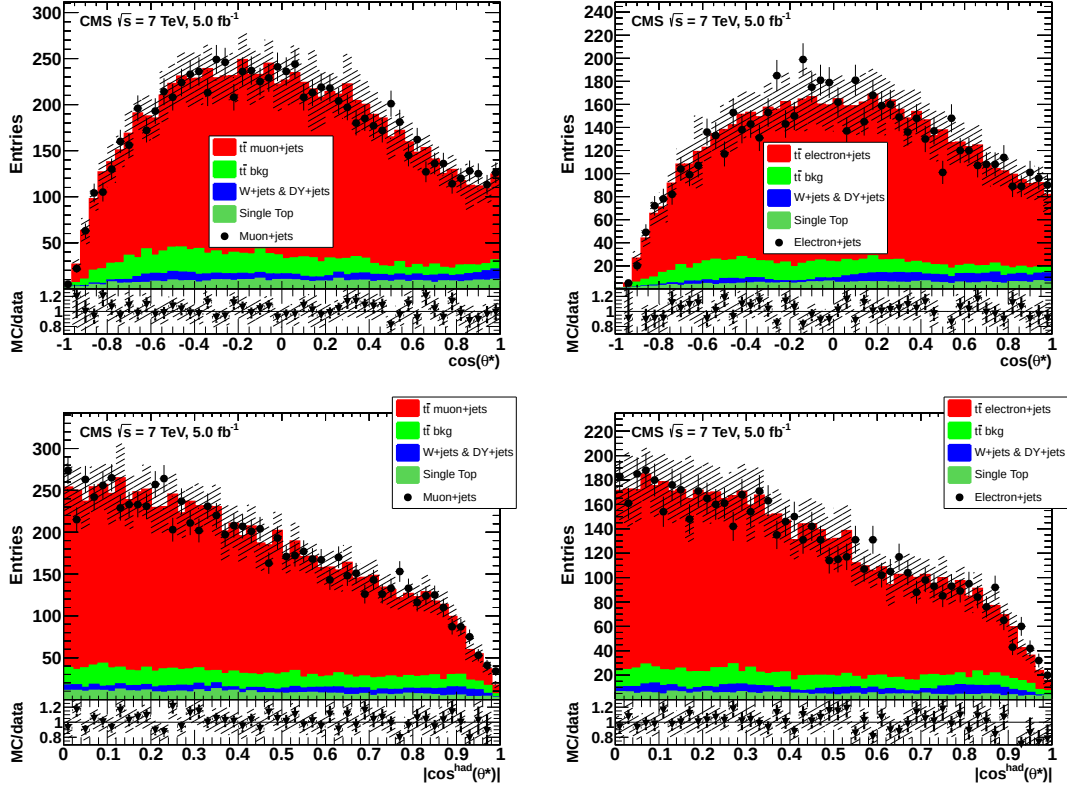
Figure 3: Cosine of the helicity angles \cos \theta^* (top) and |\cos^{\text{had}} \theta^*| (bottom) for the muon+jets (left) and electron+jets (right) channels. Data are displayed as solid points, simulated t\bar{t} signal distributions as red histograms, and the contribution from other background processes as coloured histograms. At the bottom, the ratio between prediction and data is displayed. Systematic uncertainties are shown as hatched histograms.
