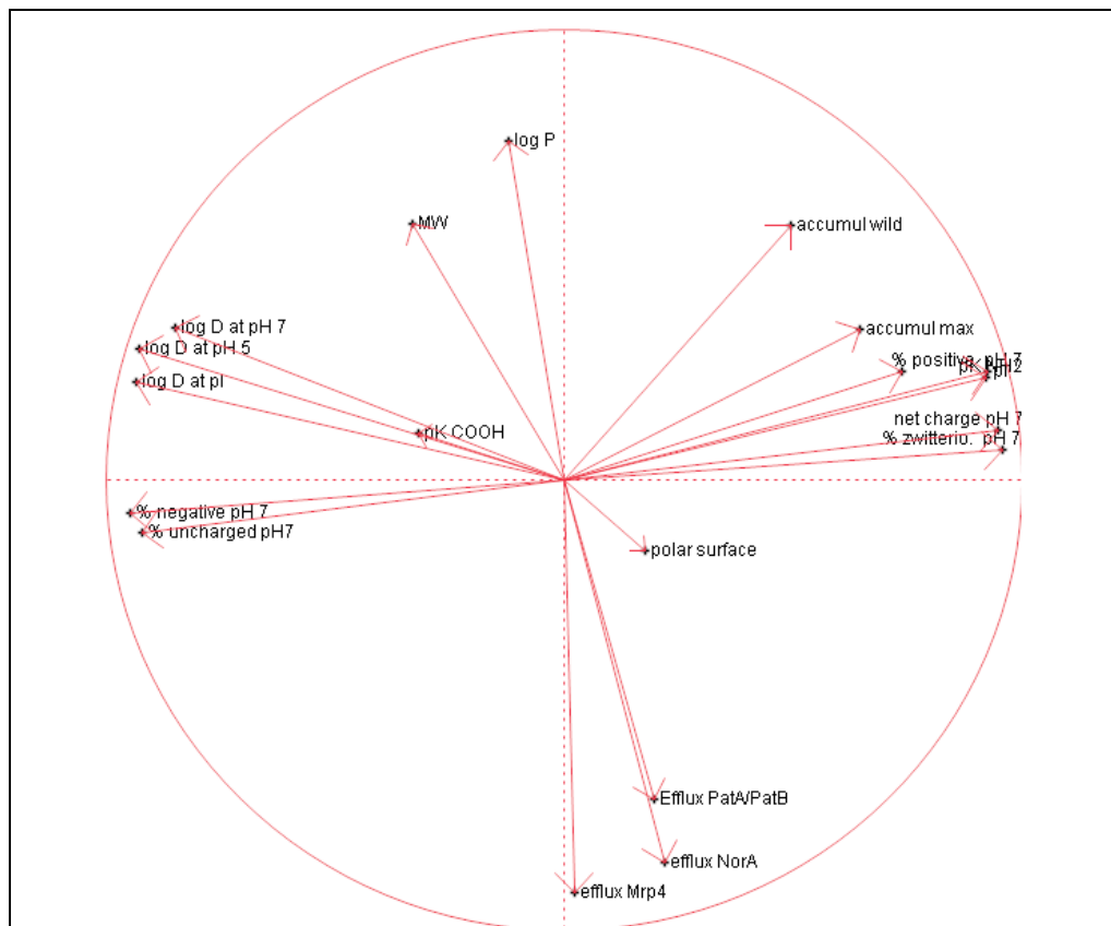
Figure 3. Principal component analysis of the correlations between physicochemical properties of fluoroquinolones and efflux mediated by Mrp4, NorA and PatA/PatB. The diagram shows a projection of multidimensional set of axes onto a 2-dimensional plane (arrows of the same length are on the same plane; arrows of different length have different orientations). The closeness of the arrows denotes the degree of correlation. Data analysis and graph generation with JMP software version 9.0.3.
