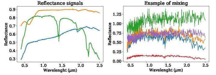
Fig. 1. Left: Reflectance signals of Andesine (blue), Celestine (orange) and Kaolinite (green). Right: Example of mixing of those signals. Each of the five signals is a column of Y .
