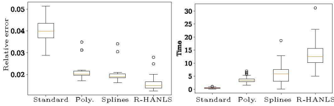
Fig. 3. Boxplots of the relative error (left) and the computation time (right), for different models solving NMF problem on mixture of signals presented in Figure 1.
