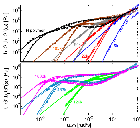
Figure 10. Experimental Storage (○) and loss (□) moduli of sample H3A1 H-polymer and of the linear matrices, at the master curve reference temperatures of 130 °C. The continuous curves correspond to the data predicted with the TMA tube model (see Section 4.1). The dashed curves for samples 483k have been obtained from creep measurements.
