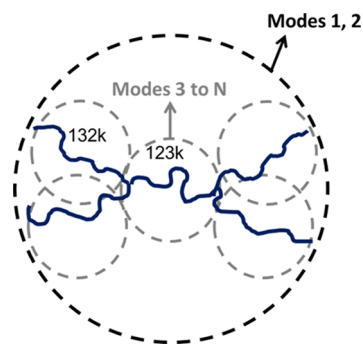
Figure 8. Description of the different Rouse modes present in the relaxation of unentangled H-polymer diluted in an oligomeric linear matrix. The gray circles define the longest molecular segment which can relax according to its intrinsic Rouse relaxation. The longest modes, 1 and 2, are possibly delayed by the slow motion of the branching points or self-entanglements.
