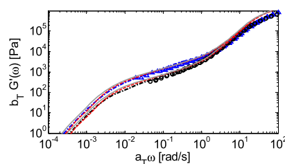
Figure 19. Comparison between experimental and theoretical linear rheology data of 1.5 wt % (exp. data: black o and dashed-dotted curve (creep)) and 3 wt % (exp. data: blue \Delta and dashed-dotted curve (creep)) of H-polymer diluted in the PSSk linear matrix, at T_{\text{ref}} = 130 °C. The data predicted with the exact Rouse model are shown by the continuous gray curve, whereas the data predicted with the approximated Rouse model are shown by the dashed red curves.
