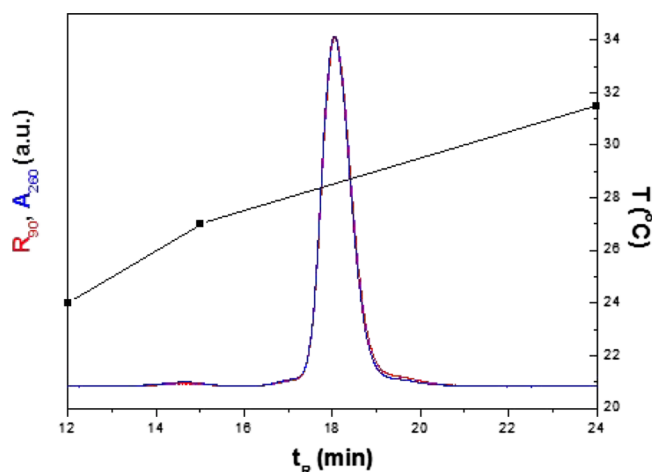
Figure 2. TGIC chromatogram of the H polystyrene H3A1. Separation condition: Nucleosil C18 (150 × 4.6 mm, 500 Å, 7 μm), CH 2 Cl 2 /CH 3 CN (58/42, v/v) at 0.5 mL/min. Temperature program is shown in the plot.
