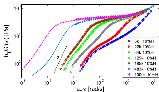
Figure 5. Linear viscoelastic storage modulus at T_{ref} = 130 °C of the binary blends composed of 10 wt % H3A1 and 90 wt % of linear PS of varying M_w (5k, 22k, 64k, 129k, 185k, 483k, and 1000k) samples. For samples 483k and 1000k, the continuous curves represent data obtained from creep measurements. In the former case, there is unambiguous evidence of the presence of a slow terminal mode (which is not fully detected), whereas in the latter case there is only a hint of possible (anticipated) slow mode.
