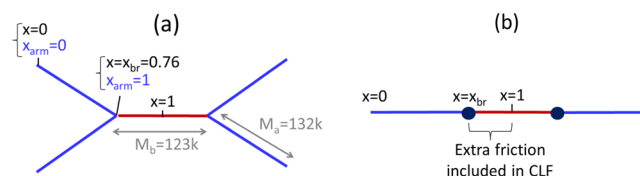
Figure 7. (a) H-polymer molecular coordinate systems. The first one, from the end of the branches, x_{\text{arm}} = 0 , to the branch point, x_{\text{arm}} = 1 , is used for determining the relaxation time of the molecular segments around the arms. The second one, from the end of the branches, x = 0 , to the middle of the backbone, x = 1 , is used to determine the relaxation time of the (inner) backbone. (b) At time longer than the relaxation time of the branches, these last ones are seen as extra friction points along the backbone of the H-polymer.
