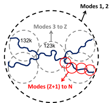
Figure 9. Description of the different Rouse modes present in the relaxation of H-polymer diluted in an entangled linear matrix. The red circles define the entanglement segments; the dashed gray circles define the longest molecular segment which can relax according to CRR motion, at the rhythm of the motion of the linear chains. The dashed black circle describes the longest modes, 1 and 2, which are possibly delayed by both the linear matrix and the slow motion of the branching points and/or the few H–H entanglements.
