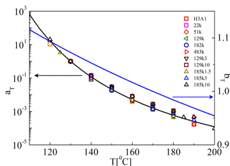
Figure 3. Horizontal a_T and vertical b_T shift factors associated to the PS linear and blend samples at T_{\text{ref}} = 130 °C.
