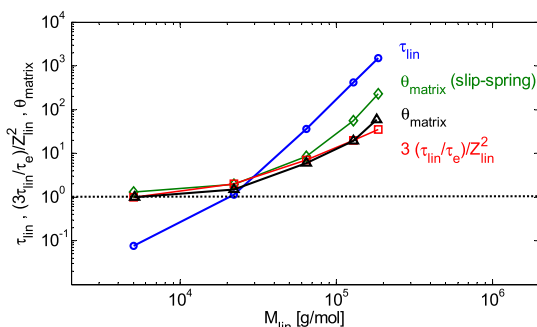
Figure 17. Retardation factor \theta_{\text{matrix}} ( \Delta ), \theta_{\text{matrix}} (slip-spring) ( \diamond ), relaxation time of the linear matrix \tau_{\text{lin}} ( \circ ), and ratio \frac{\tau_{\text{lin}}}{Z_{\text{lin}}^2} ( \square ) as functions of the molar mass of the linear matrix.
