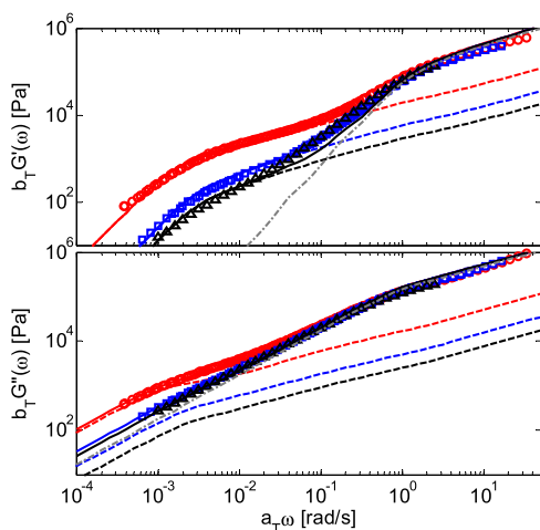
Figure 13. Storage G'(\omega) and loss G''(\omega) modulus data of 1.5% ( \Delta ), 3% ( \square ), and 10% ( \circ ) of H-polymer diluted in the linear matrix 22k, at T_{\text{ref}} = 130 °C. The experimental data (symbols) are plotted alongside the model data (continuous curves), as well as the deconvoluted linear (gray dashed-dotted curves) and H (dashed curves) contributions to the curves. The parameter \theta_{\text{matrix}} has been fixed to 1.5.
