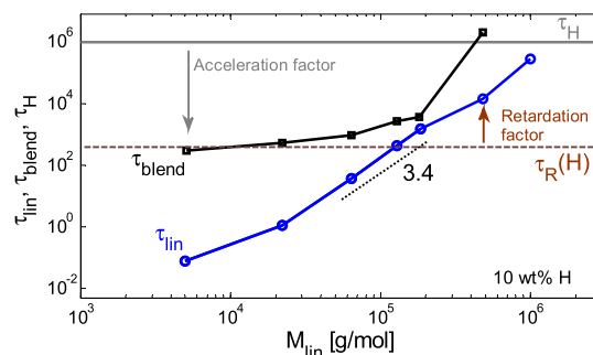
Figure 6. Comparison of the terminal relaxation time of blends with 10 wt % of H-PS, \tau_{blend} , and that of the linear matrix, \tau_{lin} , as a function of the molar mass of the latter, M_{lin} at 130 °C. The terminal time \tau_H and Rouse time \tau_R(H) of the monodisperse H-PS are indicated by horizontal full and dashed lines, respectively. The terminal times were determined experimentally by fitting the terminal regime with two lines of slopes 1 and 2 (for G'' and G' , respectively) and inverting the cross-over frequency. The only exceptions are the blends in the two largest molar masses linear matrices for which the terminal relaxation was too slow to be detected even by creep measurements. For the 483k matrix, the relaxation time was determined from the theoretical curves and involves some uncertainty. This was not attempted for the 1000k matrix because the uncertainty is huge (see also Figure 5).
