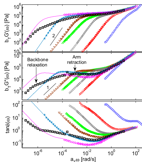
Figure 4. Experimental storage and loss moduli and \tan \delta master curves of H-PS sample H3A1 (thick black \square ) and of the linear matrices (5k (blue \circ ), 22k (red \triangle ), 64k (gray \diamond ), 129k (green \triangle ), 185k (brown \nabla ), 483k (cyan * ), and 1000k (violet \triangleleft )), at the reference temperature of 130 °C for samples PS64k, PS129k, PS185k, and PS483k, respectively, and at iso- T_g condition for the other samples, with (T_{\text{ref}} - T_g) = 24 °C (see Section 3.1). Continuous curves represent data obtained from creep measurements. The arrows indicate the relaxation peaks of the arms and backbone of the H polymer.
