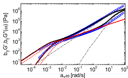
Figure 12. Comparison between experimental (O) and theoretical (continuous black curves) linear rheology data of 10 wt % of H-polymer diluted in the PS5k linear matrix, at T_{\text{ref}} = 130 °C. The parameter \theta_H has been fixed to 2. The curves represent the contributions of the H-polymer (continuous red) and the linear matrix (dashed-dotted gray) to the moduli. The dashed red curves correspond to the predictions with \theta_H = 1 .
