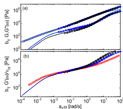
Figure 11. (a) Comparison between experimental (symbols and dashed curves) and theoretical (continuous curves) linear rheology data of 1.5 wt % (exp. data: black ○ and dashed curve (from creep); predicted data: continuous gray curve) and 3 wt % (exp. data: blue Δ and dashed curve (from creep); predicted data: continuous light blue curve) of H-polymer diluted in the PS5k linear matrix, at T_{\text{ref}} = 130 °C. The parameter \theta_{\text{H}} has been fixed to 1. (b) Experimental storage modulus of 1.5 wt % (○), 3 wt % (Δ), and 10 wt % (□) of H-polymer diluted in the PS5k linear matrix, vertically shifted by dividing G'(\omega) by the volume fraction of H-polymer, \nu_{\text{H}} .
