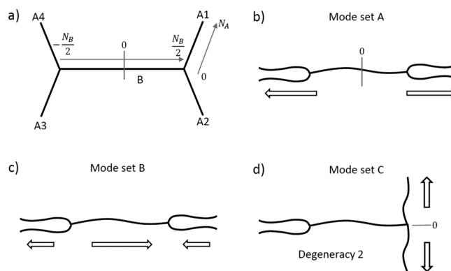
Figure 18. (a) Chain co-ordinates used for H-polymer modes. Backbone co-ordinate runs from -N_B/2 to N_B/2 . Arm co-ordinates run from 0 (at branchpoint) to N_A . (b) Symmetry of mode set A—symmetric along molecule length with displacement node at the center of the backbone. (c) Symmetry of mode set B—symmetric along the molecule length with displacement maximum at the center of the backbone. (d) Symmetry of mode set C—symmetric along arms at one end of the molecule with node at the branchpoint and rest of the molecule undisplaced. These modes have degeneracy 2. In all cases (mode A, B, and C), the slowest mode of the set is shown, but higher modes have the same symmetry.
