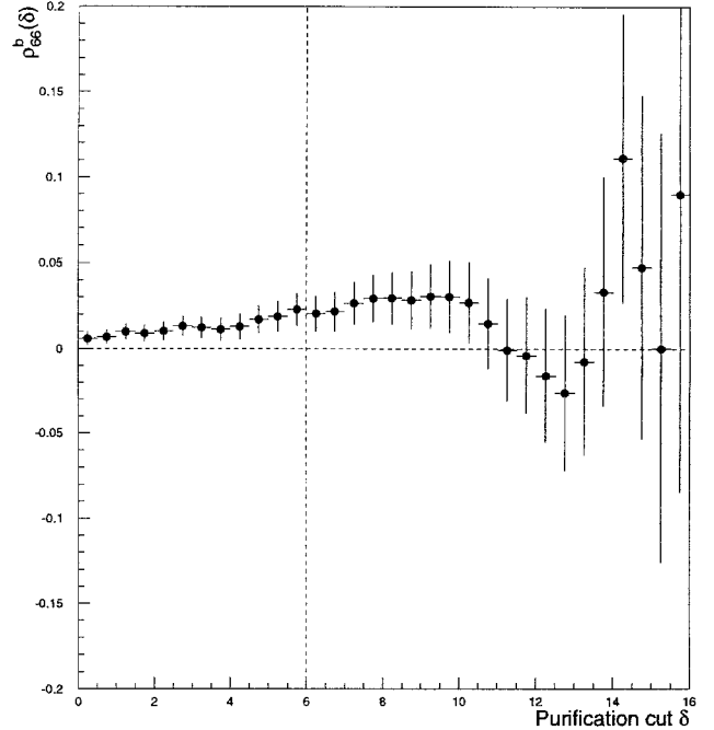
Fig. 13. Double tag hemisphere correlation factor ( I = 6, J = 6 ), as a function of \delta . For the standard cut at \delta = 6 , the value of \rho_{66}^b is 0.018 \pm 0.010 and it remains rather stable over the whole range. Note that, by definition of \rho_{66}^b , the points are bin-to-bin correlated
