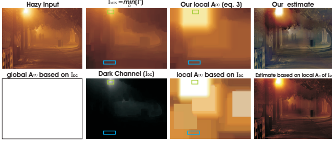
Fig. 3. Local airlight estimation. A global estimate of the A_{\infty} based on dark channel results in a white airlight. As a consequence, the dark channel might become very small (see blue rectangle in second image of bottom row), which means 1 - T(x) \approx 0 in Equation 2 and no airlight influence in Equation 1. In contrast, our local airlight estimate on the same blue rectangle results in a colored atmospheric light, which in turns results in a non-unity transmission and a non-zero atmospheric light influence.
