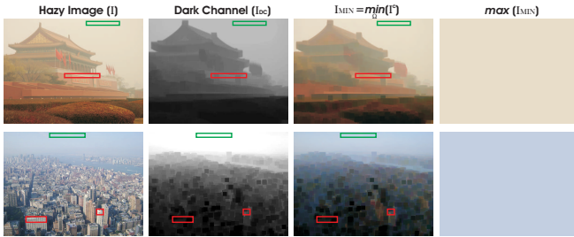
Fig. 4. Airlight estimation. Our global airlight estimate A_{L\infty}^c , derived by maximizing \min_{y \in \Omega(x)} (I^c(y)) over the entire image, appears to be quite similar to the atmospheric intensity estimated by He et al. [16], from the brightest region of the dark channel (depicted by green rectangles). The red rectangles show that, in daytime scenes, the two approaches equally reject the high image intensity locations that are not relevant regarding airlight estimation. He et al. [16] method rejects them because the prior is dark in those regions, our strategy because I_{MIN} gets darker than the initial image in those regions that are not subject to intense airlight illumination. Since I_{MIN} does not make any implicit assumption about the whiteness of the atmospheric illumination, it is more general than [16], especially in presence of artificial colored lighting.
