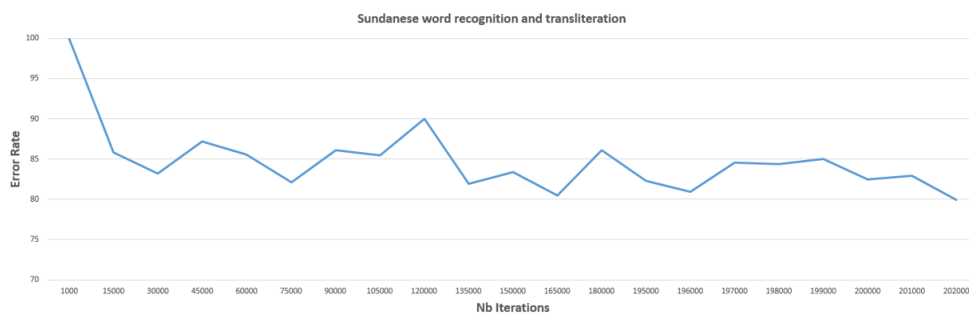
Figure 28. Error rate for Sundanese word recognition and transliteration test set.
