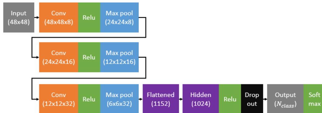
Figure 10. Architecture of the CNN.
