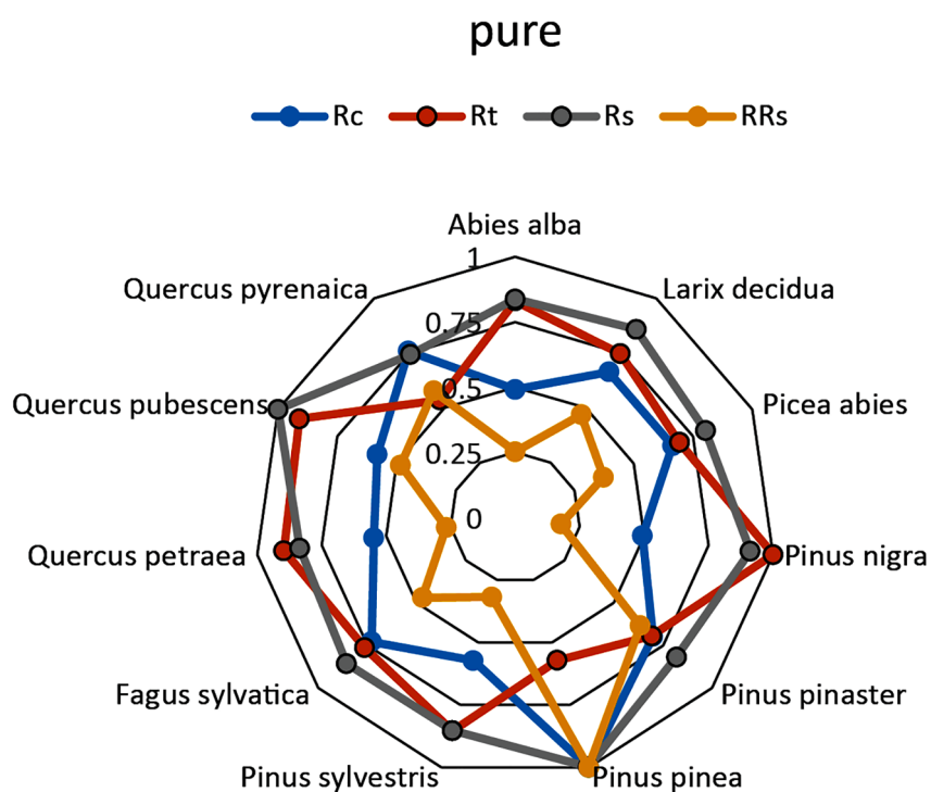
Fig. 4. Amoeba diagrams for pure and mixed stands representing Resistance (Rt), Recovery (Rc), Resilience (Rs) and Relative Resilience (RRs) for the eleven species studied. The value 1 represents the maximum value observed for Rt, Rc or Rs in pure or mixed stands.
