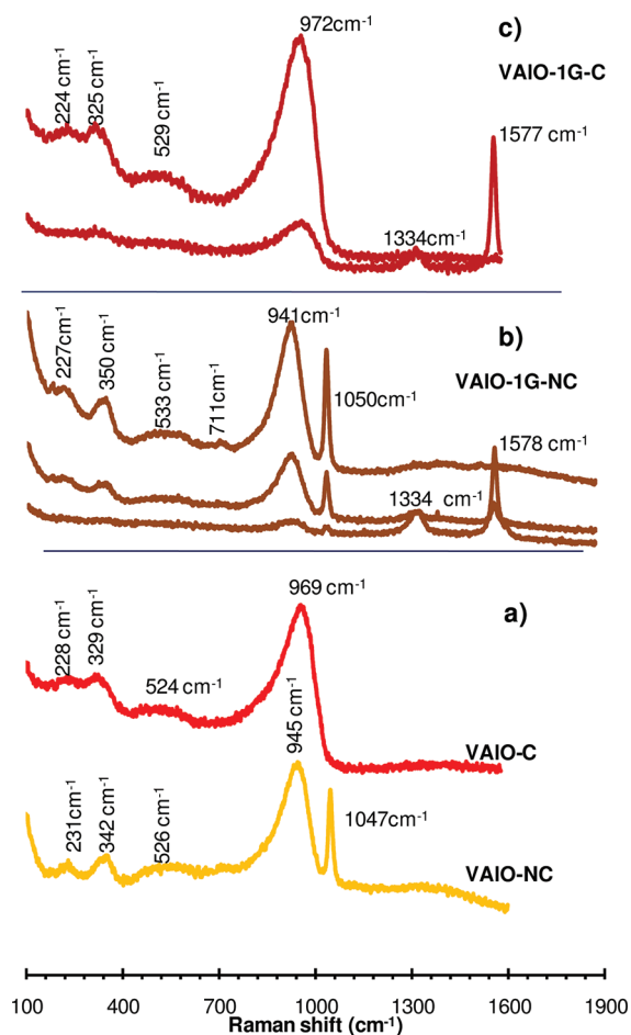
Figure 7. Raman spectra of selected VAIO-xG-NC/C: (a) Pure VAIO before and after calcination; (b) Spectra registered for three different particles of VAIO-1G-NC; and (c) spectra recorded for two different particles of VAIO-1G-C.
