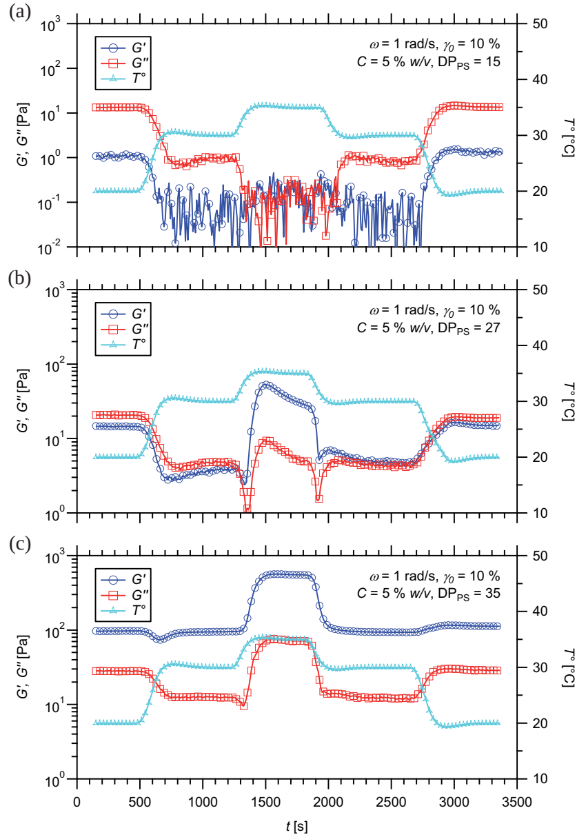
Figure 12.14 – Time dependence of dynamic moduli for hydrogels prepared from \text{PS}_m\text{-}b\text{-PNIPAAm}_{235}\text{-tpy} copolymers with increasing PS segment length and Ni(II) ions, at different temperatures.
