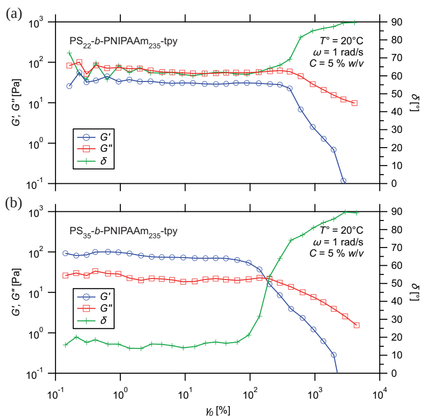
Figure 10.16 – Strain dependence of dynamic moduli for hydrogels prepared from (a) \text{PS}_{22}\text{-}b\text{-PNIPAAm}_{235}\text{-tpy} or (b) \text{PS}_{35}\text{-}b\text{-PNIPAAm}_{235}\text{-tpy} copolymer and \text{Ni(II)} ions.
