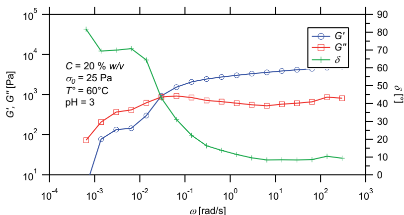
Figure 12.11 – Frequency dependence of dynamic moduli for hydrogels prepared from PNIPAAm 45 - b -PDMAEMA 105 -tpy copolymer and Ni(II) ions, at 60 °C and pH 3.
