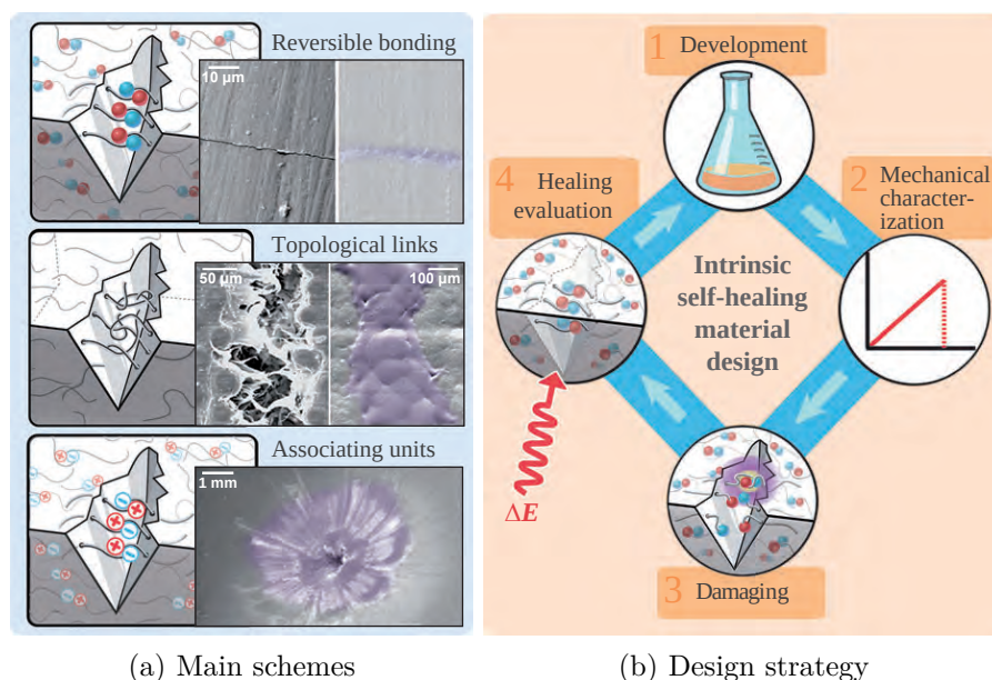
Figure 2.10 – Achieving reparation and design strategy of intrinsic self-healing materials. [59]
