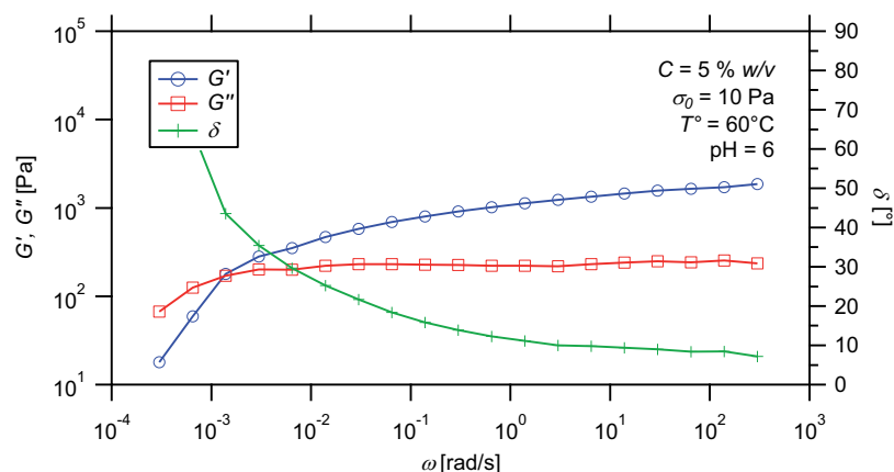
Figure 12.29 – Frequency dependence of dynamic moduli for a hydrogel prepared from PS 12 - b -PNIPAAm 75 - b -PDMAEMA 105 -tpy copolymer and Ni(II) ions, at 60 °C.
