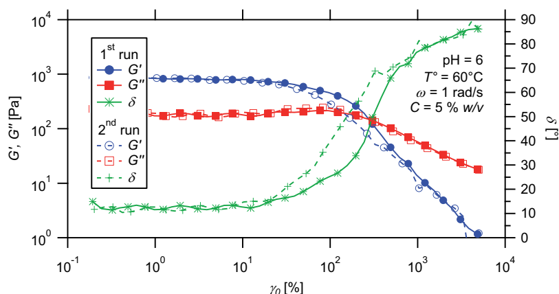
Figure 12.31 – Strain dependence of dynamic moduli for a hydrogel prepared from PS 12 - b -PNIPAAm 75 - b -PDMAEMA 105 -tpy copolymer and Ni(II) ions, at 60 °C: 1 st run under increasing strain, 2 nd run under decreasing strain.
