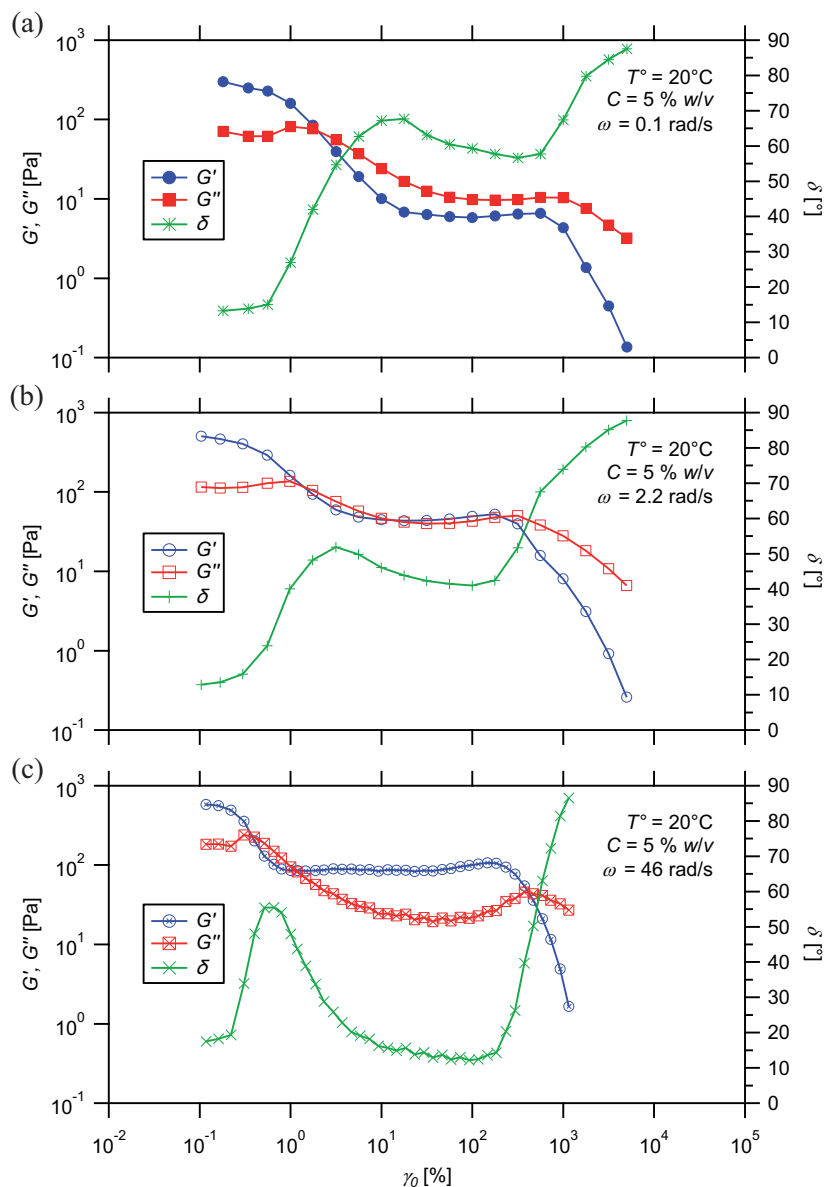
Figure 10.11 – Strain dependence of dynamic moduli for a hydrogel prepared from PS 27 - b -PNIPAAm 235 -tpy copolymer and Ni(II) ions, at selected oscillation frequencies.
