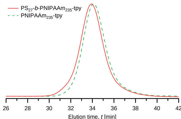
Figure 8.12 – SEC elutograms of PNIPAAm-tpy homopolymer and derived PS- b -PNIPAAm-tpy copolymer.
