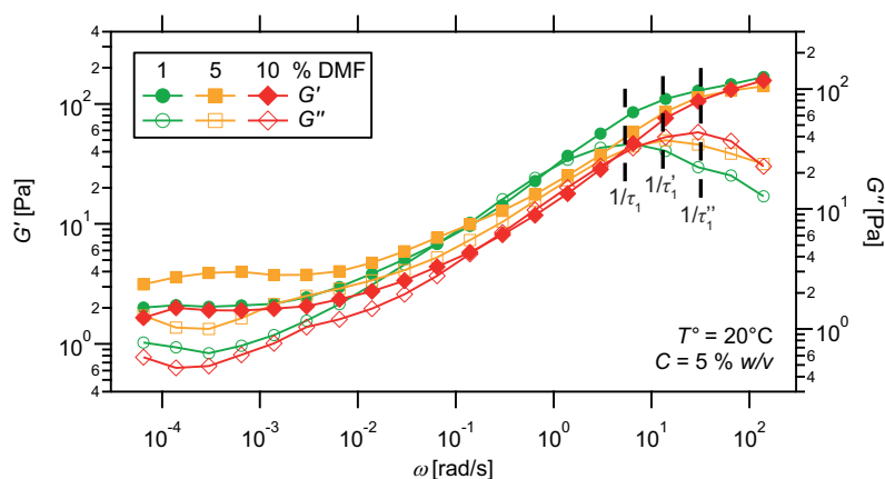
Figure 12.2 – Dynamic mechanical response of hydrogels prepared from PS 27 - b -PNIPAAm 300 -tpy copolymers and Ni(II) ions, with increasing amount in DMF.
