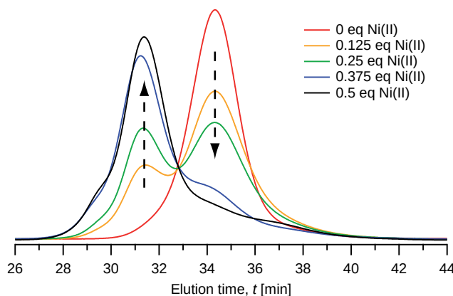
Figure 9.5 – Evolution of molar mass distribution of a PNIPAAm- b -PDMAEMA-tpy copolymer with the addition of Ni(II) ions.
