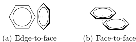
Figure 2.7 – Two main geometries for \pi - \pi interactions.
