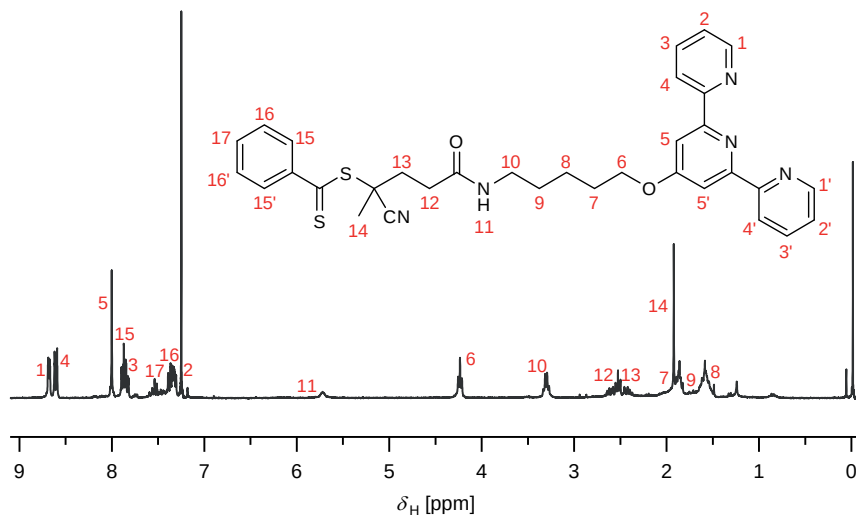
(b) ^1\text{H} -NMR spectrum of CPAD-tpy
