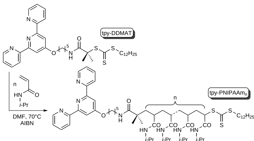
Scheme 8.3 – Synthesis of PNIPAAm-tpy homopolymers.
