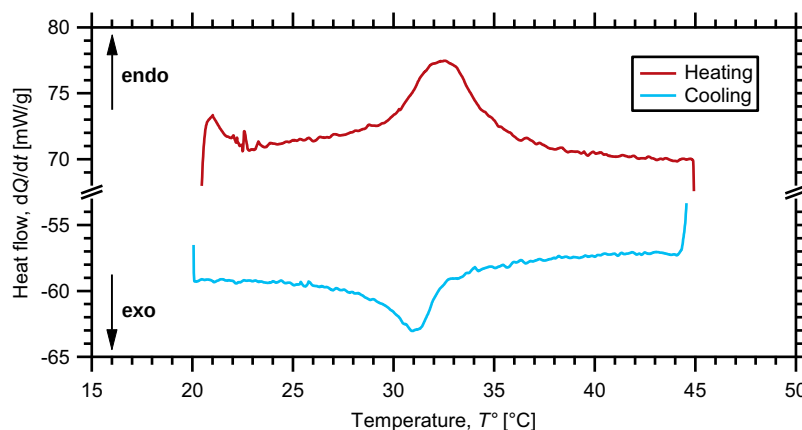
Figure 9.29 – DSC thermogram of a 5 %w/v hydrogel prepared from PS 27 - b -PNIPAAm 300 -tpy copolymer and Co(II) ions.
