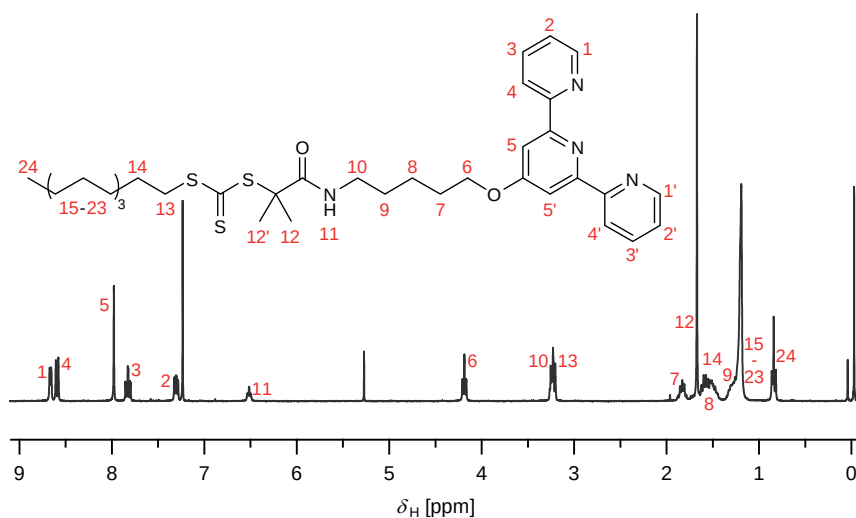
(a) ^1\text{H} -NMR spectrum of DDMAT-tpy
