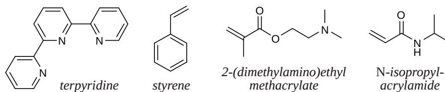
Figure 8.1 – Structures of monomers and ligand used in the synthesis of functional building blocks.
