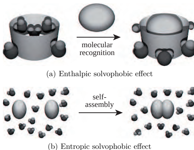
Figure 2.8 – Energetic components of the solvophobic interactions. [16]
