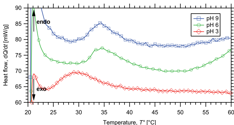
Figure 9.30 – DSC thermogram of 20 %w/v hydrogels prepared from PNIPAAm 45 - b -PDMAEMA 105 -tpy copolymer and Ni(II) ions, at different pH.
