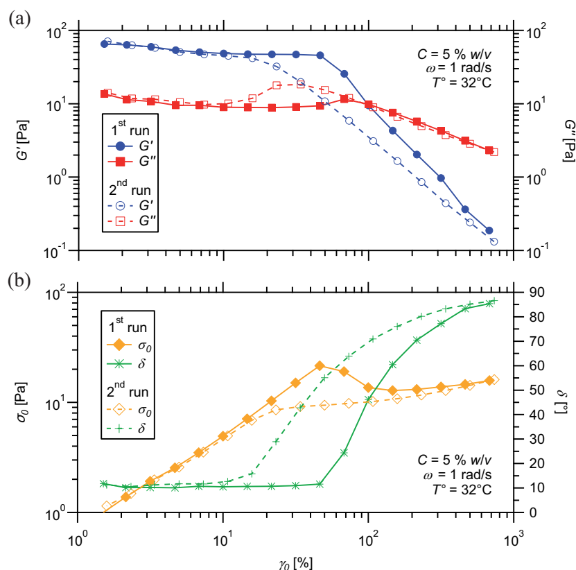
Figure 12.19 – Strain dependence of (a) dynamic moduli and (b) stress amplitude for a hydrogel prepared from PS 27 - b -PNIPAAm 300 -tpy copolymer and Co(II) ions, at 32°C: 1 st run under increasing strain, 2 nd run under decreasing strain.
