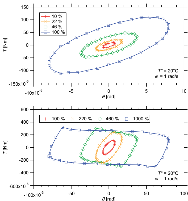
Figure 10.9 – Lissajous patterns obtained for a hydrogel prepared from PS 27 - b -PNIPAAm 235 -tpy copolymer and Ni(II) ions, at various strain amplitudes.
