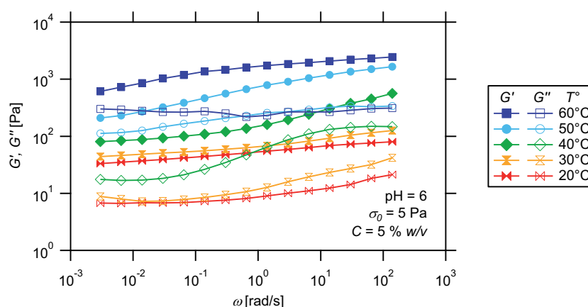
Figure 12.28 – Frequency dependence of dynamic moduli for a hydrogel prepared from PS 12 - b -PNIPAAm 75 - b -PDMAEMA 105 -tpy copolymer and Ni(II) ions, at different temperatures.
