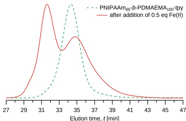
Figure 9.4 – SEC elutograms of a PNIPAAm- b -PDMAEMA-tpy copolymer and its iron(II) bis-complex.
