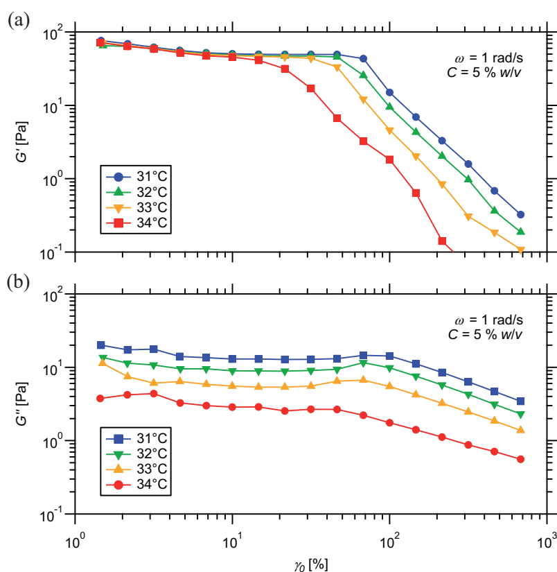
Figure 12.21 – Strain dependence of (a) elastic and (b) viscous moduli for a hydrogel prepared from PS 27 - b -PNIPAAm 300 -tpy copolymer and Co(II) ions, at different temperatures.
