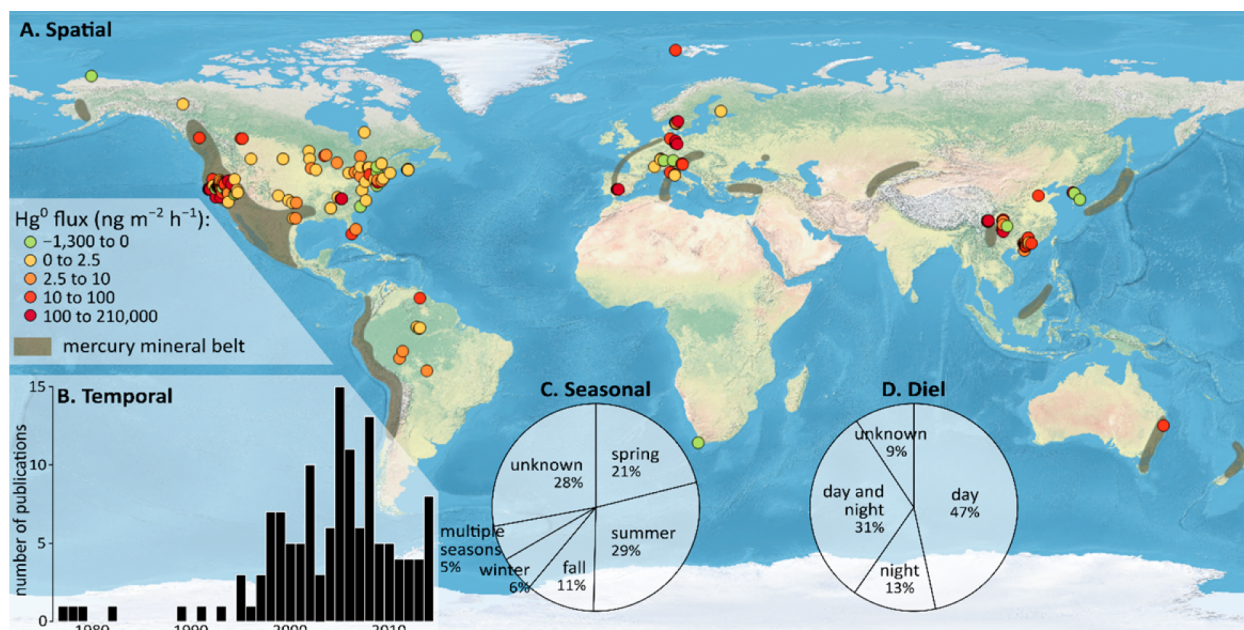
Figure 1. Coverage of study sites by averaged Hg 0 flux (the brown areas correspond to the terrestrial mercury mineral belts, 58,59 A), number of publications per year along with (B), seasonal (C) and diel (D) proportions of measurements.
