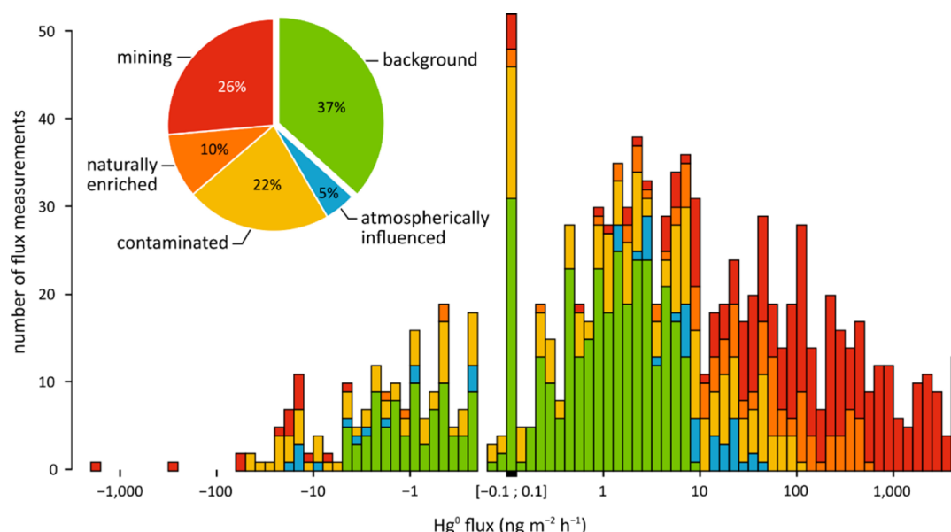
Figure 2. Distribution of \text{Hg}^0 fluxes by contamination class (logarithm scale for x -axis shows both positive (emission) and negative (deposition) fluxes).
