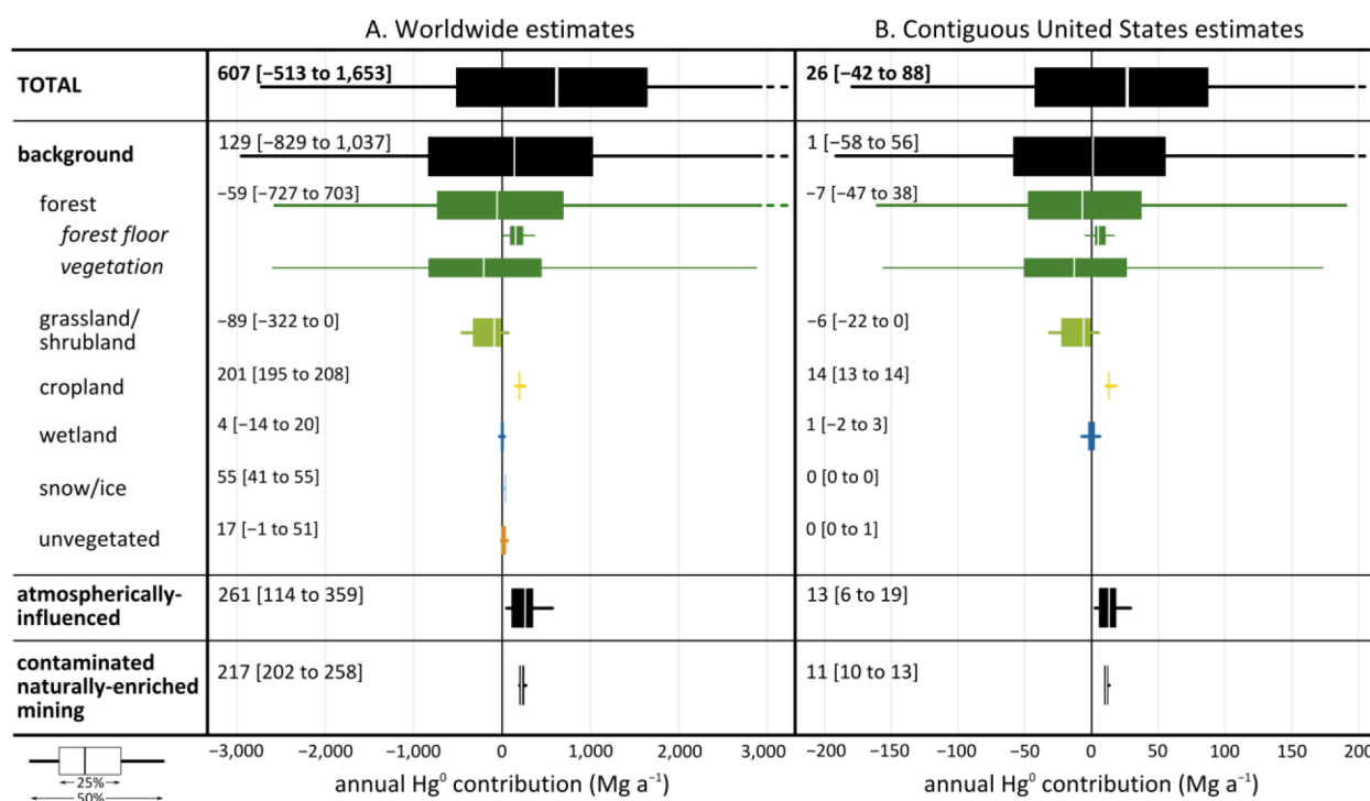
Figure 7. Global annual estimates of \text{Hg}^0 exchange ( \text{Mg}\cdot\text{a}^{-1} ) over terrestrial surfaces across different land covers: worldwide (A) and the contiguous United States (B). Positive values signify emissions, and negative values signify deposition. Numbers indicate medians and uncertainty ranges between 37.5th and 62.5th percentiles. Background represents the sum of six subcategories (forest, grassland/shrubland, cropland, wetland, snow/ice, and unvegetated (i.e., bare soils)). Forest fluxes were calculated based on forest floor \text{Hg}^0 flux measurements and leaf fluxes multiplied by leaf area indices since whole-ecosystem forest fluxes are largely missing in the literature.
