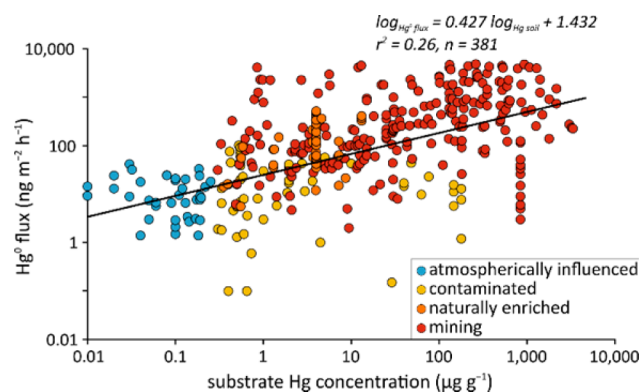
Figure 5. \text{Hg}^0 flux vs substrate Hg concentration relationship for Hg-enriched sites.
