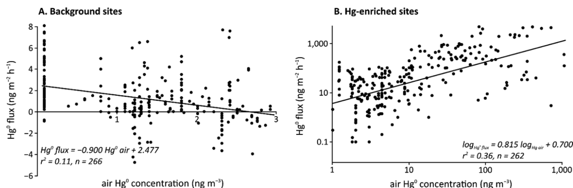
Figure 4. \text{Hg}^0 flux vs air \text{Hg}^0 concentration relationship: background (A) and Hg-enriched (B) sites.
