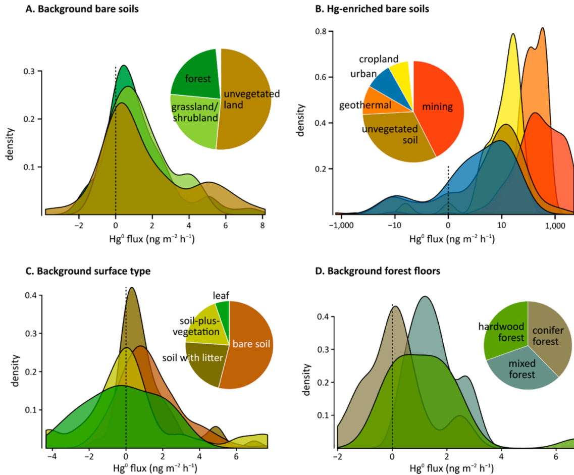
Figure 3. Distribution density of \text{Hg}^0 fluxes from background (A) and Hg-enriched (B) bare soils by land cover ( n > 10 ), background surfaces by vegetation cover type (C), and background forest floors by forest type (D). Only classes with n > 10 are presented.
