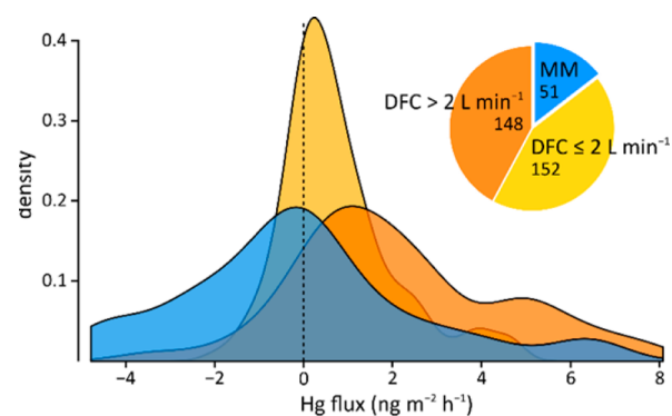
Figure 6. Methodological influence on \text{Hg}^0 flux measurements in background sites: distributions obtained by MM, DFC with a flushing flow rate \leq 2 \text{ L min}^{-1} , and DFC with a flushing flow rate > 2 \text{ L min}^{-1} .
