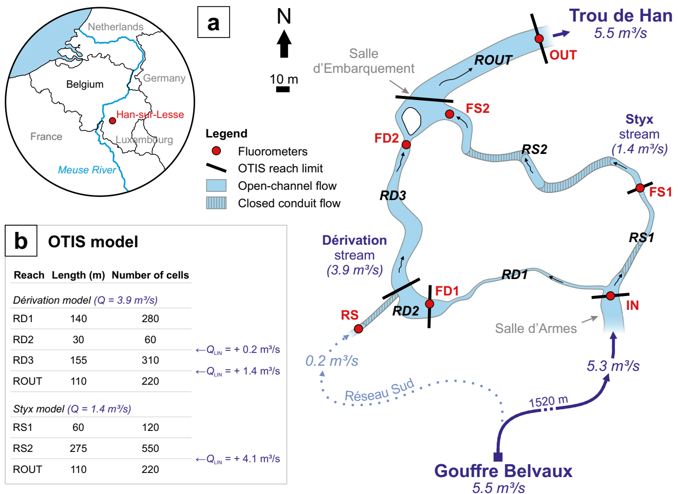
Fig. 1 a The diffifluence-confluence system of the Han-sur-Lesse Cave in Belgium, and location of the fluorometers for the tracer tests campaign; b OTIS model reaches and their respective lengths and cell numbers
