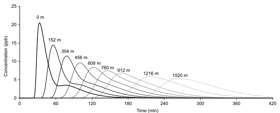
Fig. 9 Evolution of OTIS-simulated BTC at the outlet OUT as the injection is made further upstream from the diffidence. The distances are associated with reach lengths reduced to 0, 10, 20%, ... of the original length (1,520 m). As the distance increases, a merging of the two peaks makes the BTC single-peaked, thus making the observation of a DC system impossible for distal injections (more than 760 m)
