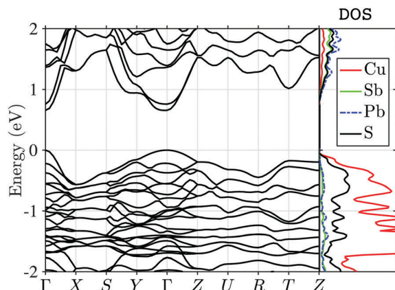
Fig. 6 The band structure and atom-projected density of states of CuPbSbS 3 . See Fig. S2–S4 (ESI†) for projected band structures of selected compounds as well as those calculated with spin orbit coupling for selected compounds.
