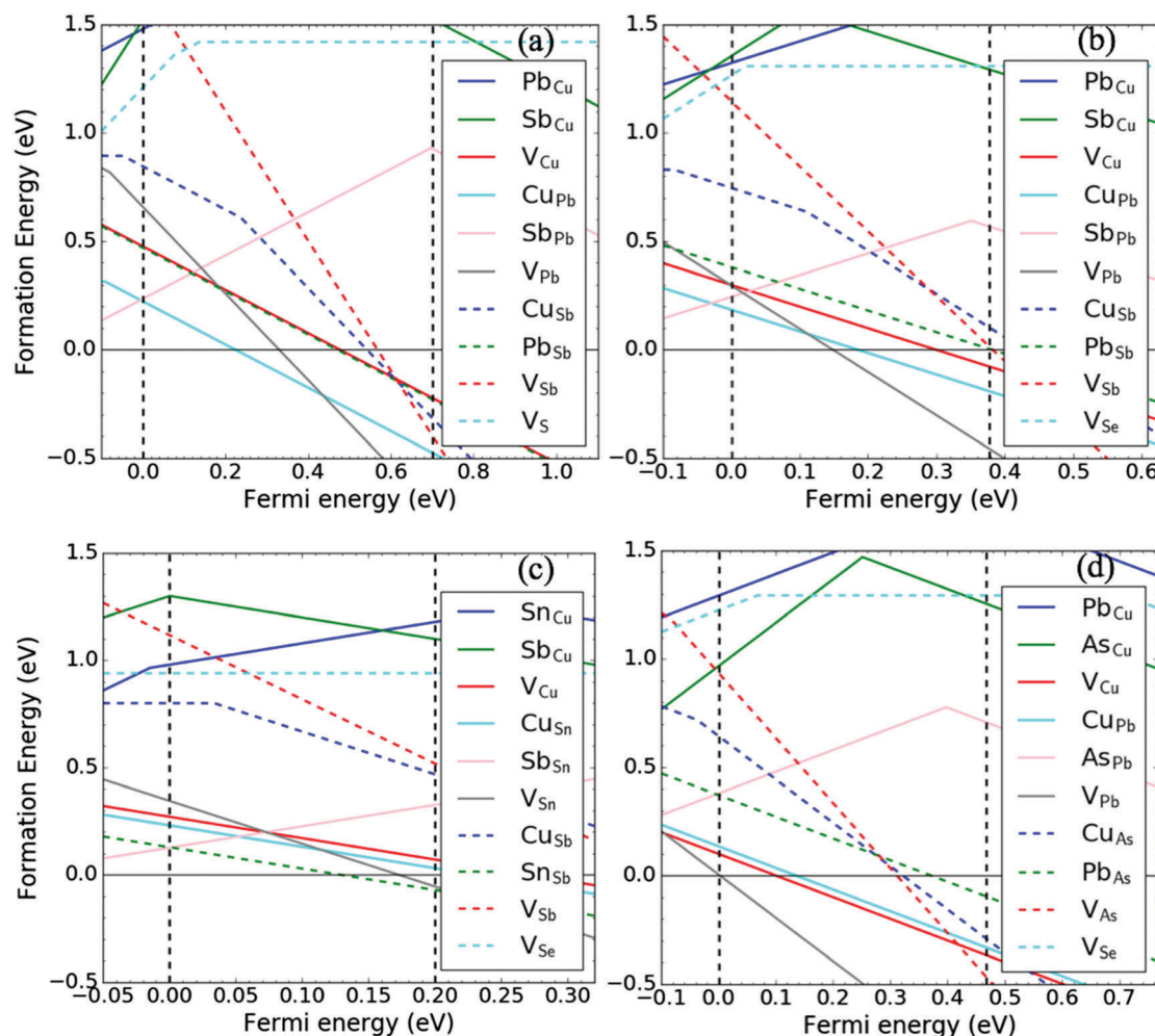
Fig. 3 Formation energies of intrinsic defects for (a) \text{CuPbSbS}_3 , (b) \text{CuPbSbSe}_3 , (c) \text{CuSnSbSe}_3 and (d) \text{CuPbAsSe}_3 . The chemical potentials (values are listed in the ESI†) are taken from a single region of the phase diagram that results in the lowest energy for shallow acceptors ( \text{Cu}_{\text{Pb}} , \text{Cu}_{\text{Pb}} , \text{Sn}_{\text{Sb}} and \text{V}_{\text{Pb}} , respectively) in order to optimize p-doping. The two dashed vertical lines represent the VBM and CBM. All three a, b, c diagrams indicate strong p-type preference with potential for enhancement through Sb-poor synthesis. Defect diagram of \text{CuPbAsSe}_3 shows strong intrinsic p-type characteristic. See Fig. S6–S13 (ESI†) for further diagrams containing both the intrinsic defects at all chemical potentials as well as extrinsic defects for \text{CuPbSbS}_3 . We note that the symbol “V” indicates a vacancy in these plots, not the element vanadium.
