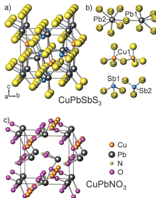
Fig. 1 (a) Crystal structure CuPbSbS 3 . (b) The local bonding environments of CuPbSbS 3 : Pb neighbors 6 and 7 S atoms, with Cu in tetrahedral and Sb in trigonal pyramidal coordination environments. (c) Crystal structure of DFT-optimized CuPbNO 3 : the bournonite-type structure is not retained upon cell and atom position optimization, even though the spacegroup number (31) remains the same.
