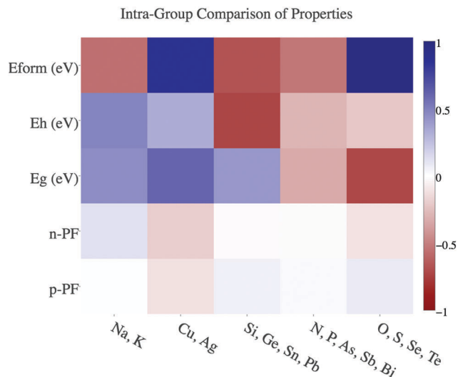
Fig. 5 A visualization of trends in property changes of bournonite when substituting elements by moving down a group. The number of times that a property increases or decreases when we replace one element in ABCD_3 with a heavier element immediately lower (e.g. Si/Ge not Si/Sn) in the periodic table divided by the total number of comparisons presented in a scale -1 (always decreasing) to 1 (always increasing). Darker colors represent a more consistent change of that property, e.g., there is a strong tendency for band gaps to decrease for heavier anion (dark red for row E_g , column O, S, Se, Te). For more details, see the accompanying text.
