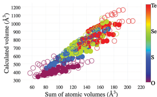
Fig. 2 The DFT optimized volume plotted against the sum of atomic volumes determined by the composition (both in Å 3 ). The colors separate compounds based on their anion. The overall volume is to a large extent determined by the size of their constituent atoms. Filled markers indicate that the structures are similar to bournonite while the open markers are structures relaxed to non-bournonite arrangements.
