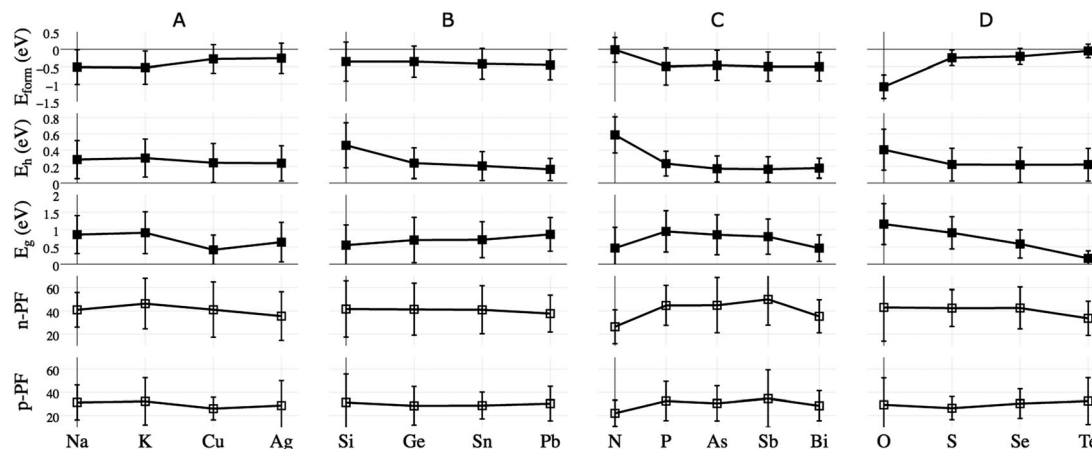
Fig. 4 Overview of how elemental substitutions affect the several properties of bournonite. The average of the properties and their change within each group is plotted. The error bars indicate standard deviation in calculated values when one element is held fixed but others are allowed to vary. For n-PF and p-PF, the results are in the units of \mu\text{W cm}^{-1} \text{K}^{-2} . Open symbols mean that not all data is available in the average, e.g., due to unconverged calculations. An analysis of trends is presented in the discussion.
