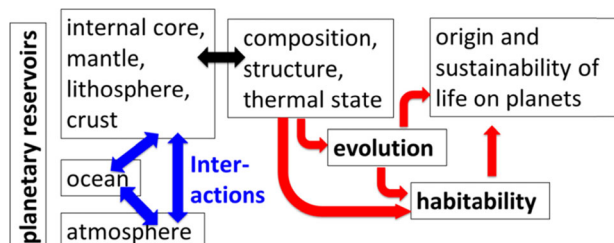
Fig. 1 Sketch on the themes involved in Planet TOPERS. Note that this sketch is done for all terrestrial planets including the Earth
