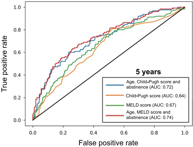
FIGURE 3 Receiver operating characteristic curves of the different models in the derivation data set.
