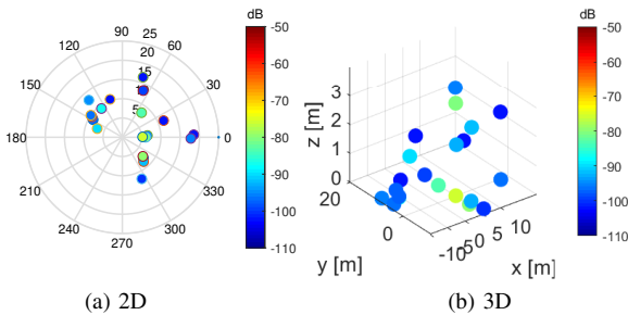
Fig. 4. Omnidirectional PADP extracted from VCA measurements.
