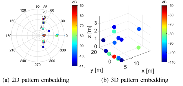
Fig. 5. PADP with T-RIS embedding for \phi_s = 0^\circ .
