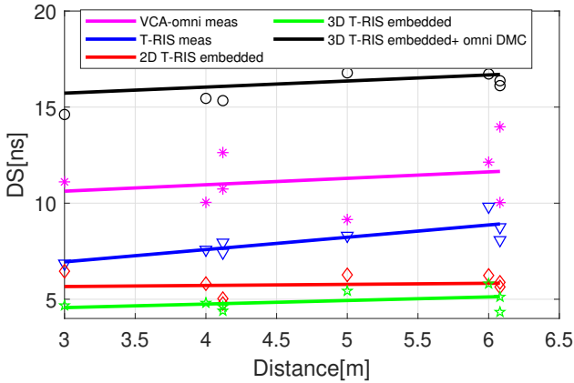
Fig. 10. Delay Spreads comparison: measurements vs models.
