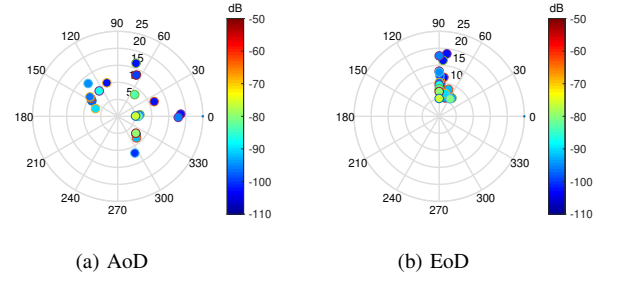
Fig. 3. Power Angular Delay Profile (PADP) extracted from VCA measurements in the azimuth plane (a) and elevation plane (b) for receiver position RX5.
