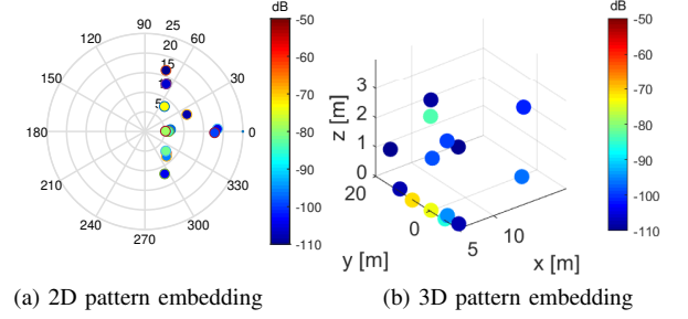
Fig. 6. PADP with T-RIS embedding for \phi_s = 50^\circ .
