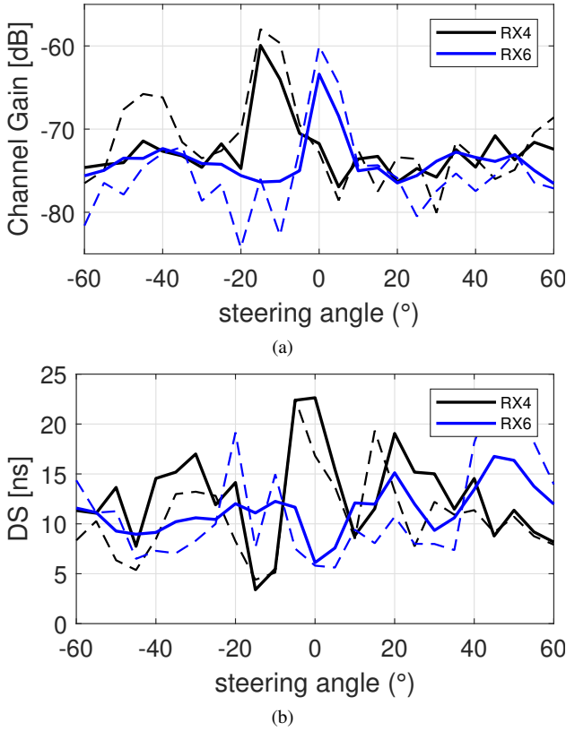
Fig. 7. Channel gain (a), Delay spread (b) as a function of steering angle: measured (solid) vs 3D T-RIS embedding (dotted line).
