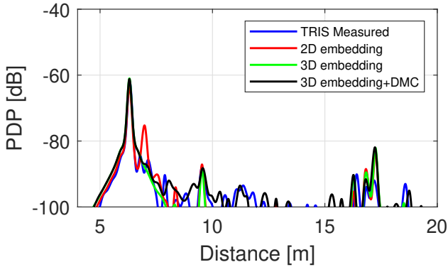
Fig. 8. Example of PDP comparison: actual measured PDP vs synthesized PDPs.
