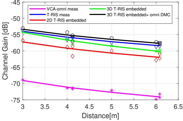
Fig. 9. Channel gain comparison: measurements vs models.
