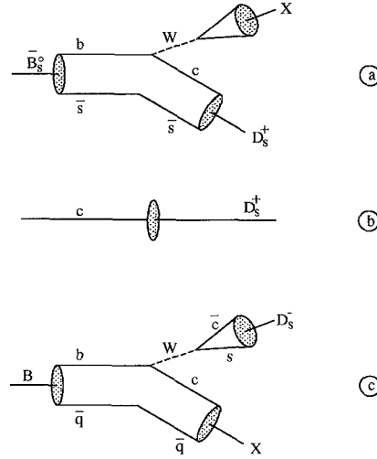
Fig. 1a–c. Quark diagrams contributing to inclusive D_s meson production
