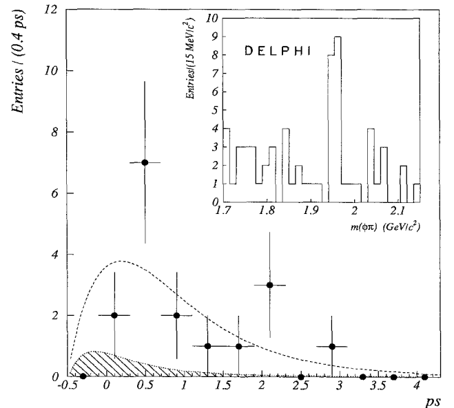
Fig. 5. The measured B proper time distribution for the D_s sample, shown by the points with the error bars. The curve is the result of the likelihood fit. The shaded area corresponds to the background distribution. In the inset is plotted the invariant mass distribution of the \phi \pi candidates used for the lifetime measurement after tighter selection cuts
