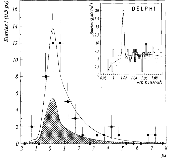
Fig. 9. Measured proper time distribution of \phi - l events. The curve is the result of the likelihood fit. The shaded area corresponds to the background distribution. In the inset is plotted the invariant mass distribution of the \phi candidates used for the lifetime measurement. The curve is the result of the fit of the mass spectrum using a Gaussian distribution for the signal and the same parametrization for the background as in Fig. 2
