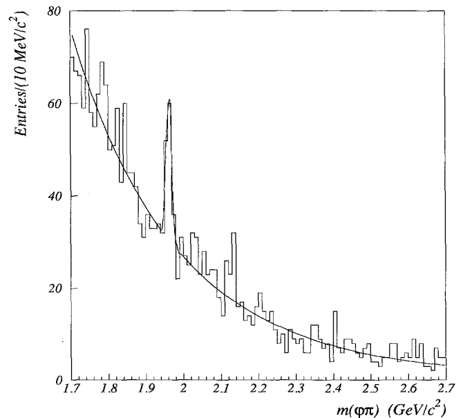
Fig. 3. Invariant mass distribution of the \phi\pi candidates. The curve shows the result of a fit with a Gaussian and a term for the background. The latter has been parametrized with the exponential of a second order polynomial
