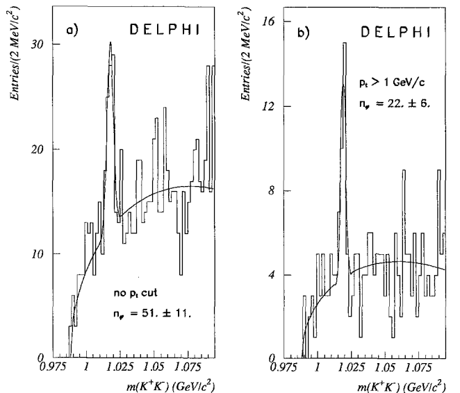
Fig. 6a, b. \phi meson signal in events accompanied by a muon in the same jet: a with no muon transverse momentum cut, and b with a muon transverse momentum greater than 1 GeV/c. The curves are the result of the fit of the mass spectrum using a Gaussian distribution for the signal and the same parametrization for the background as in Fig. 2
