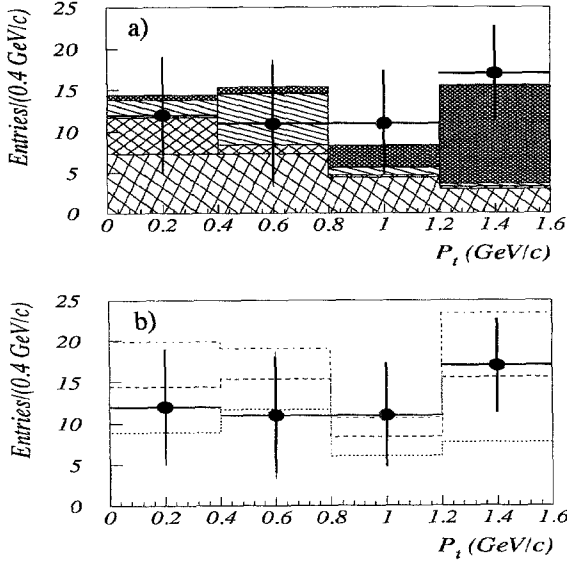
Fig. 8a, b. Transverse momentum distribution of the muon in \phi - \mu events. The last bin contains all events with p_t^\mu greater than 1.2 GeV/c. a Data (points with error bars) and contributions from (i) fake muons (cross-hatched), (ii) direct muons from D mesons (dense cross-hatched), (iii) cascade muons (diagonal hatched) and (iv) direct muons from B^0 mesons (dark-hatched). b Data compared with expectations for different values of f_s^w : (i) 0.2 (the fit result - dashed), (ii) 0.0 (dotted), and (iii) 0.4 (dash-dotted)
