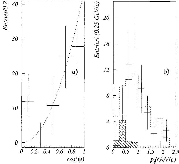
Fig. 4. a |\cos(\psi)| distribution for the events selected in the D_s signal region after combinatorial background subtraction. b Transverse momentum distribution of the selected D_s candidates. The Monte Carlo predictions for D_s meson production for b\bar{b} and c\bar{c} events are shown as dotted and hatched histograms respectively
