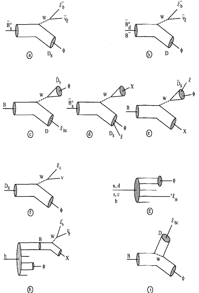
Fig. 7a-i. Processes contributing to the production of \phi - \mu events with the \phi and the muon appearing in the same jet. When several mechanisms of the same type contribute to a given process, only the dominant diagram has been displayed.
