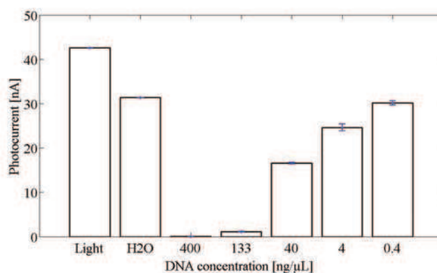
Fig. 8. Detection of different DNA concentrations ( Escherichia coli ) in the quartz cuvettes: Light and \text{H}_2\text{O} concentrations were used as references
