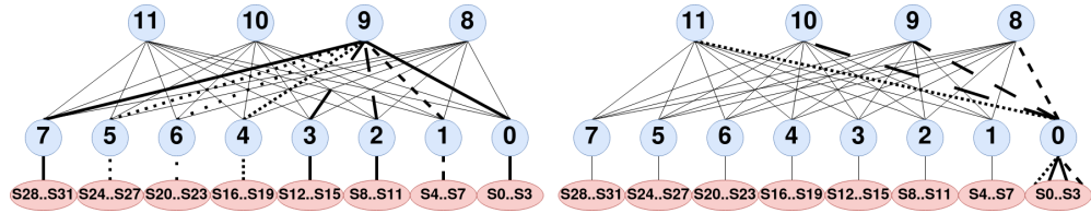
Fig. B1: Illustration of the deterministic nature of the paths in a two-layer fat-tree topology. On the left, all servers have one unique path to join spine 9 represented by different dashed lines. On the right, all spine switches have one unique path to join servers 0..3.
