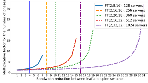
Fig. 7: Multiplicative factor for the number of phases as a function of the bandwidth reduction f between leaf and spine switches for several fat-tree topologies. FT(2;8,16) contains 128 servers, FT(2;16,16) contains 256 servers, FT(2;20,18), our use-case DAQ network, contains 360 servers, FT(2;16,32) contains 512 servers and FT(2;32,32) contains 1024 servers. The vertical lines correspond to the loss of half the bandwidth for each topology.
