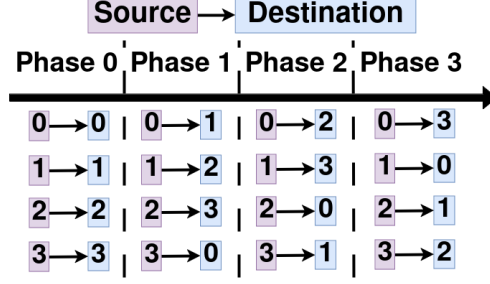
Fig. 1: The Linear-shift scheduling with 4 processes. Each process communicates with all other processes. To prevent congestion, the exchange is divided into 4 phases. In each phase, each process sends data to another process and receives data from another one. The minimum number of phases for the all-to-all exchange is the same as the number of processes.
