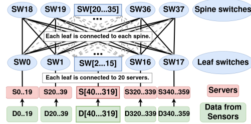
Fig. 2: The fat-tree topology of the studied DAQ Network. The notation of the fat-tree topology is FT(L = 2; M_0 = 20, M_1 = 18) , where L defines the number of layers, M_0 is the number of spine switches and M_1 is the number of leaf switches. The number of servers is M_0 * M_1 = 360 .
