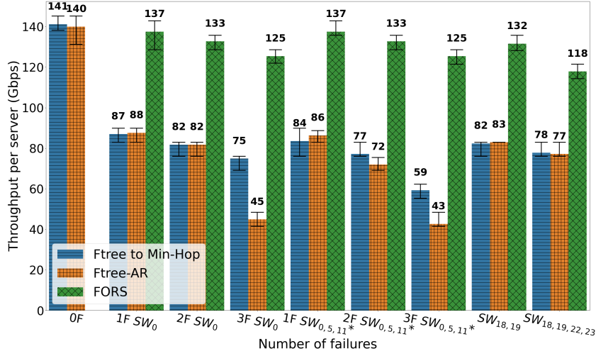
Fig. 6: Evaluation of FORS throughput compared to the default routing algorithms Ftree/Min-Hop and the adaptive routing version of Ftree. To obtain the total throughput achieved by the DAQ application, one can multiply the throughput per server by the number of servers in the DAQ application, which is 326. The error bars represent the minimum, mean and maximum values over one minute of measurement. The fat-tree topology of the studied data acquisition network is FT(2;20,18), illustrated in Figure 2. The failure scenarios noted with "*" are the ones where an ILP model was needed to compute the routing solution.
