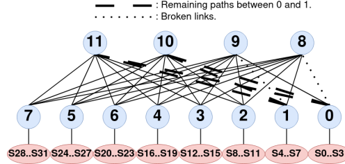
Fig. 5: Illustration of a failure scenario on a two-layer fat-tree topology involving an unequal number of paths between different leaf switches. The links 0-8 and 1-9 are broken, resulting in switch 0 having only 2 paths available to switch 1 and 3 paths available to the rest of the leaf switches.
