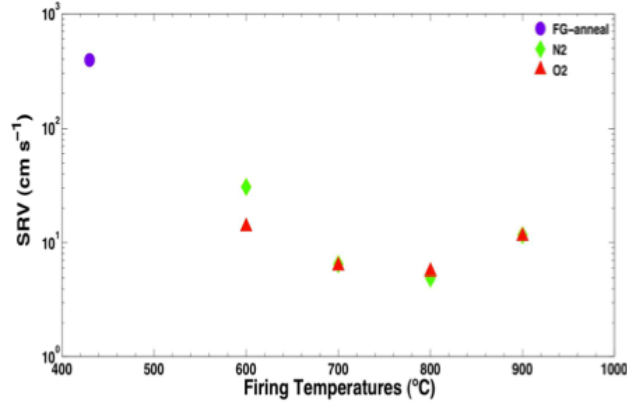
Fig 3.1(c): Estimated effective SRV values as function of firing temperatures at \Delta n = 2 \times 10^{15} \text{ cm}^{-3} for both atmospheric (N 2 and O 2 ) conditions.
