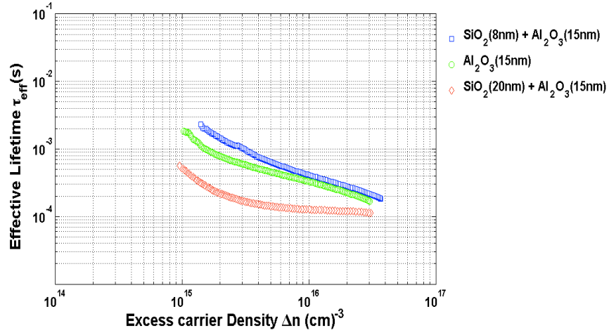
Figure 2.5: Injection-dependent effective minority carrier lifetime measurements on \text{Al}_2\text{O}_3/\text{SiO}_2 stacks
