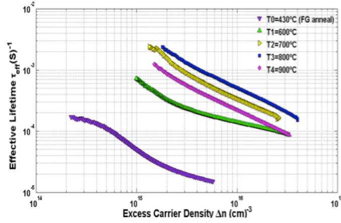
Fig 3.1(a): Injection dependent minority carrier lifetime measurements on the samples that underwent firing in N_2 atmosphere.
