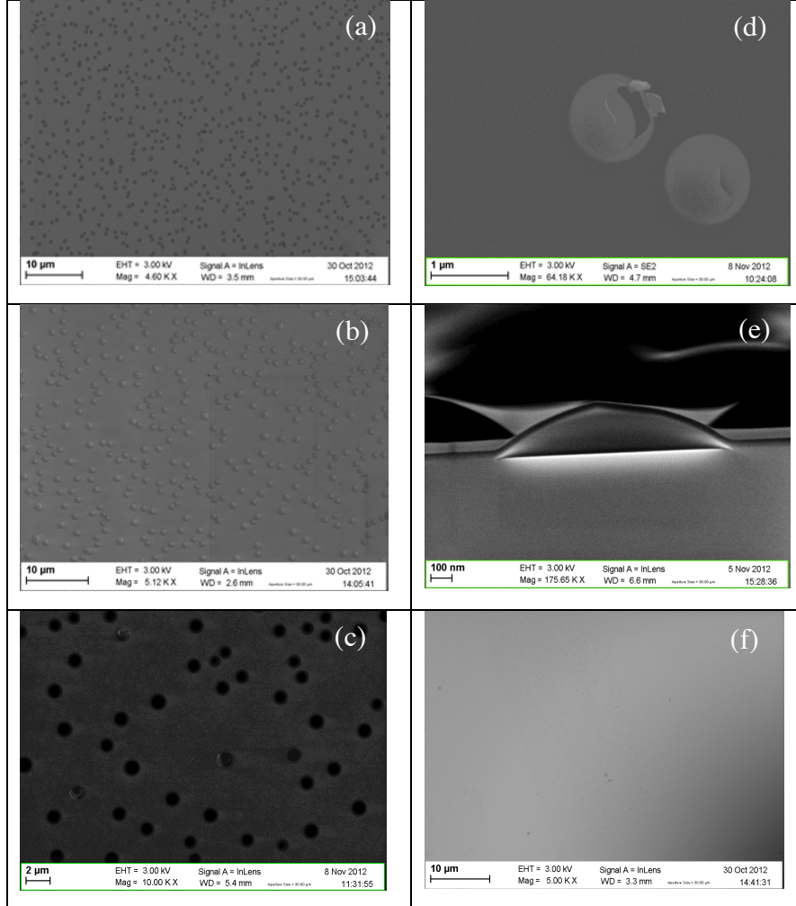
Fig 3.3: Scanning Electron Microscopy (SEM) images of the \text{Al}_2\text{O}_3 films fired in \text{N}_2 and \text{O}_2 atmosphere: Fired at (a) 700°- \text{N}_2 atmosphere (b) 800°- \text{N}_2 atmosphere (c) 900°- \text{N}_2 atmosphere (d) Delamination of \text{Al}_2\text{O}_3 film from the silicon surface when fired at 900°- \text{N}_2 atmosphere (e) Cross-sectional view of the blister (f) fired at 900°C- \text{O}_2 atmosphere.
