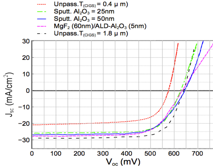
Figure 5.2: J-V characteristics of the unpassivated (0.4 \mu\text{m} , 1.8 \mu\text{m} ) and (MgF 2 /) Al 2 O 3 rear surface passivated Cu(In, Ga) Se 2 solar cells [taken from ref 95]
