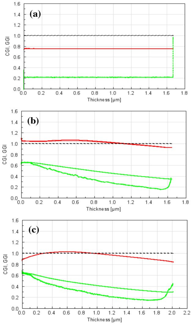
Elemental depth profiling (CGI and GGI) in the target material for (a) UG, (b) BSG and (c) DSG CIGS solar cells
