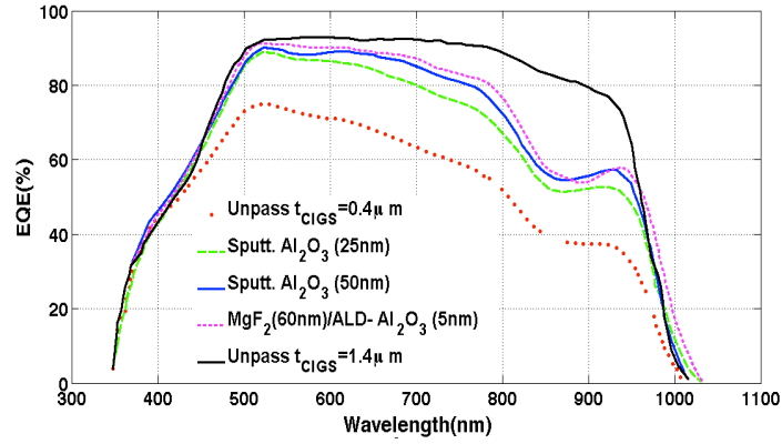
Figure 5.4: External Quantum efficiency measurements for unpassivated reference cells and passivated ( MgF_2 )/ Al_2O_3 rear surface passivated CIGS solar cells (Courtesy of B. Vermang and Universität Uppsala [95])
