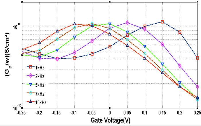
Fig 2.3.3: D_{it} extraction using conductance method: the maximum energy loss due to trapping/de-trapping mechanism at the interface ( \text{SiO}_2/\text{Si} ) were recorded by plotting parallel conductance ( G_p ) as a function of depletion gate voltage ( V_g ) for given frequency ( f )
