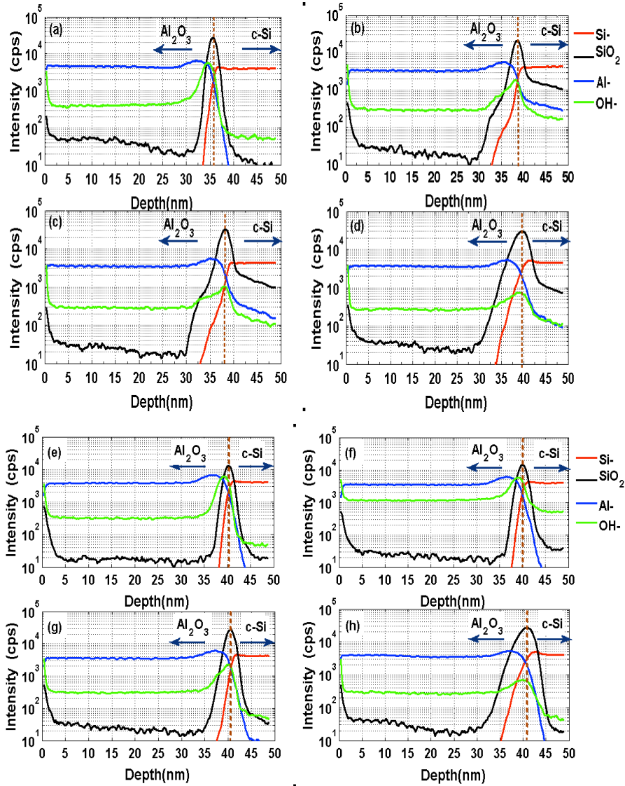
Figure 2.6.4 (a-h). The time of flight secondary Ion mass spectroscopy profiling of \text{Al}_2\text{O}_3 films depth fired at differed atmosphere and temperatures a. 600°- temperature and \text{N}_2 atmosphere (b) 700° temperature and \text{N}_2 atmosphere (c) 800° temperature and \text{N}_2 atmosphere (d) 900° temperature and \text{N}_2 atmosphere (e) 600° temperature and \text{O}_2 atmosphere (f) 700° temperature and \text{O}_2 atmosphere (g) 800° temperature and \text{O}_2 atmosphere (h) 900°- \text{O}_2 atmosphere.
