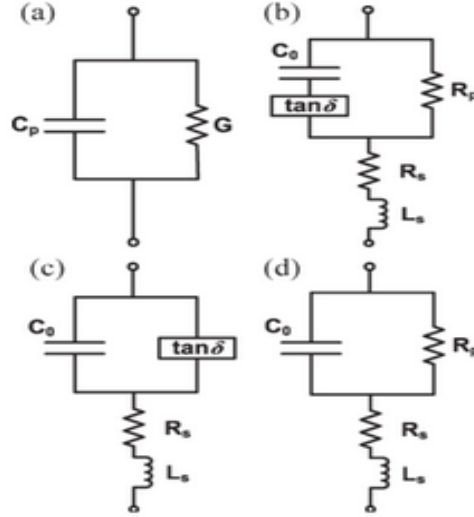
Small-signal equivalent circuit model of MOS capacitor (a) simple parallel circuit model (b) Five element model proposed by W.H.Wu et. al. (c) Four-element circuit model for low leakage high k -dielectrics (d) Four-element circuit model for ultra-thin and leaky k -dielectrics [taken from 101].
