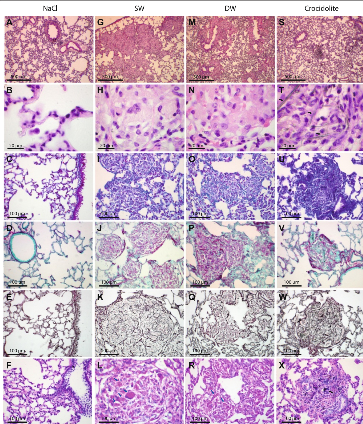
Figure 4 Ge-implolites induce a fibrotic lung response. Wistar rats were intra-tracheally instilled with NaCl (controls), 2 mg crocidolite, 1 mg SW and DW Ge-implolites. Lung histology was examined 60 d after exposure. (A-F) NaCl, (G-L) SW Ge-implolites, (M-R) DW Ge-implolites and (S-X) crocidolite. Sections stained with H&E (A-B, G-H, M-N, S-T), Trichrome blue (C, I, O, U), Sirius Red (D, J, P, V), reticulin (E, K, Q, W), PAS (F, L, R, X). Black and blue arrows indicate asbestos fibres and glycoprotein-rich areas, respectively.
