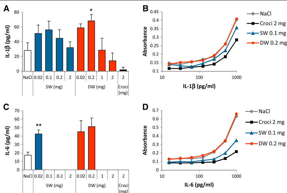
Figure 2 Ge-imogolites induce inflammatory cytokine secretion in rat alveoli 3 d after intra-tracheal instillation. Wistar rats were intra-tracheally instilled with NaCl (controls), 2 mg crocidolite, 0.02 to 2 mg SW and DW Ge-imogolites. Inflammatory cytokines were quantified by ELISA in the BALF after 3 d. BALF (A) IL-1 \beta and (C) IL-6. (B) IL-1 \beta and (D) IL-6 curves obtained from cytokine standards diluted with BALF from NaCl, 2 mg crocidolite, 0.1 mg SW and 0.2 mg DW Ge-imogolite-exposed rats. * P < 0.05 and ** P < 0.01 relative to control rats (Dunnett multiple comparisons test between NaCl and Ge-imogolite-treated rats or t-test between NaCl and crocidolite-treated rats, n = 4 , means SEM).
