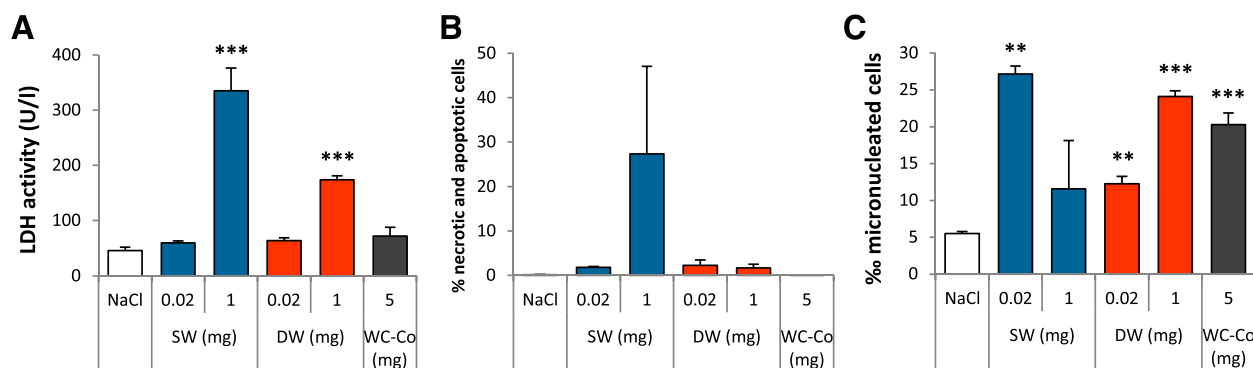
Figure 6 Ge-imogolites induce genotoxicity in rat lungs. Wistar rats were intra-tracheally instilled with NaCl (controls), 5 mg WC-Co, 0.02 and 1 mg SW and DW Ge-imogolites. Micronuclei were assessed in isolated AEC-II 3 d after exposure. (A) BALF LDH activity, (B) % of necrotic and apoptotic cells and (C) micronucleated cells. **P < 0.01 and ***P < 0.001 relative to control rats (Dunnett multiple comparisons test between NaCl and Ge-imogolite-treated rats or t-test between NaCl and WC-Co-treated rats, n = 3, means SEM).
