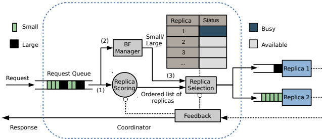
Fig. 6: Operating principle of Héron.
