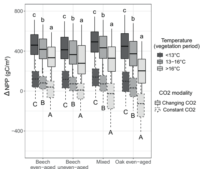
Fig. 5. Comparison of the simulated change in annual NPP in virtual sites between historical period (1976–2005) and RCP8.5 scenario (2071–2100) for the two atmospheric \text{CO}_2 modalities: highlighting of the stand type effect as well as the effects of the air temperature during the vegetation period. For each box, the horizontal line corresponds to the median, the ends indicate the 25th and 75th percentiles and the whiskers show the values above and below these quartiles within 1.5 interquartile. For a same stand type, temperatures during vegetation period with common letters are not significantly different (paired Wilcoxon signed-rank).
