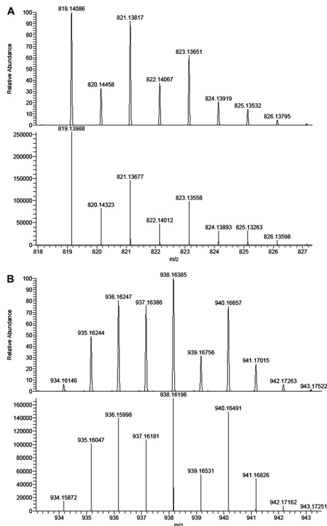
Fig. 5. Experimental (at the top) and theoretical (at the bottom) isotopic distribution of: part A: [\text{Zn}:\textbf{7a}] coordination complex (with atomic composition: \text{C}_{30}\text{H}_{46}\text{O}_{14}\text{N}_2\text{ClP}_2\text{Zn} ). Part B: [\text{Gd}:\textbf{7a}] coordination complex (with atomic composition: \text{C}_{30}\text{H}_{46}\text{O}_{16}\text{N}_4\text{GdP}_2 ).
