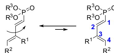
Fig. 1. s-trans / s-cis equilibrium of ( E )- 1 .
