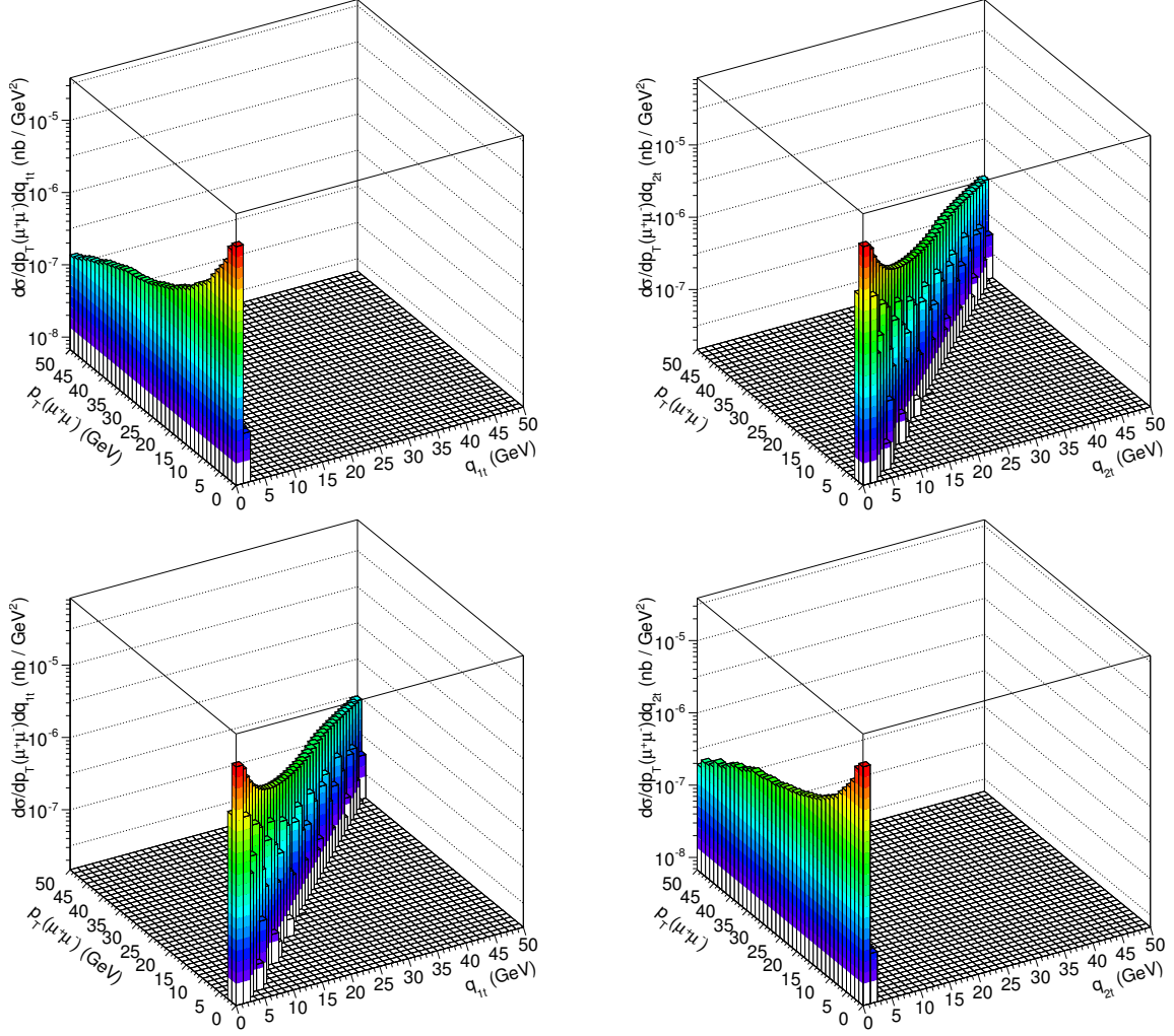
Figure 7. Two-dimensional distribution in p_{T,\text{sum}} and one of transverse momentum ( q_{1T} or q_{2T} ) of the virtual photon for elastic-inelastic (top row) and inelastic-elastic (bottom row) components at \sqrt{s} = 7 TeV. The additional cuts of p_T(\mu^\pm) < 50 GeV, |\eta(\mu^\pm)| < 2.5 , and M_X = [1.07, 1000.00] GeV are used.
