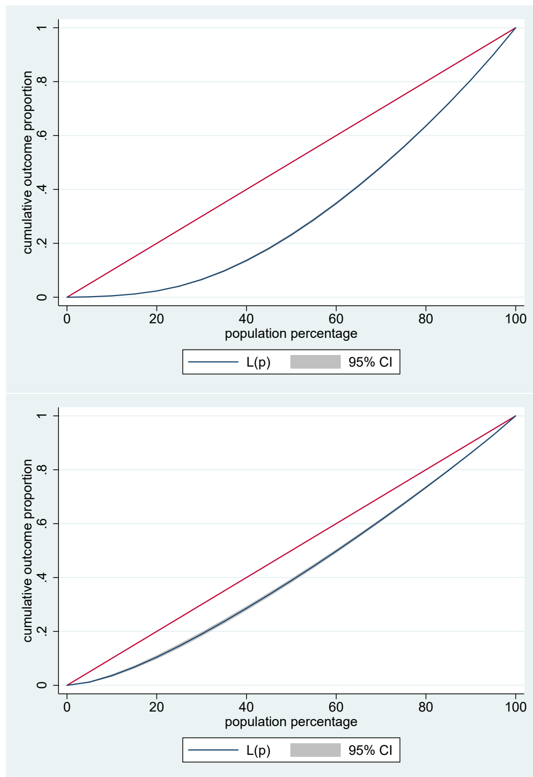
Figure B.3. Estimates of Lorenz curves (accumulated lifespan share by decile of the lifespan definition).
