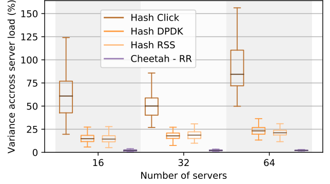
Figure 7: Variance among servers' load of various methods for an increasing number of servers. The average requests/s is 100 per server. CHEETAH, though stateless, allows a near-perfect load spreading.
