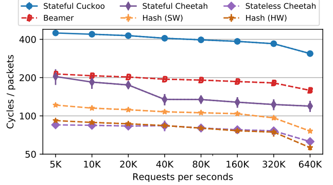
Figure 5: CPU cycles/packets for various methods. CHEETAH achieves the same load balancing performance as stateful LBs with 5x fewer cycles and only a minor penalty over hashing.
