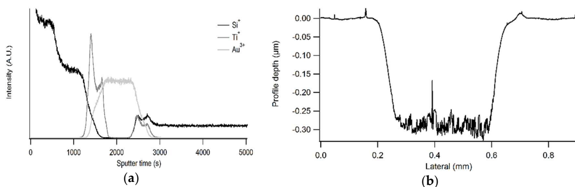
Figure 8. Complete profile of Si model sample b obtained with SIMS (a). Profilometry analysis (b) was conducted on a fresh zone and sputtering was stopped when the Ti signal reached half of the maximal intensity.
