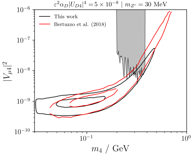
FIG. 18. A comparison of the LEE neutrino energy spectrum fit in this work and that of Ref. [36] for the choice of m_{Z'} = 30 MeV. The 1\sigma and 2\sigma regions are shown as smaller and larger closed regions, respectively. We assume that the results in Ref. [36] are quoted for |U_{D4}|^2 = 1 .
