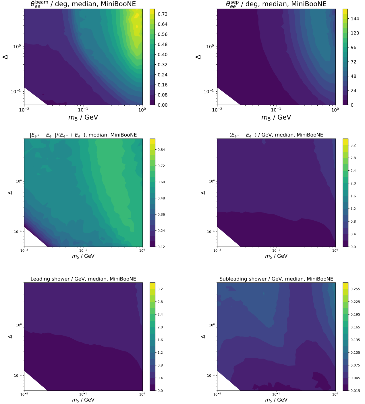
FIG. 20. The median of kinematical variables in dark neutrino events at MiniBooNE for the 3+2 model with m_{Z'} = 1.25 \text{ GeV} . We show the median of (1) the angle between the shower and beam, (2) the angle between the two showers, (3) the asymmetry of the showers, (4) the total energy of the showers, and the energy of the leading (5) and subleading (6) showers.
