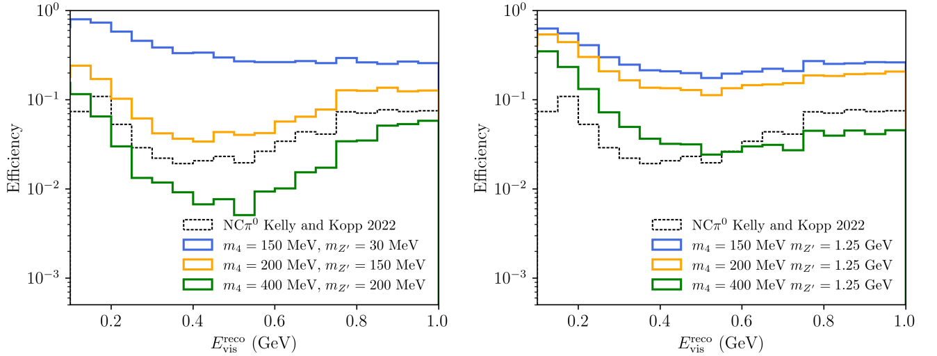
FIG. 15. A comparison between the pre-selection (circ1) efficiency for dark neutrino events and the misidentification probability for \pi^0 background events (from [8]) in the reconstructed visible energy variable.
