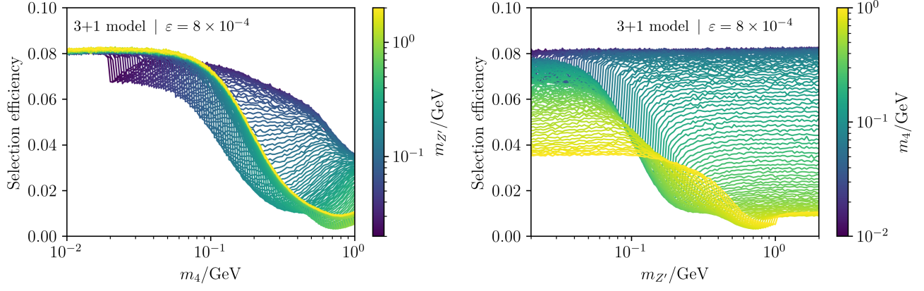
FIG. 16. The signal selection efficiency of our simulation for dark neutrino events in MiniBooNE for the 3+1 model. On the left, we show the efficiency as a function of the heavy neutrino mass m_4 for fixed values of the mediator mass, m_{Z'} . On the right, we show the same efficiency, now as a function of m_{Z'} for fixed values of m_4 . The geometric acceptance is not included.
