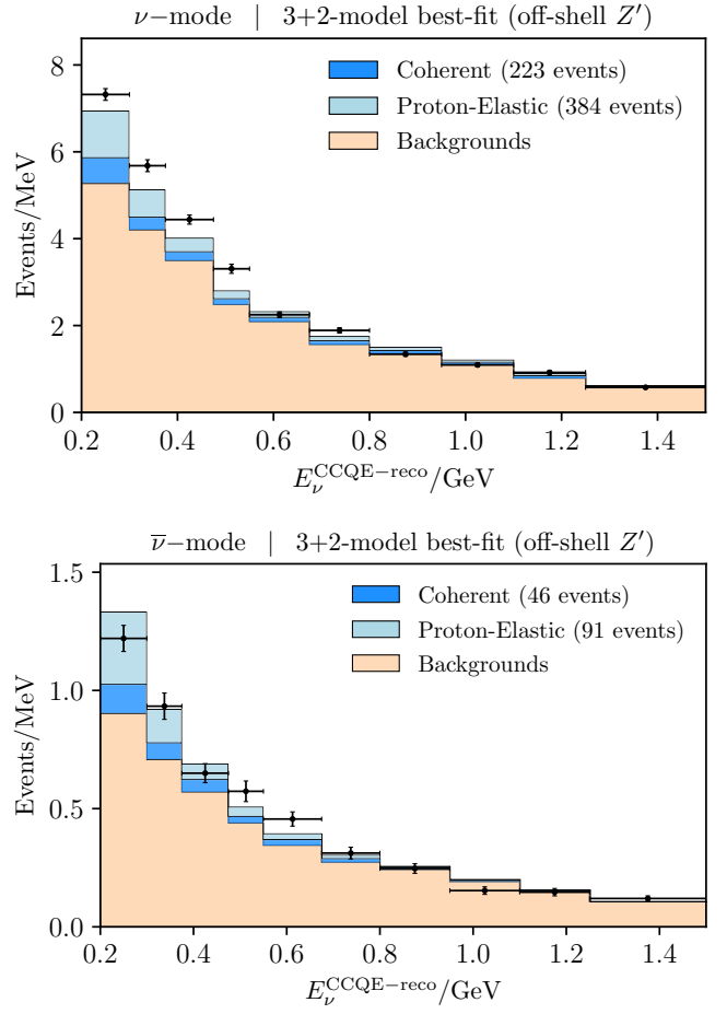
FIG. 9. The reconstructed neutrino energy E_{\nu}^{\text{CCQE-reco}} at MiniBooNE for \nu mode (upper panel) and \bar{\nu} mode (lower panel). The prediction of the best-fit point in the 3+2-model ( m_{Z'} = 100 MeV, m_5 = 615 MeV, \Delta = 0.3 , |V_{\mu 4}|^2 = |V_{\mu 5}|^2 = 1.1 \times 10^{-6} , \varepsilon = 8 \times 10^{-4} ) is shown as solid blue histograms, separated into events from coherent neutrino-nucleus scattering and proton-elastic neutrino scattering.
