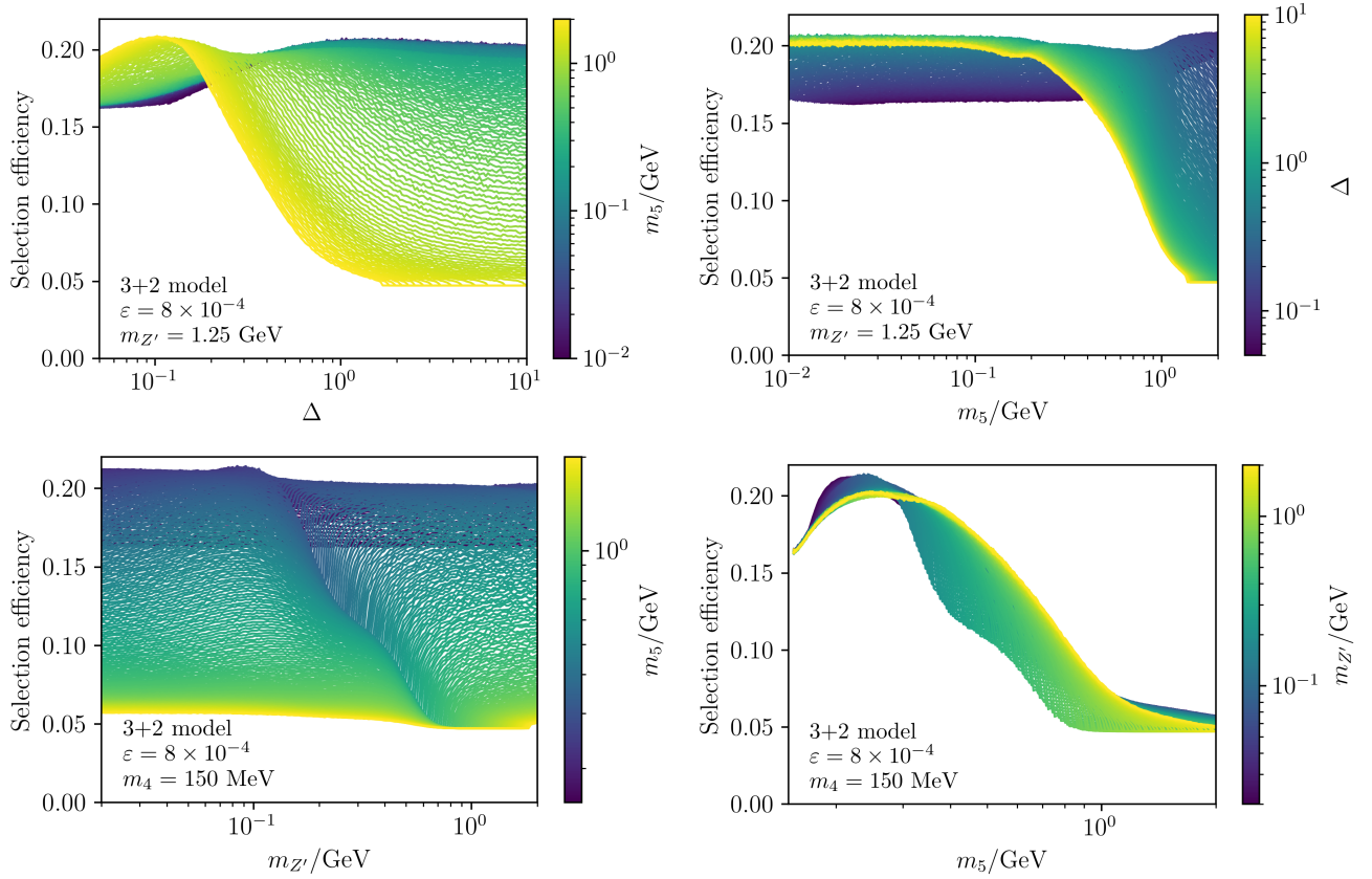
FIG. 17. The signal selection efficiency of our simulation for dark neutrino events in MiniBooNE for the 3+2 model. The upper panels show the efficiency as a function of the HNL mass splitting \Delta (left) and the parent HNL mass m_5 (right) for a single fixed value of m_{Z'} . The lower panels show the efficiency as a function of the mediator mass m_{Z'} (left) and the parent HNL mass m_5 (right) for a single fixed value of m_4 . The geometric acceptance is not included.
