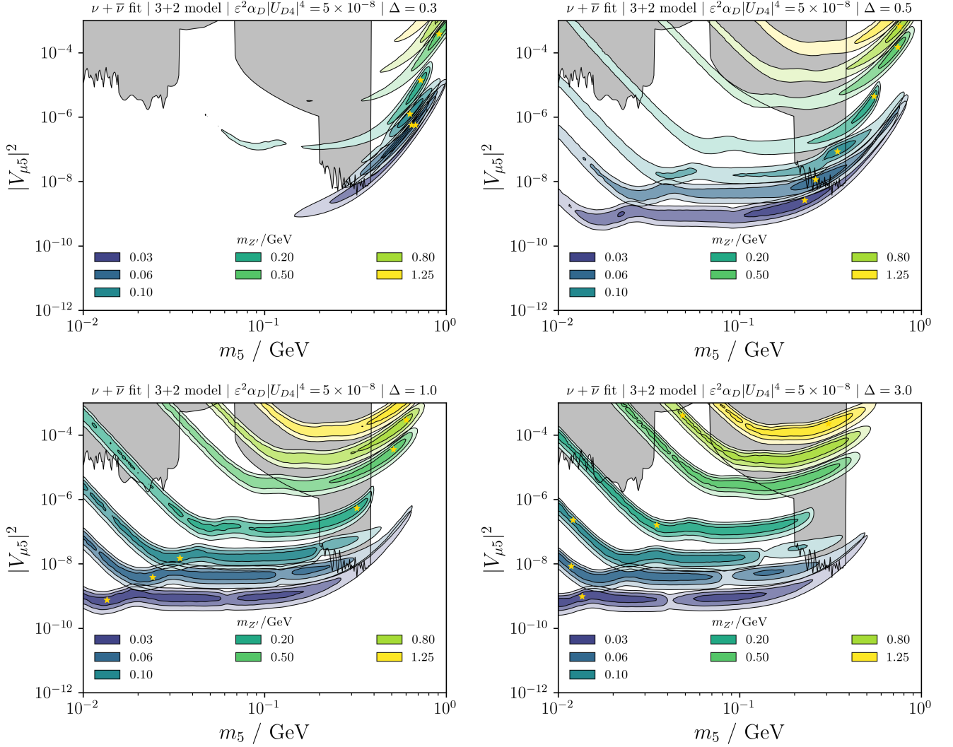
FIG. 7. The MiniBooNE E_\nu^{\text{CCQE-reco}} best-fit regions in the |V_{\mu 5}|^2 and m_5 plane for the 3+2 model. Each panel corresponds to a different value of \Delta , as indicated at the top of the panel. Each color represents a given fixed value of m_{Z'} , and the different shading corresponds to the 1\sigma , 2\sigma , and 3\sigma CL regions (2 d.o.f.). Model-independent limits on heavy neutrinos exclude the shadowed region [209]. Other constraints from neutrino scattering and meson decays are not shown.
