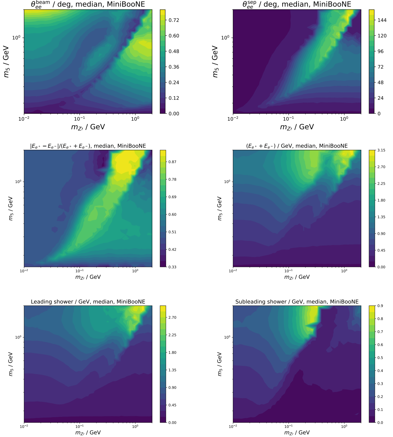
FIG. 21. The median of kinematical variables in dark neutrino events at MiniBooNE. We show the median of (1) the angle between the shower and beam, (2) the angle between the two showers, (3) the asymmetry of the showers, (4) the total energy of the showers, and the energy of the leading (5) and subleading (6) showers. We fix m_4 = 150 MeV and \epsilon = 0.01 .
