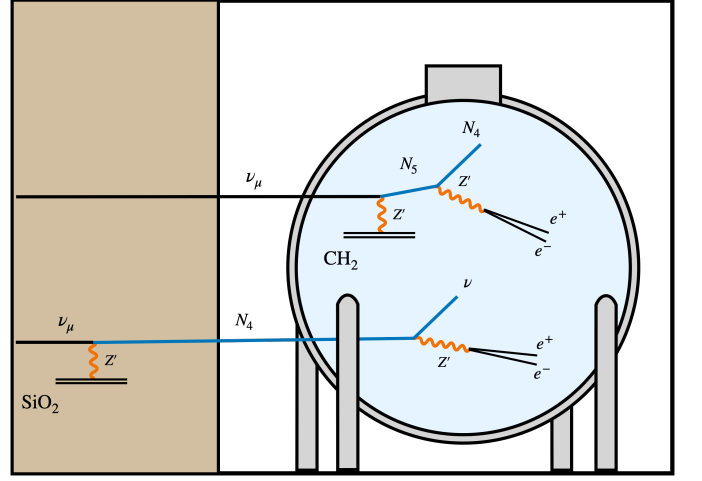
FIG. 2. The dark neutrino upscattering signature at MiniBooNE for 3+1 models ( N_4 \rightarrow \nu e^+ e^- ) and 3+2 models ( N_5 \rightarrow N_4 e^+ e^- ). As an example, we show a scattering inside the detector for 3+2 and in the dirt upstream of the detector for 3+1.
