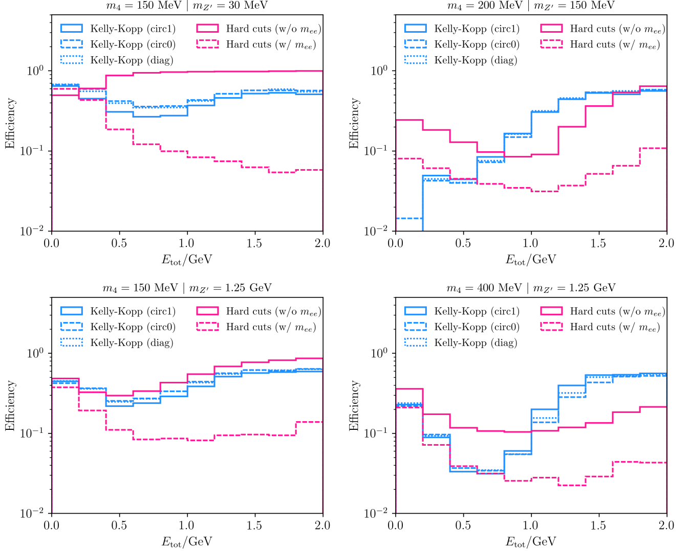
FIG. 13. The final signal efficiency using different pre-selection methods. The true-variable method, discussed in Appendix A 0 a, is shown with and without applying the cut on the e^+e^- invariant mass m_{ee} . The simplified \pi^0 method, discussed in Appendix A 0 b, is referred to as Kelly-Kopp. We show the different methods based on the choice of the r variable, as defined in [8]. In all cases, we generate upscattering inside the detector and enforce N_4 to decay promptly. The fits in the main text are based on the Kelly-Kopp (circ1) method.
