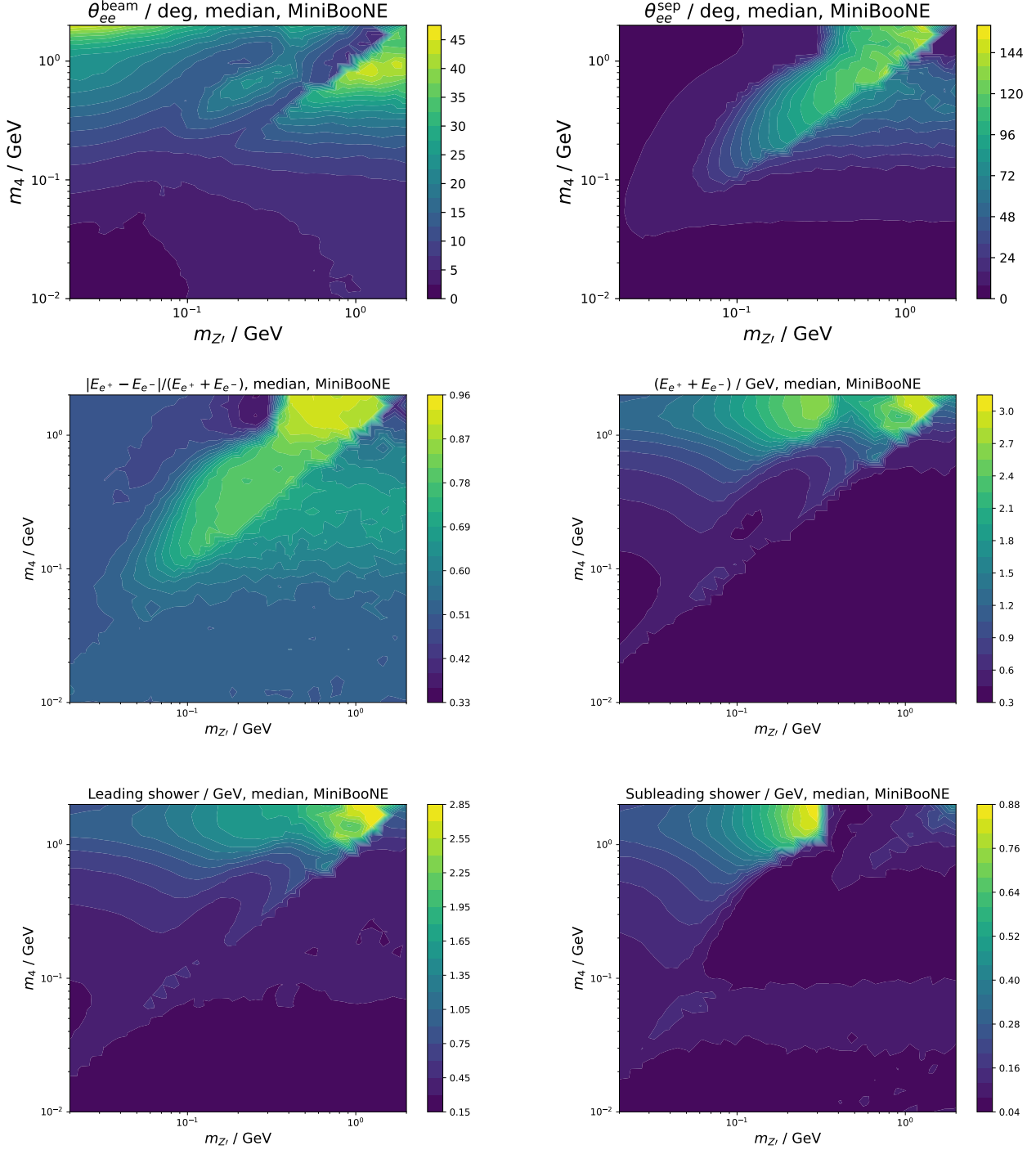
FIG. 19. The median of kinematical variables in dark neutrino events at MiniBooNE for the 3+1 model. We show the median of (1) the angle between the shower and beam, (2) the angle between the two showers, (3) the asymmetry of the showers, (4) the total energy of the showers, and the energy of the leading (5) and subleading (6) showers.
