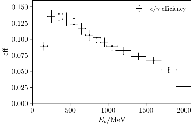
FIG. 12. MiniBooNE single electron/photon efficiencies as a function of energy [207] used in this work.
