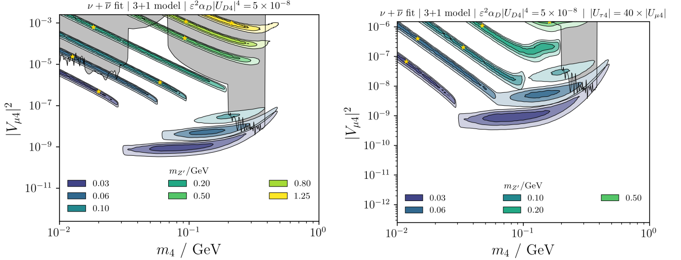
FIG. 3. The MiniBooNE E_\nu^{\text{CCQE-reco}} best-fit regions in the |V_{\mu 4}|^2 and m_4 plane for the 3+1 model. On the left, we set |U_{\tau 4}| = 0 , and on the right |U_{\tau 4}| = 40|U_{\mu 4}| . Each color represents a given fixed value of m_{Z'} , and the different shading corresponds to the 1\sigma , 2\sigma , and 3\sigma CL regions (2 d.o.f.). Model-independent limits on heavy neutrinos exclude the shadowed region [209]. Other constraints from neutrino scattering and meson decays are not shown.
