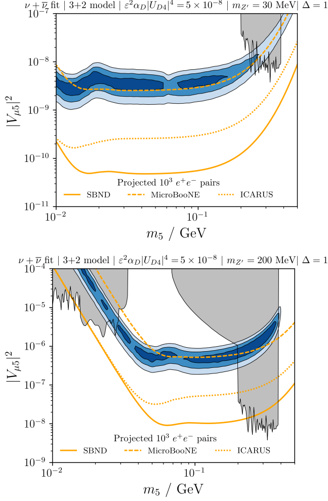
FIG. 8. Same as Fig. 7 but for m_{Z'} = 30 MeV (upper) and m_{Z'} = 200 MeV (lower). The mass splitting has been fixed to \Delta = 1 . The orange lines indicate where the MicroBooNE (dashed), ICARUS (dotted), and SBND (solid) detectors can expect 10^3 e^+ e^- pairs from N_5 decays to be produced inside their respective fiducial volumes (before any reconstruction efficiencies).
