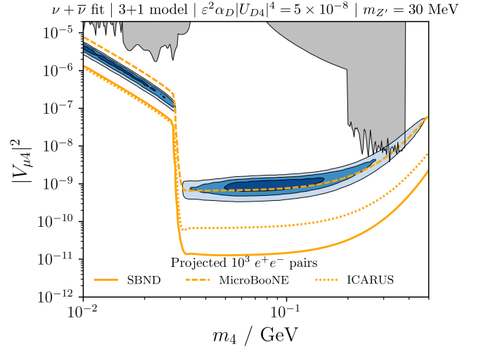
FIG. 5. Same as Fig. 3 showing only the case where m_{Z'} = 30 MeV and |U_{\tau 4}| = 0 . The orange lines indicate where the MicroBooNE (dashed), Icarus (dotted), and SBND (solid) detectors can expect 10^3 e^+e^- pairs from N_5 decays to be produced inside their respective fiducial volumes (before any reconstruction efficiencies).
