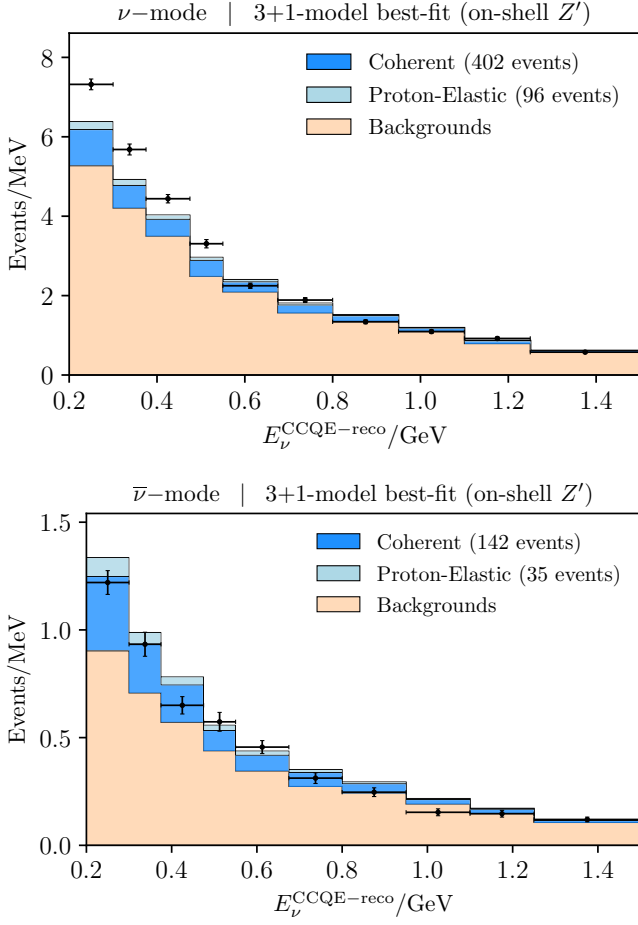
FIG. 4. The reconstructed neutrino energy E_{\nu}^{\text{CCQE-reco}} at MiniBooNE for the FHC ( \nu ) mode (upper panel) and the RHC ( \bar{\nu} ) mode (lower panel). The prediction of the best-fit point in the 3+1-model ( |V_{\mu 4}|^2 = 4.8 \times 10^{-7} , m_4 = 20 MeV, m_{Z'} = 30 MeV) is shown as a solid blue histogram, separated into events from coherent neutrino-nucleus scattering and proton-elastic neutrino scattering.
