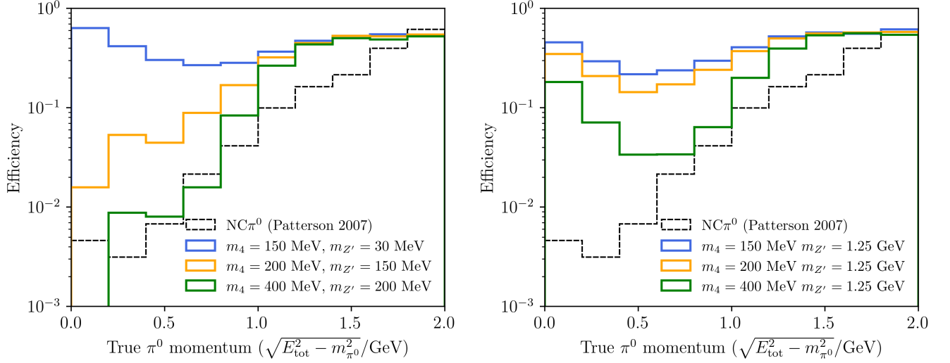
FIG. 14. A comparison between the MiniBooNE signal selection efficiency for dark neutrino events and the misidentification probability for \pi^0 background events (from [215]) in the true \pi^0 momentum variable. The latter is defined as \sqrt{E_{\text{tot}}^2 - m_{\pi^0}^2} for e^+e^- events.
