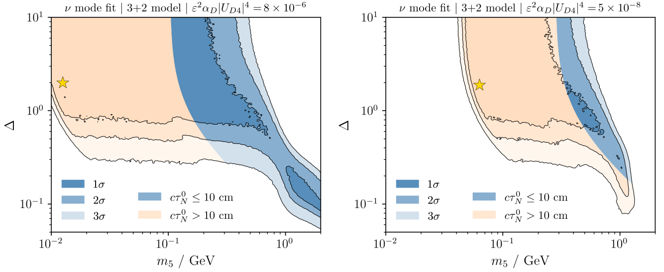
FIG. 10. The MiniBooNE E_\nu^{\text{CCQE-reco}} best-fit regions in the m_5 and \Delta plane for the 3+2 model for two choices of couplings. The different regions show the 1\sigma , 2\sigma , and 3\sigma best-fit regions. The couplings |U_{\mu 4}|^2 = |U_{\mu 5}|^2 are profiled over with an upper bound of |U_{\mu 4}|^2 < 10^{-2} , which can be tightened by choosing larger dark couplings and kinetic mixing. All the plots consider m_{Z'} = 1.25 GeV and couplings as indicated at the top of each panel. We divide the regions into a short-lived and a long-lived regime, where the HNLs decay rapidly, c\tau_N^0 \leq 10 cm, and a region where dirt events and displaced vertices are expected, c\tau_N^0 > 10 cm, where c\tau_N^0 is the HNL proper lifetime.
