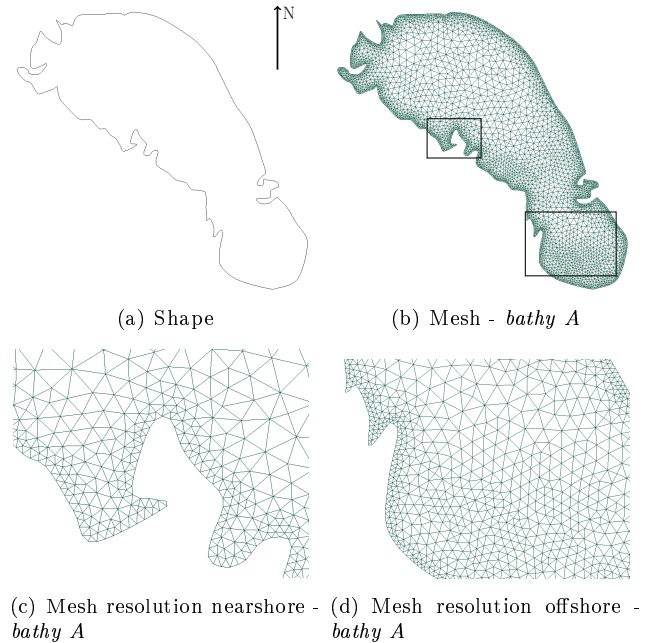
Figure 3: Discretization of Ontario Lacus using mesh-generation package GMSH: the coastline (Panel (a)) and the mesh used for bathy A (Panel (b)). Panel (c) shows the higher spatial resolution nearshore. Panel (d) shows the refinement in shallow regions in bathy A
