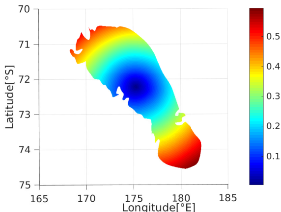
Figure 15: Lake surface elevation range in Ontario Lacus with a southerly wind of 1 \text{ ms}^{-1} blowing during 1 TD . It is higher in the south (due to the higher contribution of the constant term): the maximum lake surface elevation range is 0.593 \text{ m}
