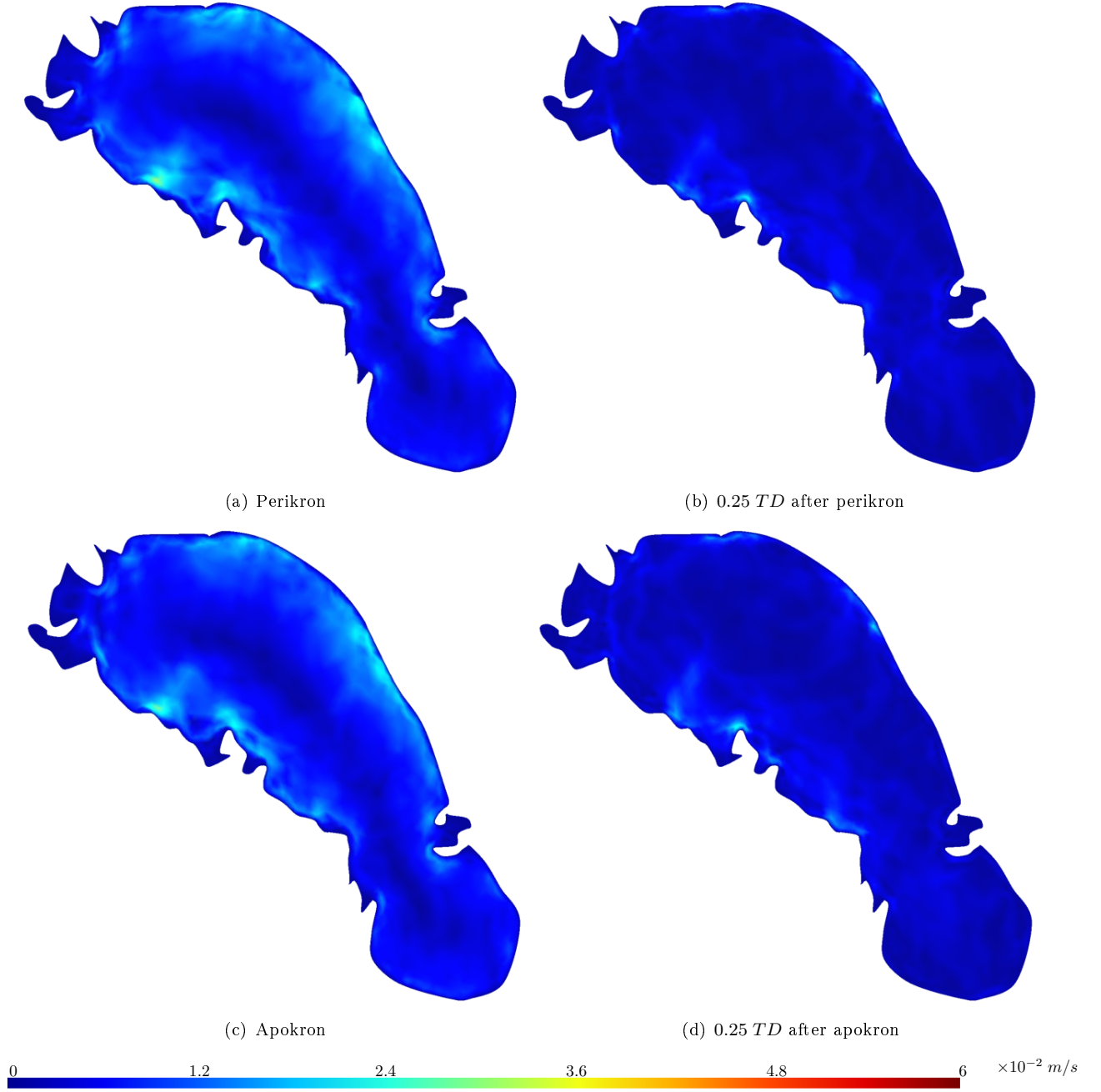
Figure 7: Tidal current magnitude (in \text{ms}^{-1} ) in Ontario Lacus at (a) Perikron, (b) 0.25 TD after Perikron, (c) Apokron and (d) 0.25 TD after Apokron with bathy C implemented. The current magnitude is maximum nearshore, at areas P or Q (see Fig. 1), depending on the time, and decreases with the distance to the shore. Globally, the speed is higher at perikron and apokron than 0.25 TD after perikron and apokron
