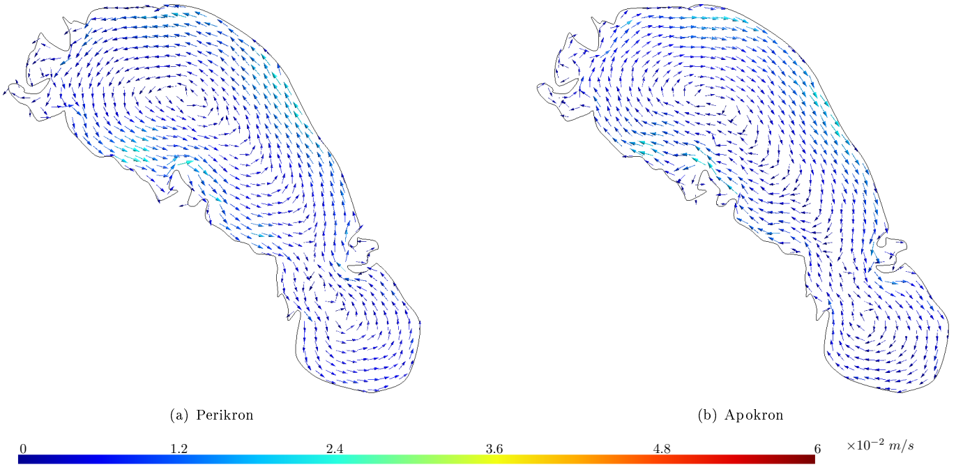
Figure 8: Tidal current orientation in Ontario Lacus at (a) Perikron, and (b) Apokron with bathy C implemented (the flow is interpolated on a structured grid in order to increase the quality of the figure). The flow forms a closed loop which rotates anticlockwise at perikron and clockwise at apokron
