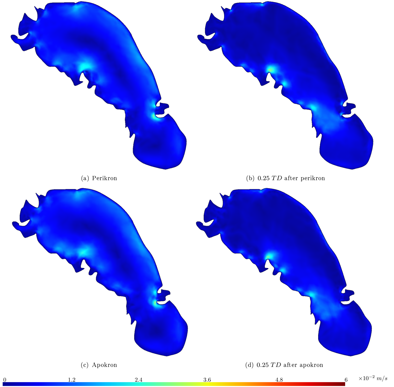
Figure 11: Tidal current magnitude (in ms^{-1} ) in Ontario Lacus with bathy B implemented at (a) Perikron, (b) 0.25 TD after Perikron, (c) Apokron and (d) 0.25 TD after Apokron. The current magnitude is maximum nearshore, at area E, and is significantly large at area G
