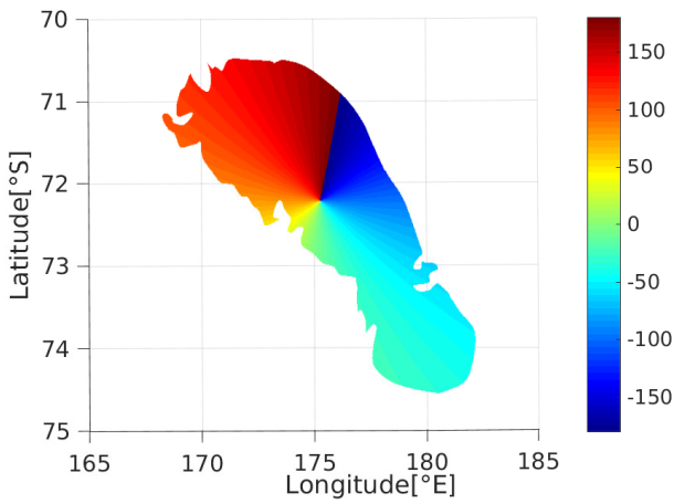
(b) Tidal phase of the main component (in degrees)
