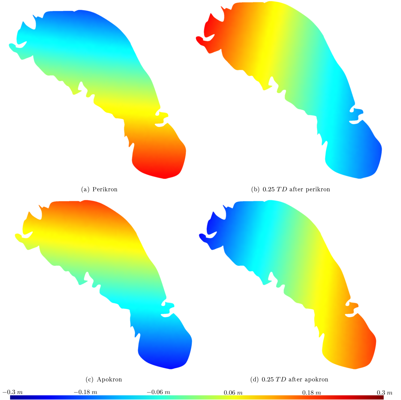
Figure 6: Surface elevation (in meters) in Ontario Lacus at (a) Perikron, (b) 0.25 TD after Perikron, (c) Apokron and (d) 0.25 TD after Apokron with bathy C implemented. The tide is high in the southern part at perikron and rotates clockwise with an exact period of 1 Titan day. The maximum/minimum surface elevation respectively occurs 0.11 TD before perikron/apokron, in the south
