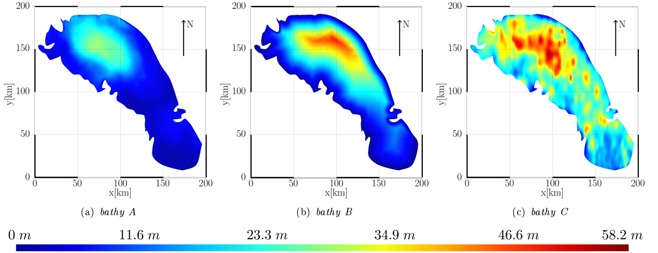
Figure 2: Bathymetries of Ontario Lacus (in meters). Panel (a) is the bathymetry computed by Ventura et al. (2012) from SAR data. The bathymetry is smoothed to be coherent with the bottom of dry lakes. bathy B is shown in Panel (b) and bathy C is shown in Panel (c). Except at the shore, bathy C is deeper and presents more pits than bathy A . bathy B is also deeper than bathy A and is more accurate nearshore than bathy C
