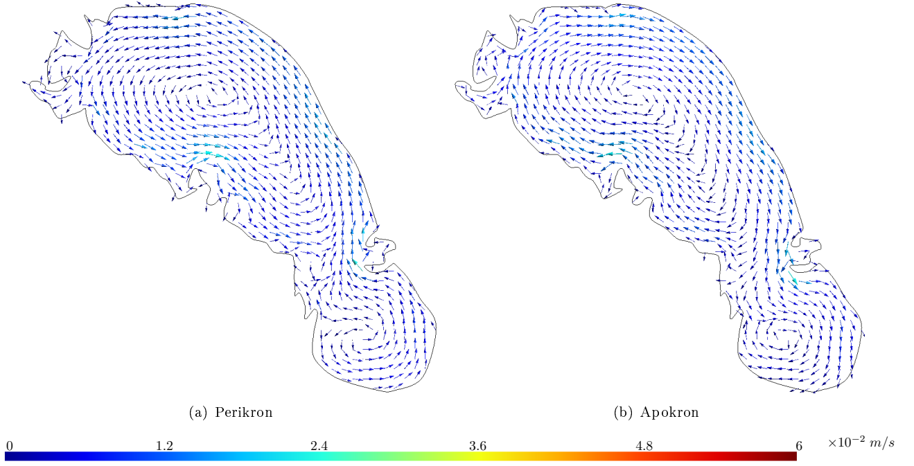
Figure 12: Tidal current orientation in Ontario Lacus with bathy B implemented at (a) Perikron and (b) Apokron (the current is interpolated on a structured grid in order to increase the quality of the figure). As with the other bathymetries, the flow forms a closed loop in the north. A southern closed loop also appears at perikron and apokron
