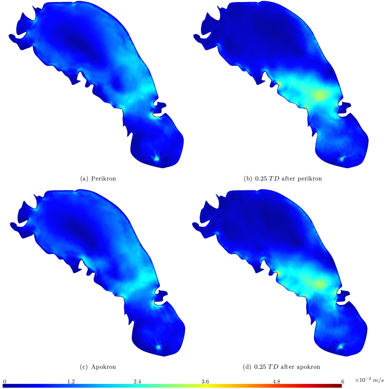
Figure 9: Tidal current magnitude (in m/s ) in Ontario Lacus with bathy A implemented at (a) Perikron, (b) 0.25 TD after Perikron, (c) Apokron and (d) 0.25 TD after Apokron. The current magnitude is maximum nearshore, at area 0 (see Fig. 1) and decreases with the distance to the shore except near area N and R where a wide offshore unidirectional high-speed area is predicted
