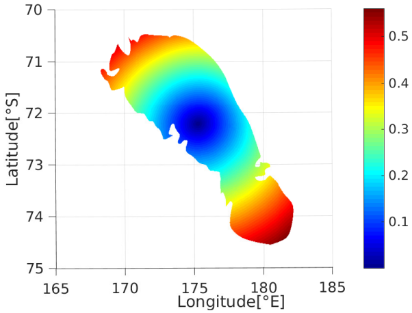
(a) Tidal range of the main component (in meters)
