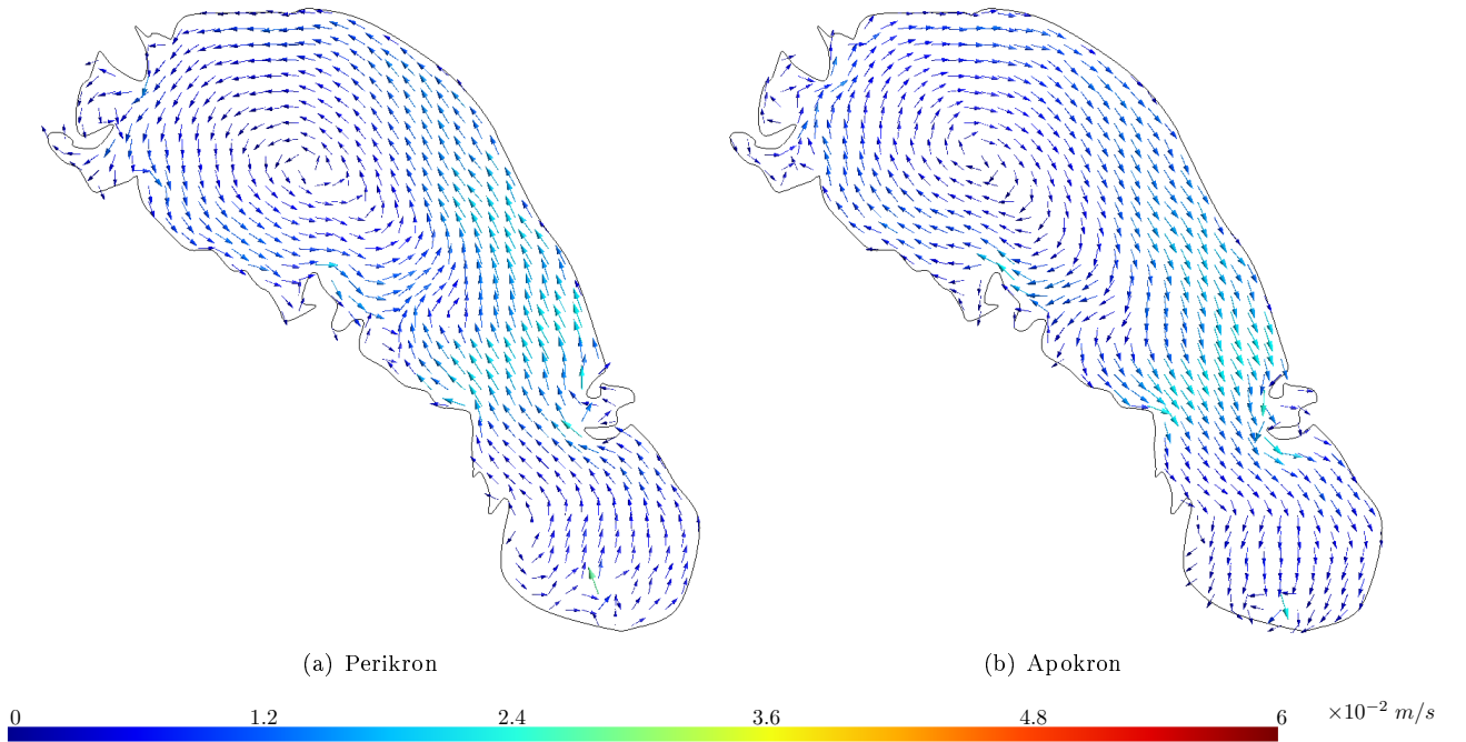
Figure 10: Tidal current orientation in Ontario Lacus with bathy A implemented at (a) Perikron and (b) Apokron (the flow is interpolated on a structured grid in order to increase the quality of the figure). As with bathy C , a closed loop is noticeable in the north. In the offshore high-speed area near point N and R (see Fig. 1), the current is unidirectional along the lake axis (it is northward at perikron and southward at apokron)
