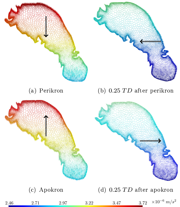
Figure 4: Instantaneous maps of the acceleration caused by Saturn in Ontario Lacus at four different times (perikron, 0.25 TD after perikron, apokron and 0.25 TD after apokron)(the black arrows represent the mean direction). It rotates clockwise with an exact period of 1 TD and it is maximum in the northern part of the lake
