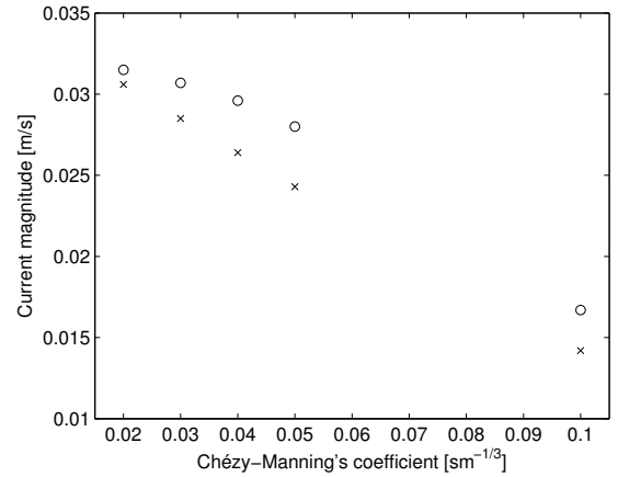
Figure 14: Evolution of maximum current speed with respect to the Manning's friction coefficient at two different times: perikron (circle) and apokron (cross). As expected, the flow decreases as the bottom friction increases
