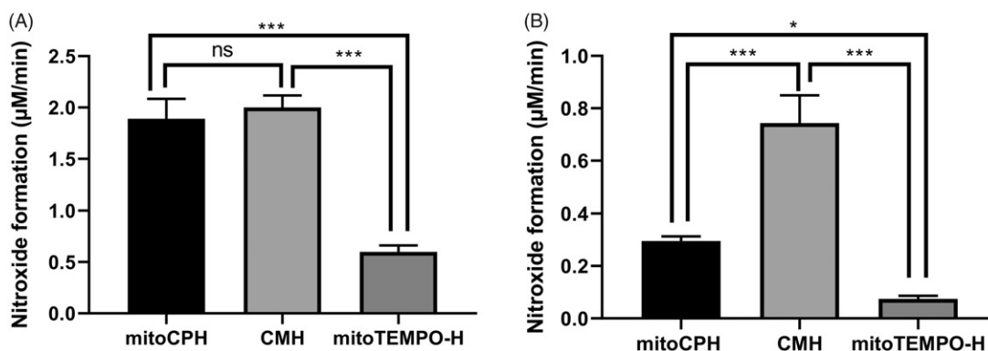
Figure 6. Comparison in trapping efficiency of the different cyclic hydroxylamines in PBS buffer (A) and in cell lysates (B). Rate of nitroxide apparition in 1 min for each probe. The generated superoxide flux was 1.97 μM/min. Superoxide was produced with HX 1 mM, DTPA 1 mM and XO 5 mU/mL ( n = 3 ). Concentrations of the probes were 0.5 mM. * p < .05 , *** p < .001 , ns p > .05 one-way ANOVA with Turkey test.
