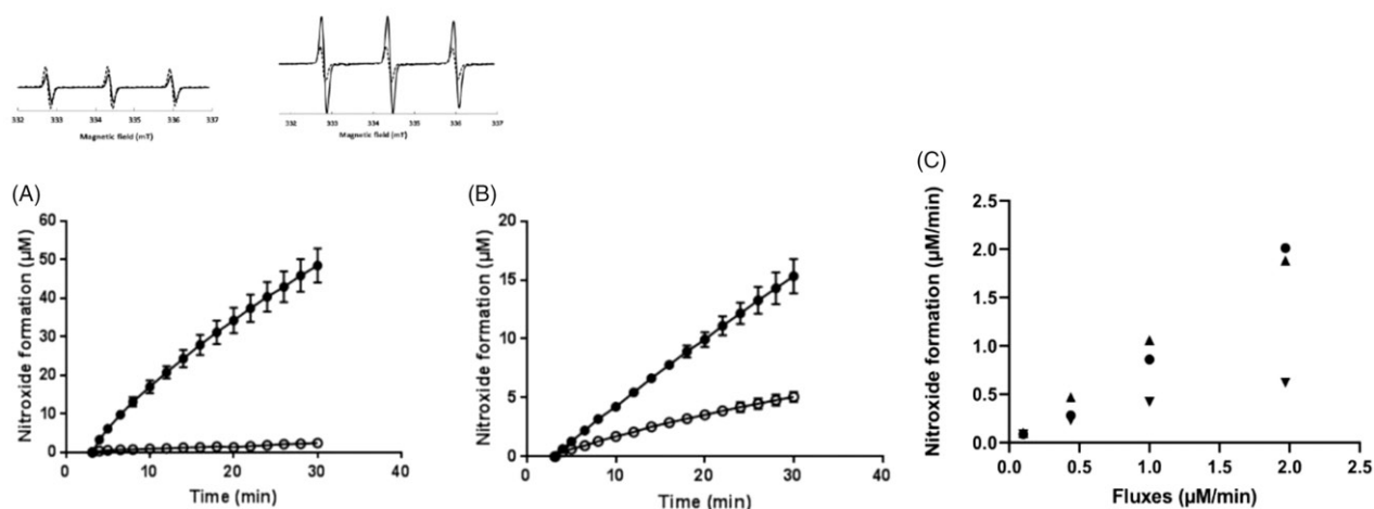
Figure 4. EPR monitoring of superoxide production in the presence of mitoCPH. Evolution of the EPR signal intensity over time in PBS buffer (A) and in cell lysates (B), in the absence (filled circle) or in the presence (open circles) of SOD (300 U/mL). Insert: EPR spectrum of mitoCPH in PBS after 10-min incubation in the presence of superoxide with (dashed line) or without SOD (black line). Superoxide was produced in PBS or cell lysates with HX 1 mM, DTPA 1 mM and XO 5 mU/mL. Concentration of the probe was 0.5 mM. (C) Nitroxides formation per minute at different superoxide generated fluxes (1.97, 1, 0.44 and 0.1 \mu\text{M}/\text{min} ) using mitoTEMPO-H (reverse triangle), CMH (filled circle) or mitoCPH (triangle). Superoxide was produced in the presence of XO 5, 2.5, 1 or 0.25 mU/mL in addition of HX 1 mM and DTPA 1 mM in PBS. Concentration of the probes was 0.5 mM.
