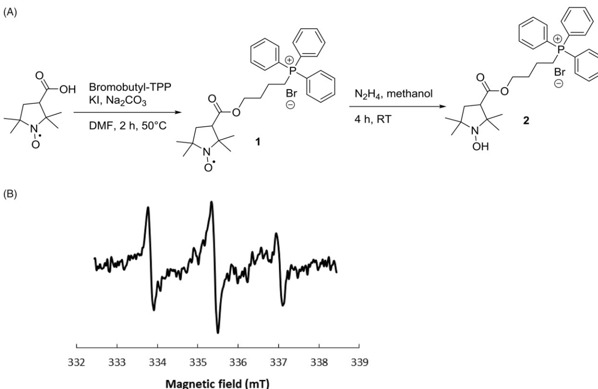
Figure 3. (A) Chemical synthesis of mitoCPH (2). (B) MitoCPH EPR signal recorded in the mitochondrial fraction of SiHa cells. This spectrum was recorded after incubation of SiHa cells in the presence of 160 \mu\text{M} of mitoCPH.
