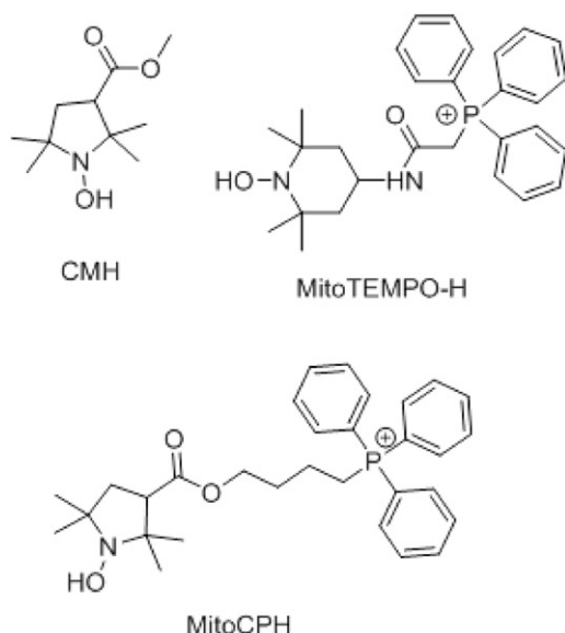
Figure 2. Chemical structures of cyclic hydroxylamines used for superoxide detection: CMH is a non-targeted agent; mitochondria-targeted compounds include the 6-membered ring mitoTEMPO-H, and the new 5-membered ring mitoCPH.
