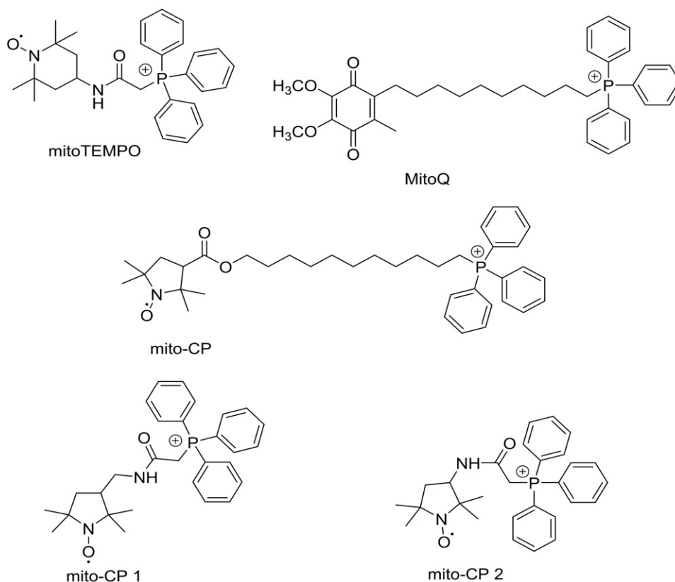
Figure 1. Examples of existing mitochondria-targeted antioxidants (MTA).
