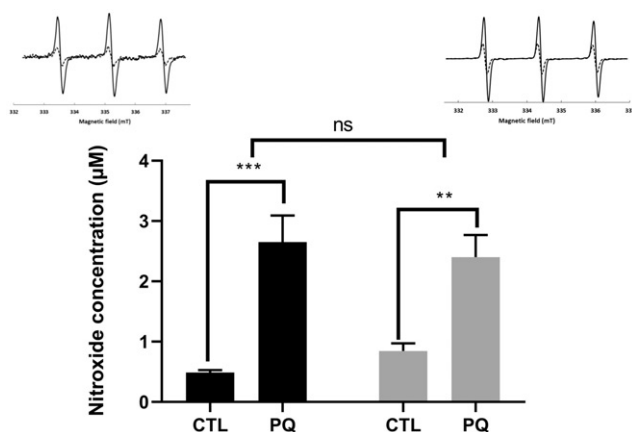
Figure 7. Detection of mitochondrial superoxide induced by paraquat (900 μM) during 10-min incubation at 310 K in EPR cavity in the presence of SiHa cells and mitoTEMPO-H (black) or mitoCPH (light grey). Data are expressed as the difference in EPR signal amplitude recorded at 10 min and the initial signal amplitude. Inserts: representative spectrum of mitoTEMPO-H (left) in unstimulated (dashed line) and stimulated cells (black line), and mitoCPH (right) in unstimulated (dashed line) and stimulated cells (black line). Experimental samples were obtained with 20 \times 10^6 cells/mL, DTPA 1 mM, PQ (900 μM) or PBS and the probe (50 μM). * p < .05 , *** p < .001 , ns p > 0.05 by two-way ANOVA with Turkey test.
