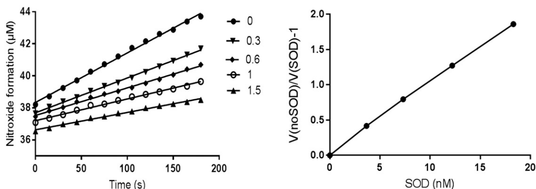
Figure 5. Determination of the bimolecular constant rate of mitoCPH oxidation by superoxide. On the left, evolution of the nitroxide concentration as a function of time upon superoxide generation in HX/XO system in the presence of different SOD concentrations. MitoCPH 1 mM; HX 1 mM; XO 3 mU/mL. On the right, dependence of relative efficiency of SOD-induced inhibition of nitroxide formation by superoxide on SOD concentration. Linear fit yields the bimolecular rate constant of mitoCPH oxidation by superoxide equal to 1.5 \times 10^4 \text{ M}^{-1} \text{ s}^{-1} .
