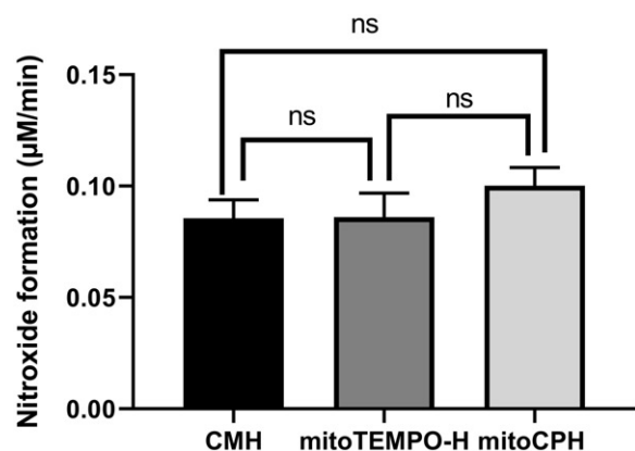
Figure 8. Nitroxides formation per minute at superoxide flux of 0.1 \mu\text{M}/\text{min} for each probe. Superoxide was generated using the XO/HX system in PBS and 1 mM DTPA was added. Concentration of the probes was 0.5 mM.
