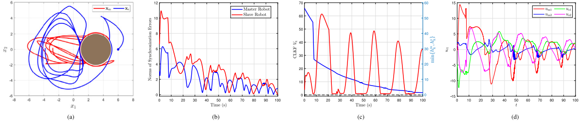
Fig. 3. Simulation of the master-slave synchronization problem under time-varying delays. (a) the state trajectories of the master and slave robots; (b) the norm evolution of the synchronization errors; (c) the evolution of the CLKF and CBKF; and (d) the control inputs for the master and slave robots.
