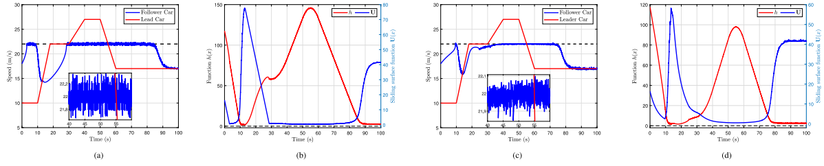
Fig. 1. Simulation of the CCC problem under two different controllers and \Delta = 0.2 . (a)–(b): the controller (50) with \mathbf{K}(\phi) = 5\text{sgn}(\mathbf{U}(\phi(0))) . (c)–(d): the controller (50) with \mathbf{K}(\phi) = 2.2\mathbf{U}(\phi(0)) - 2\|\mathbf{U}(\phi)\|^2/\mathbf{U}(\phi(0)) .
