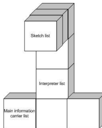
Figure 9. Three dimensional data structure which acts as an information carrier between the sketch interpretations
