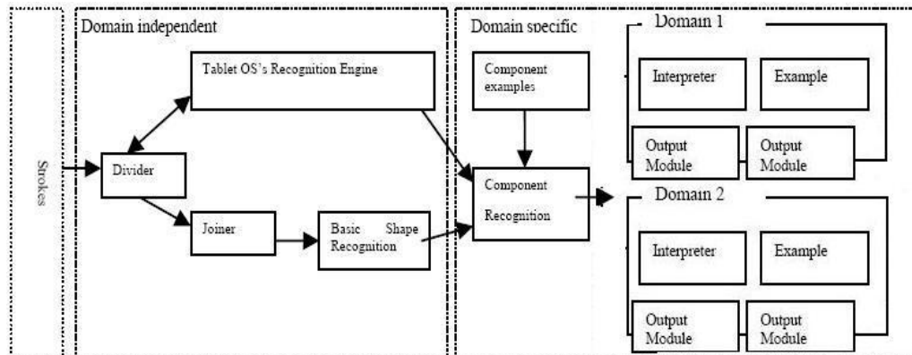
Figure 3. Architecture InkKit
