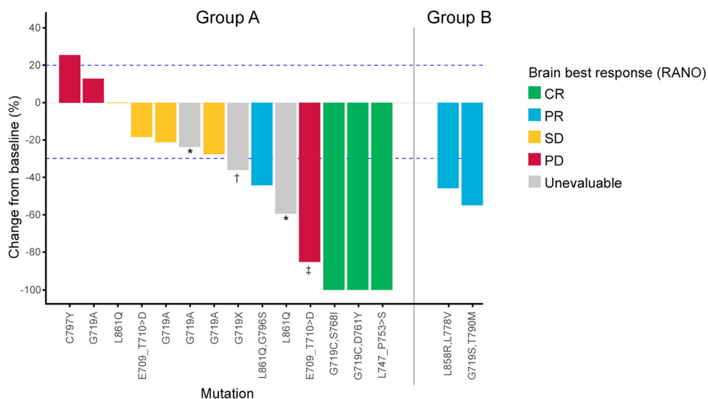
Figure 3. Waterfall plot revealing the maximal response in the size of measurable brain metastases. The corresponding EGFR mutations are depicted below. *Received radiotherapy to brain lesions; †missing data about clinical condition; ‡clinical deterioration. CR, complete response; PD, progressive disease; PR, partial response; SD, stable disease.
