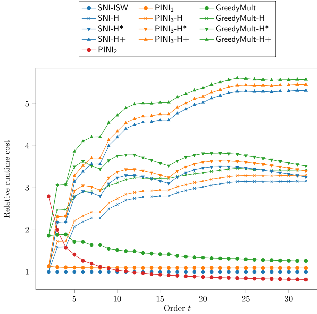
Figure 11: Runtime cost (relative to the SNI-ISW multiplication gadget) of different masked multiplication gadgets (with different noise rates).
