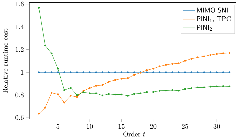
Figure 2: Software runtime cost for a bitslice, masked and composable AES S-box implementation. The cost is measured relatively to the cost of the optimized MIMO-SNI S-box in [CS18]. The curves for PINI 1 and TPC (S-box implementation with only ISW multiplications and no refresh elements, proven secure in [BGR18]) are indistinguishable at the scale of this plot. The source code for this plot is available from [Cas18b].
