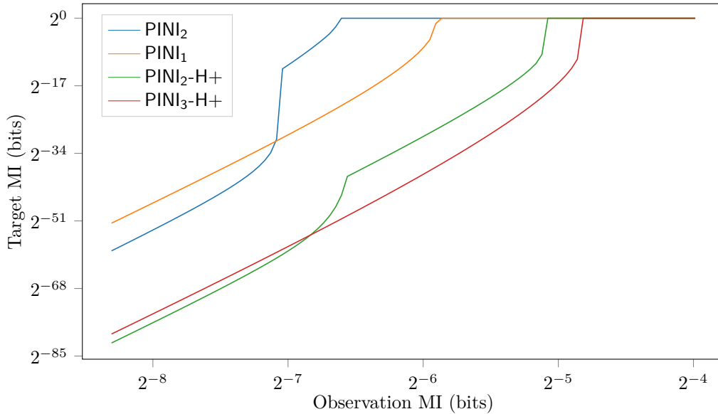
Figure 7: Target MI as a function of observation MI, for various PINI multiplication gadgets at order t = 15 .
