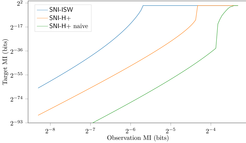
Figure 10: Target MI as a function of observation MI, for the SNI-H+ multiplication gadget at order t = 15 . For the SNI-H+ naive curve, the target MI is extracted through the sums of the input and output shares only (naive attack). For the SNI-H+ curve, the improved attack is considered (equations about sums of refresh input/outputs are added). The SNI-ISW curve (which is the same for both attacks) is shown as a reference point.
