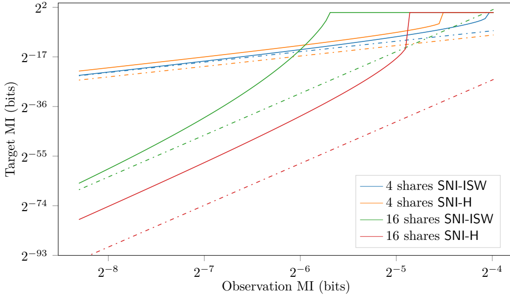
Figure 3: Target MI as a function of observation MI, for the SNI-ISW multiplication gadget [ISW03] and the SNI-H multiplication gadget [BCPZ16]. The continuous line is the bound on the target MI that can be extracted by the BP algorithm and the dashed line is a lower bound for the target MI computed assuming that only the leakages on input shares are exploited. The results for the NI multiplication gadget of Belaid et al. [BBP + 16] are identical to the SNI-ISW curves.
