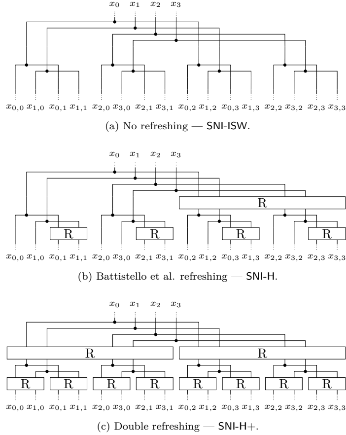
Figure 5: Exemplary instantiations of the generalized MatGen algorithm (Algorithm 2) for d = 4 . The algorithm basically corresponds to two trees of internal refresh gadgets (one for sharings of x , one for those of y ). The input shares are x_0, \dots, x_3 . The x_{i,j} are the outputs of the MatGen stage (see Equation (1)).
