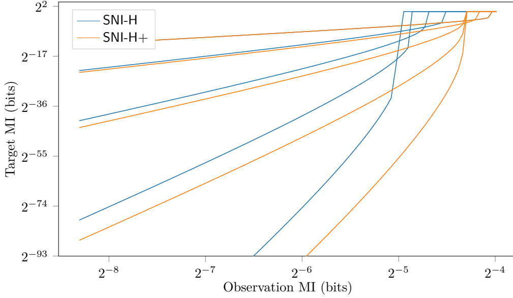
Figure 6: Target MI as a function of observation MI, for the SNI-H and SNI-H+ multiplication gadgets at orders t = 1, 3, 7, 15 and 31 .
