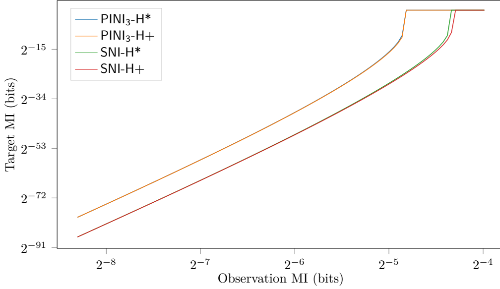
Figure 9: Target MI as a function of observation MI, for the SNI-H+, SNI-H*, PINI 3 -H+ and PINI 3 -H* multiplication gadgets at order t = 15 .
