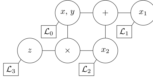
Figure 1: Factor graph with six nodes. \mathcal{L} labels indicate intrinsic information.
