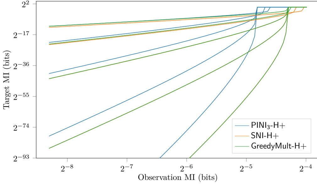
Figure 8: Target MI as a function of observation MI, for the SNI-H+, PINI 3 -H+ and GreedyMult-H+ multiplication gadgets at orders t = 1, 3, 7, 15, 31 . The curves for SNI-H+ and GreedyMult-H+ are superimposed for t \geq 7 .
