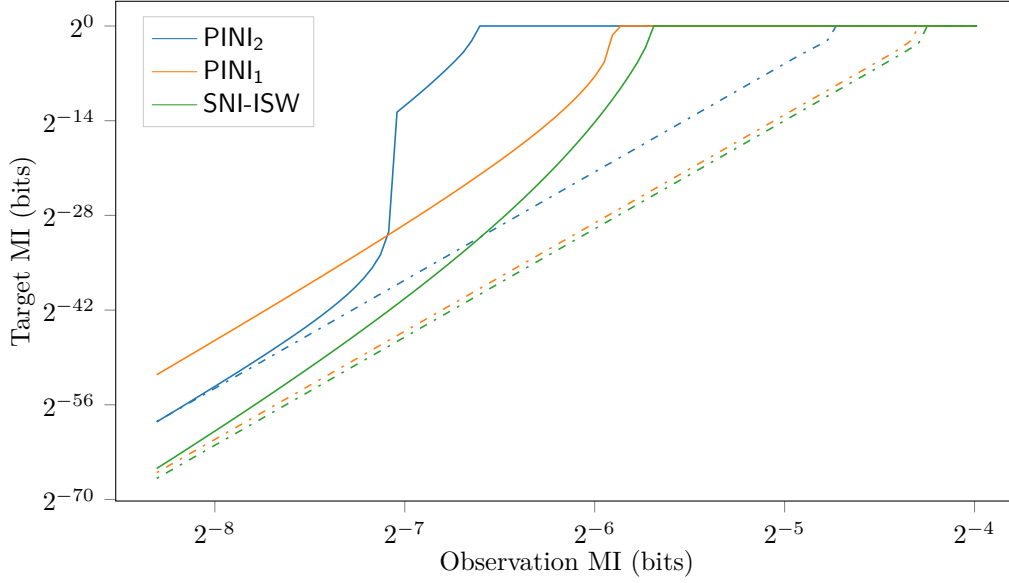
Figure 4: Target MI as a function of observation MI, for the SNI-ISW multiplication gadget [ISW03], the \text{PINI}_1 multiplication gadget [CS18] and the \text{PINI}_2 gadget (Section 3). The continuous line is the result of the belief propagation algorithm for the MI and the dashed line is a lower bound for the target MI computed assuming only the leakage on input shares are exploited. Results are shown for order 15.
