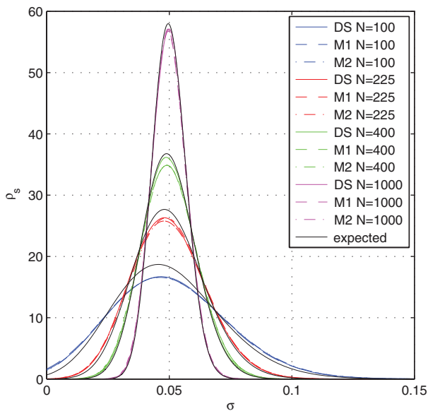
Figure 1. Stationary distributions of the process \sigma for \sigma_0 = 0.05 , \tau = 3 h and different values of N , as the result of the direct simulation of the lattice model DS (solid line) and of the iteration of the equivalent SDE with two different algorithms M1 and M2 (dashed and dot-dashed lines). All the runs are performed for a time period T = 3 years with time step \Delta t = 15 min, starting from the initial condition \sigma = \sigma_0 , so that no transient behaviour has to be taken into account. The distributions have been filtered with a window of length 1/N . The black solid lines represent the expected behaviour following the solutions of the corresponding Fokker–Planck equation.
