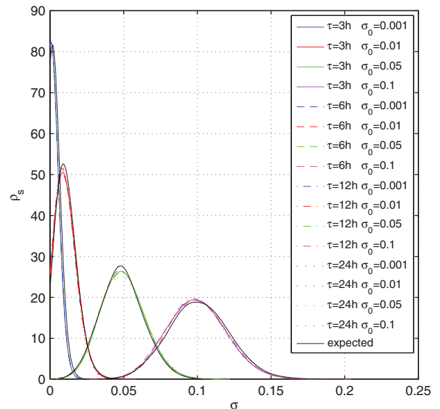
Figure 2. Stationary distributions of the process \sigma for N = 225 and different values of \sigma_0 and \tau , as the result of the direct simulation of the lattice model. All the runs are performed for a time period T = 3 years with time step \Delta t = 15 min, starting from the initial condition \sigma = \sigma_0 , so that no transient behaviour has to be taken into account. The distributions have been filtered with a window of length 1/N . The black solid lines represent the expected behaviour following the solutions of the corresponding Fokker–Planck equation.
