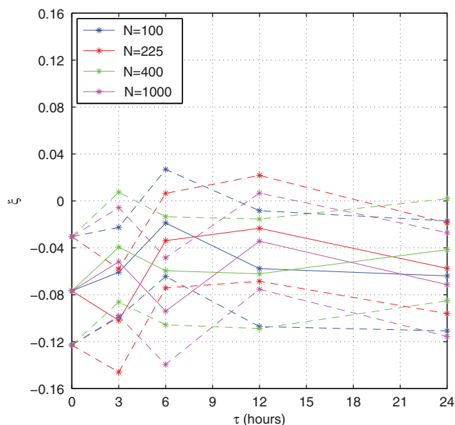
Figure 10. Shape parameter of the GEV distribution of maxima of daily convective precipitation at 1.4^\circ\text{N} versus values of \tau , for \sigma_0 = 0.05 and different values of N , for Aquaplanet experiments in the absence of a diurnal or seasonal cycle. The point at \tau = 0 represents the standard deterministic case with the BM scheme without shallow convection. The maxima have been selected following the block maxima approach, using the methodology explained in the text. The dashed lines represent the 95% confidence interval of the estimate of the GEV parameters obtained with the maximum-likelihood method.
