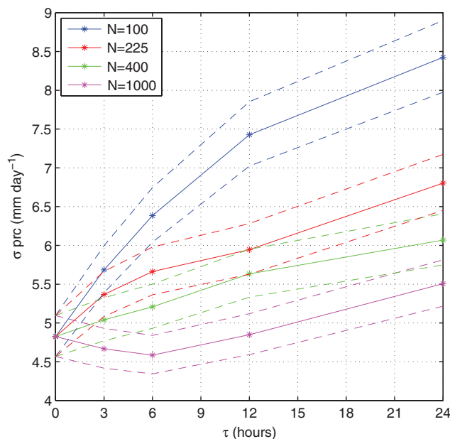
Figure 9. Scale parameter of the GEV distribution of maxima of daily convective precipitation at 1.4^\circ\text{N} versus values of \tau , for \sigma_0 = 0.05 and different values of N , for Aquaplanet experiments in the absence of a diurnal or seasonal cycle. The point at \tau = 0 represents the standard deterministic case with the BM scheme without shallow convection. The maxima have been selected following the block maxima approach, using the methodology explained in the text. The dashed lines represent the 95% confidence interval of the estimate of the GEV parameters obtained with the maximum-likelihood method.
